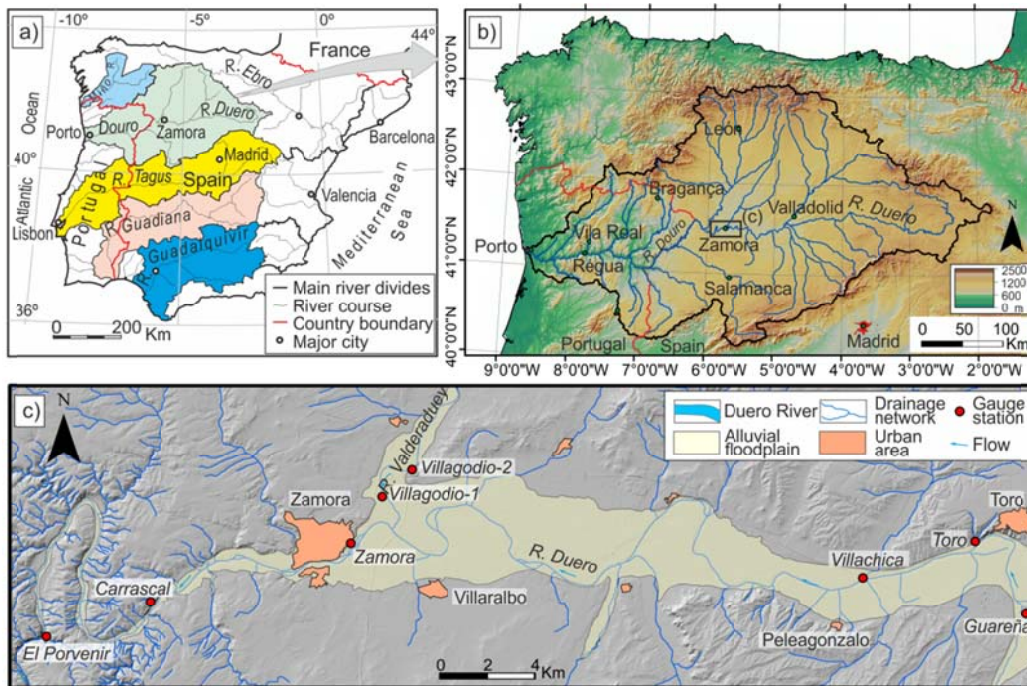
Figure 1: a) The Duero River Basin (green) in the Iberian Peninsula together with Miño (light blue), Tagus (yellow), Guadiana (orange) and Guadalquivir (dark blue) catchments draining towards the Atlantic Ocean; b) Relief map of NW Iberia with the Duero catchment boundary, main drainage network and major cities. The rectangle at Zamora shows the location of (c); c) Hillshade map with extension of the floodplain between Toro and Zamora. Map shows location of gauge stations in the Duero and Valderaduey rivers.
