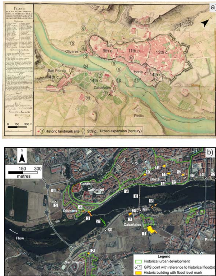
Figure 2: Historic flood landmarks and GPS point locations. a) Historic map of Zamora (1:2900 in scale) published on March 11, 1766 by Juan Martín Cermeño. Old graphic scale of 200 toess (1toe = 13.5 cm) Black polygons illustrate the timing of urban development through time in the old city (9-13th centuries) and suburbs (14th century and beyond). The city of Zamora was rounded by walls that in the old city had defence purposes and in the suburbs protected against flooding; b) Orthophoto of Zamora (year 2017) showing same urban expansion areas as a). Legend: 1) Las Dueñas convent; 2) San Frontis church; 3) Olivares mills; 4) San Claudio de Olivares church; 5) Campo de la Verdad (likely location of old Santa Clara convent); 6) Santiago de los Caballeros church; 7) Old San Francisco convent; 8) Stone bridge; 9) Gate of Pescado dated at 14th century (a new one was built in 1849; Fig. 4b); 10) Santa Lucia church; 11) Santa Maria de la Horta; 12) Santo Tomás church; 13) San Leonardo; 14) Cavalry headquarters; 15) Mengue Avenue; 16) Iron bridge; 17) Railway bridge; 18) Cabañales mills; 19) San Jerónimo; 20) Survey monument N.P. 1482 (IGN 1925); 21) IGN Survey mark 305004; 22) IGN Survey mark 305005; 23) IGN Survey mark 305003. Source: a) Biblioteca virtual Ministerio de Defensa https://bibliotecavirtual.defensa.gob.es/ ; b) National Geographical Institute.
