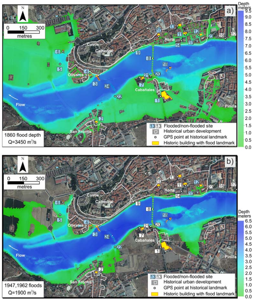
415 Figure 5: Bi-dimensional hydraulic model results. a) Flood extension and depth for 3450 m 3 /s estimated for the 1860 flood and flood landmarks and descriptions of flooded sites (number in blue square). b) Flood extension and depth for a discharge of 1900 m 3 /s. Legend with names of flood landmarks and flooded sites in Fig. 2. Elevation (meters above sea level) reached by 1860-flood in Table S1. Aerial Orthophoto from the Spanish National Geographic Institute, IGN; https://www.ign.es .
