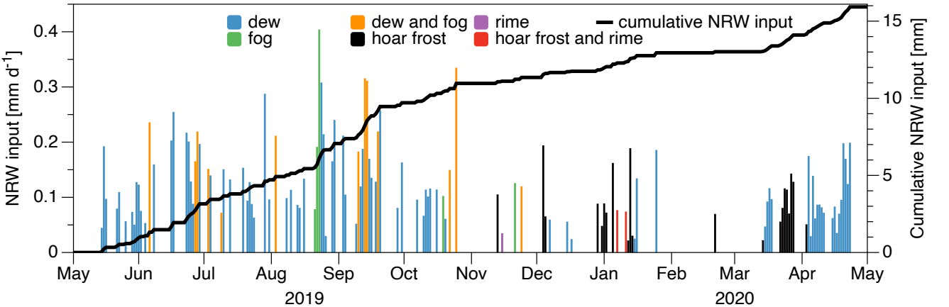
Fig. 8. Daily NRW inputs at CH-FRU over one year, starting on 2nd May 2019 till 2nd May 2020. The blue bars indicate NRW events with their corresponding NRW input per day. Different colours indicate different types of NRW inputs. The black line indicates the cumulative NRW input over one year. The annual total NRW input was 15.9 mm, about 1% of total precipitation during this time.
