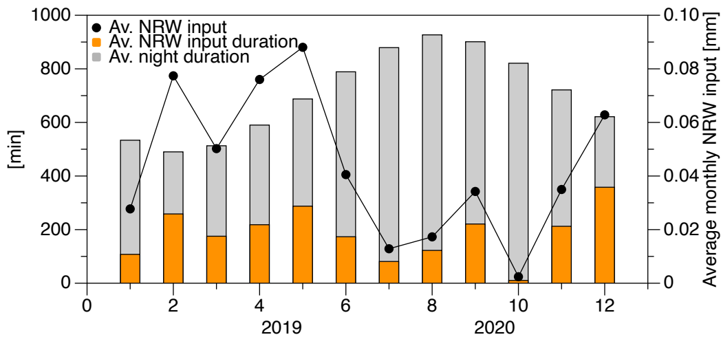
Fig. G1. Average monthly NRW input with average monthly NRW input duration and average night duration (potential NRW input duration).
