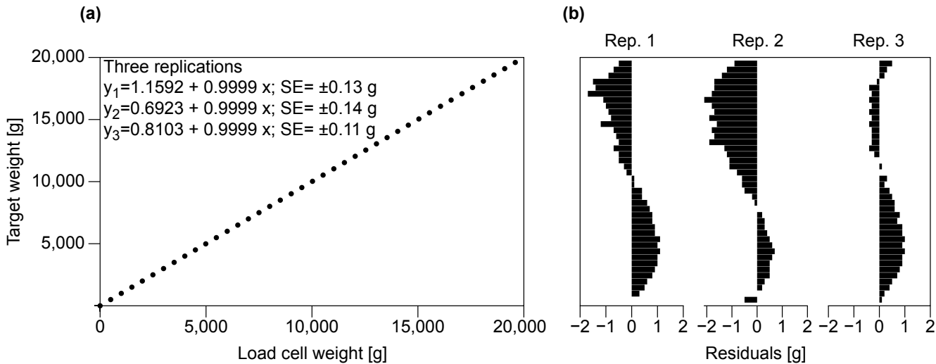
Fig. 2 (a) Absolute calibration of a load cell placed in a weighing platform. Three replications (overlapping data points) are shown with SE of the intercept. (b) The residuals from the target mass of three replications (Rep. 1 to 3) were in the range of \pm 2 g.
