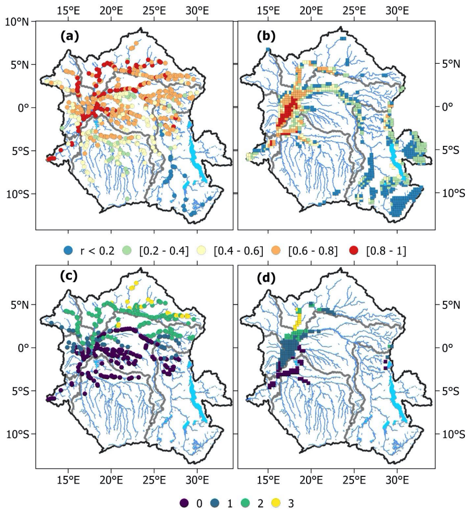
1420 Figure 11. Maps of the optimal coefficient correlation and associated lag at each VS and GIEMS-2 cells. (a) Optimum coefficient correlation between altimetry-derived SWH (from ERS2, ENV, SRL, J2/3 and S3A missions) at each VS against in situ water stage at the Brazzaville/Kinshasa station. (b) Same as (a) for each GIEMS-2 cell against the river discharge at Brazzaville/Kinshasa station. (c) and (d) show, respectively, their optimum lag in months. In (c) and (d), only the time lags for which the maximum correlation has p-value <0.05 are displayed.
