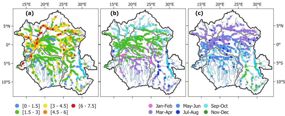
1340 Figure 5 Statistics for radar altimetry VSs. (a) displays the maximum amplitude of SWH (in m), (b) presents the 1345 average month of the maximum of SWH, and (c) shows the average month of the minimum of SWH.
