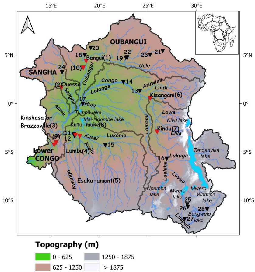
1285 Figure 1 Congo River Basin (CRB): its topography from Multi-Error-Removed Improved -Terrain (MERIT) digital elevation model, major sub-basins (in brown line), major rivers and tributaries. Also displayed are the locations of in situ gauging stations (triangle). Red and black triangles represent respectively the gauge stations with current (>1994) and historical observations. Their characteristics are reported in Table 1.
