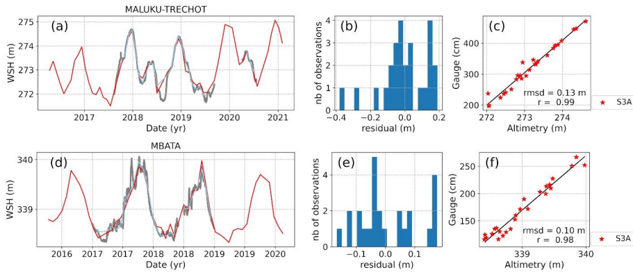
1330 Figure 4 Similar to Fig. 3 but the in situ stations are located right below the satellite track of S3A. Comparison of in 1335 in situ water stage (Table 1) and S3A altimeter-derived SWH at different sites (Fig. 1 for their locations). The left panel presents the time series of both in situ and altimetry-derived water height where the grey line in the background shows the in situ daily WS variations (grey), the sky-blue line indicates the in situ WS sampled at the same date as the altimetry-derived SWH from S3A (red) mission. The middle panel shows the histogram of the difference between the altimetry-derived SWH and the in situ WS. The right panel portrays the scatterplot between altimetry-derived SWH and in situ WS. The linear correlation coefficient r and the Root-Mean-Square Deviation (RMSD) considering all the observations are indicated. The solid line shows the linear regression between both variables.
