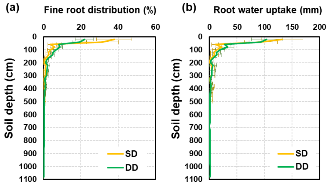
Figure 11: Profile of (a) fine root density distributions (%) and (b) root water uptake distributions (mm) resulting from different approaches (SD and DD approach). The error bars represent the standard error (STD) of the mean of different years.
