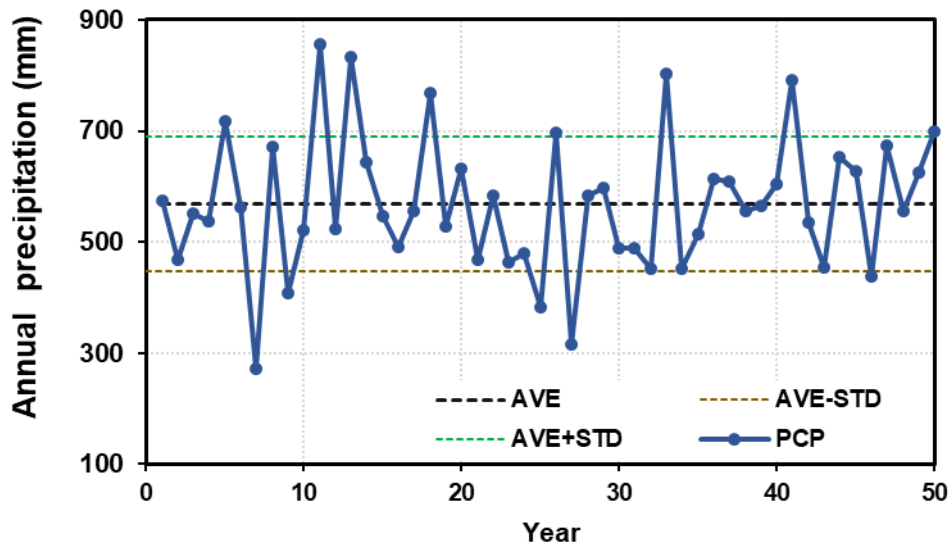
260 Figure 4: Time series of annual precipitation (mm). Dashed coloured lines represent the average values (AVE) and plus or minus one standard deviation (STD).
