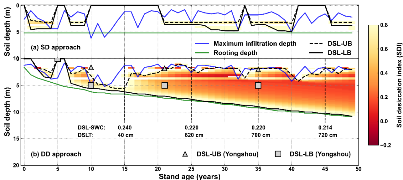
495 Figure 12: Evolution of the drying soil layers with stand age simulated by (a) the static rooting depth (SD) and (b) the dynamic rooting depth (DD) approaches over a 50-year period at Yongshou, Loess Plateau. The triangles and squares are the observed upper and lower boundaries, respectively, adopted from Jia et al. (2017a). Notes: DSL-UB: the upper boundary of drying soil layer; DSL-LB: the lower boundary of drying soil layer; DSL-SWC: mean soil water content within the drying soil layer; DSLT: the thickness of the drying soil layer.
