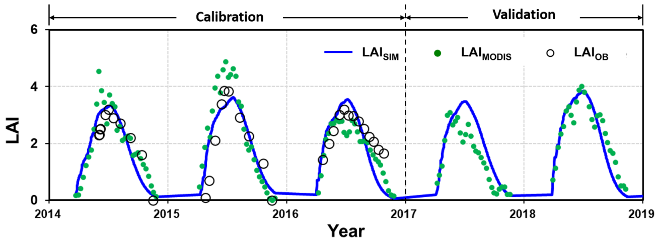
Figure 5: Comparison of leaf area index (LAI) from simulation ( LAI_{SIM} ), MODIS-derived data ( LAI_{MODIS} ), and plot observation ( LAI_{OB} ) for the calibration (2014–2016) and validation (2017–2018) periods.
