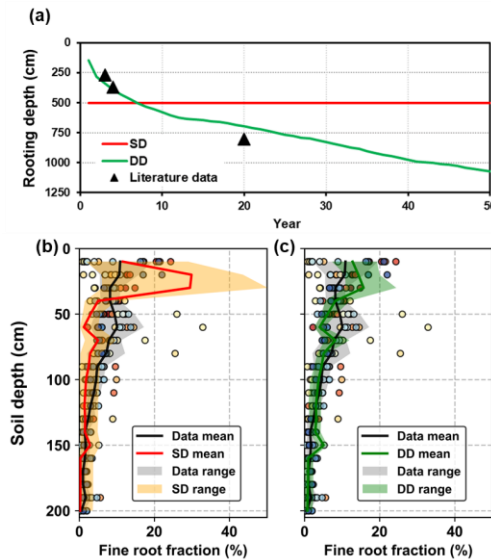
Figure 8: Evaluation of the simulated root distribution against the literature data. (a) Rooting depth, (b) fine root distribution in top 2.0 m soil layer for the static rooting depth approach (SD), (c) fine root distribution in top 2.0 m soil layer for the dynamic rooting depth approach (DD). The scatters with different colours illustrate the observational data from different literature, and the shaded areas illustrate the range of mean \pm standard deviation of simulation.
