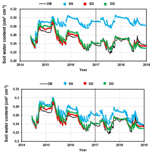
Figure 6: Comparison of the 5 m profile averaged soil water content (SWC) from observation (OB) and three root simulation approaches during the calibration (2014–2016) and validation (2017–2018) period. Notes: SS, Static rooting depth and Static fine root distribution; SD, Static rooting depth and Dynamic fine root distribution; DD, Dynamic rooting depth and Dynamic distribution of fine roots.
