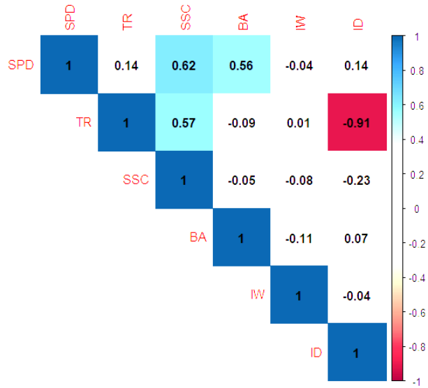
320 Table 43: Pearson correlation coefficients between sediment deposition per day (SPD), tidal range (TR), suspended sediment concentration (SSC), beel surface area (BA), width of the inlet (IW) and inundation depth (ID).
