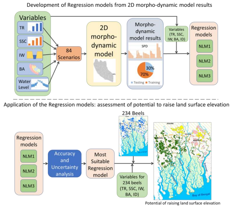
Figure 2: General approach used to establish the regression models for sediment deposition from physical control variables/parameters, and their subsequent application to estimate potential of raising land surface elevation throughout the southwestern Bangladesh delta.
