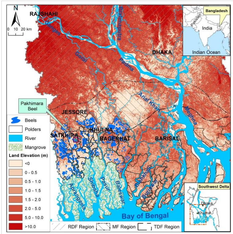
Figure 1: Polders and beels of southwestern Bangladesh. Elevation data from Coastal Dem DEM (Kulp and Strauss, 2018). Beel data from Adnan et al., 2020.
