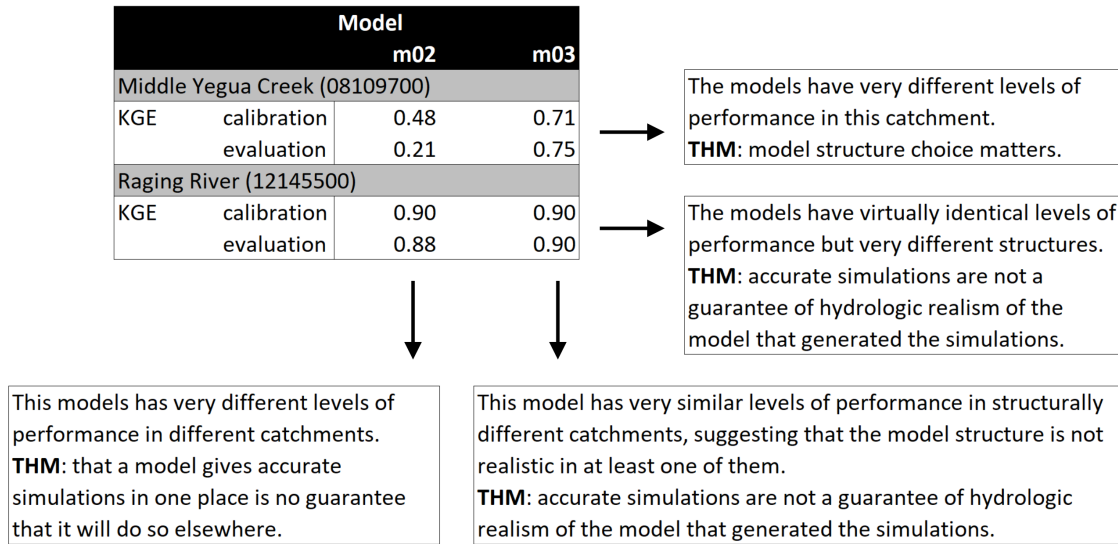
Figure 1. Using comparative assessments The table shows which calibration and evaluation Kling-Gupta Efficiency (KGE) scores the students will find when calibrating a single optimal parameter set for each combination of model and catchment, using their own adaptation of existing calibration code included in the MARRMoT repository. The calibration period is set as 1989-01-01 to transfer lessons 1998-12-31; evaluation data cover the period 1999-01-01 to 2009-12-31. Comparative assessments of these KGE scores transfers certain Take Home Messages (THM) about hydrologic model structure uncertainty, as detailed in the four text boxes.
