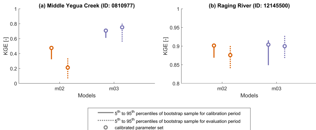
Figure 4. Sampling uncertainty in KGE calculation, quantified as the 5 th to 95 th percentile of the Bootstrap samples performed by the gumboot package. Note the different scales on the y-axes.
