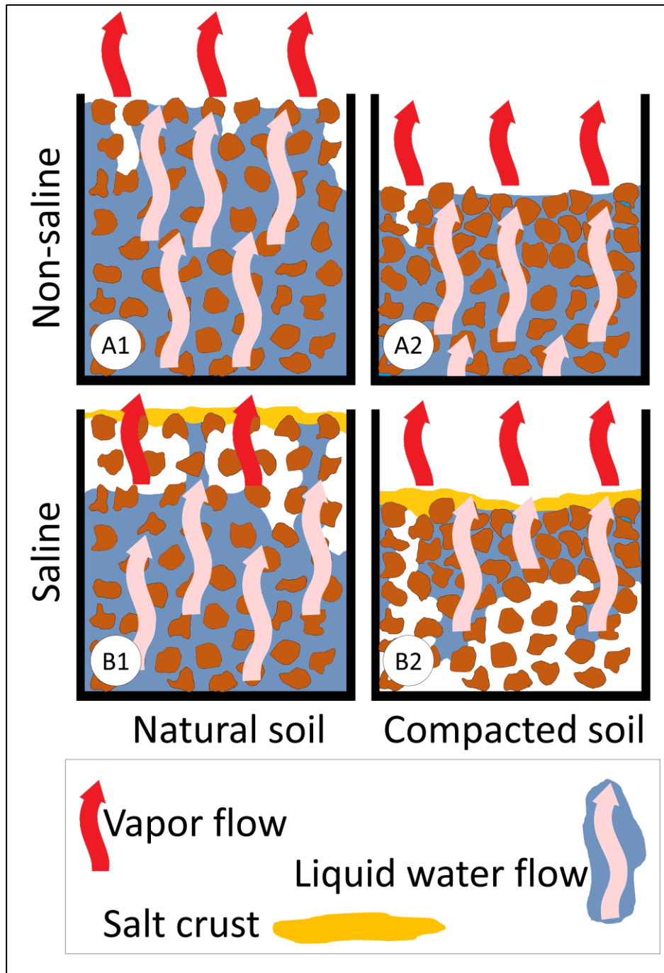
Figure 1: Conceptual model of evaporation and salt precipitation under compacted and non-compacted conditions; (A) initial stages of evaporation with the first air entry into the matrix. (B) advanced stages of evaporation, with the receding drying front and the hydraulic discontinuity between the soil and the salt crust (yellow layer), for the non-compacted soil, and the hydraulic continuity between the salt crust and the underlying soil, for the compacted state.
