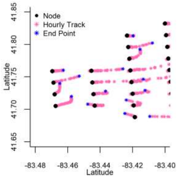
445 Figure B1. Surface current data was available hourly within western Lake Erie. These 24-hour data were used to track the daily movement of water from each node.
