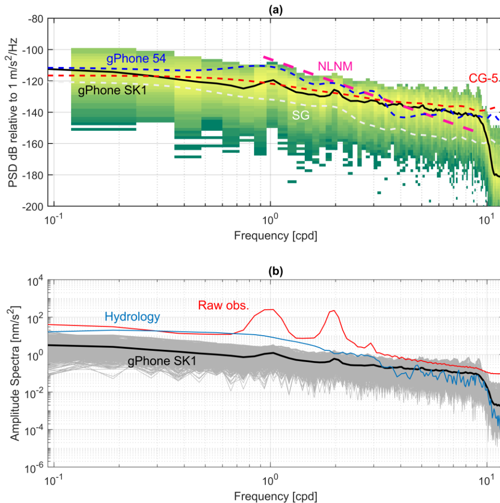
Figure 3 Power Spectral Density (PSD) of the Škocjan gravity residuals. Frequency is expressed in cycles per day (cpd). Coloured patches: histogram showing the distribution of the PSDs; color code proportional to the number of PSD values for given intervals of frequency and dB. Black solid line: median PSD. For comparison median PSD of gravimeters installed in a Strasbourg station ((Riccardi et al., 2011)): blue dashed line: gPhone #54 ; red dashed line: PSD of the Scintrex CG5; white dashed line: PSD of the Superconducting gravimeter SG-C026. Purple thick dashed line: New Low Noise Model according to (Petersen, 1993). b) Amplitude spectrum of the Škocjan gravity residuals. Grey lines: individual spectral estimates. Black Solid line: median value. Blue curve: amplitude spectrum of the flood event in February 2019; red line: average amplitude spectrum for observations including tidal contribution and atmospheric effects.
