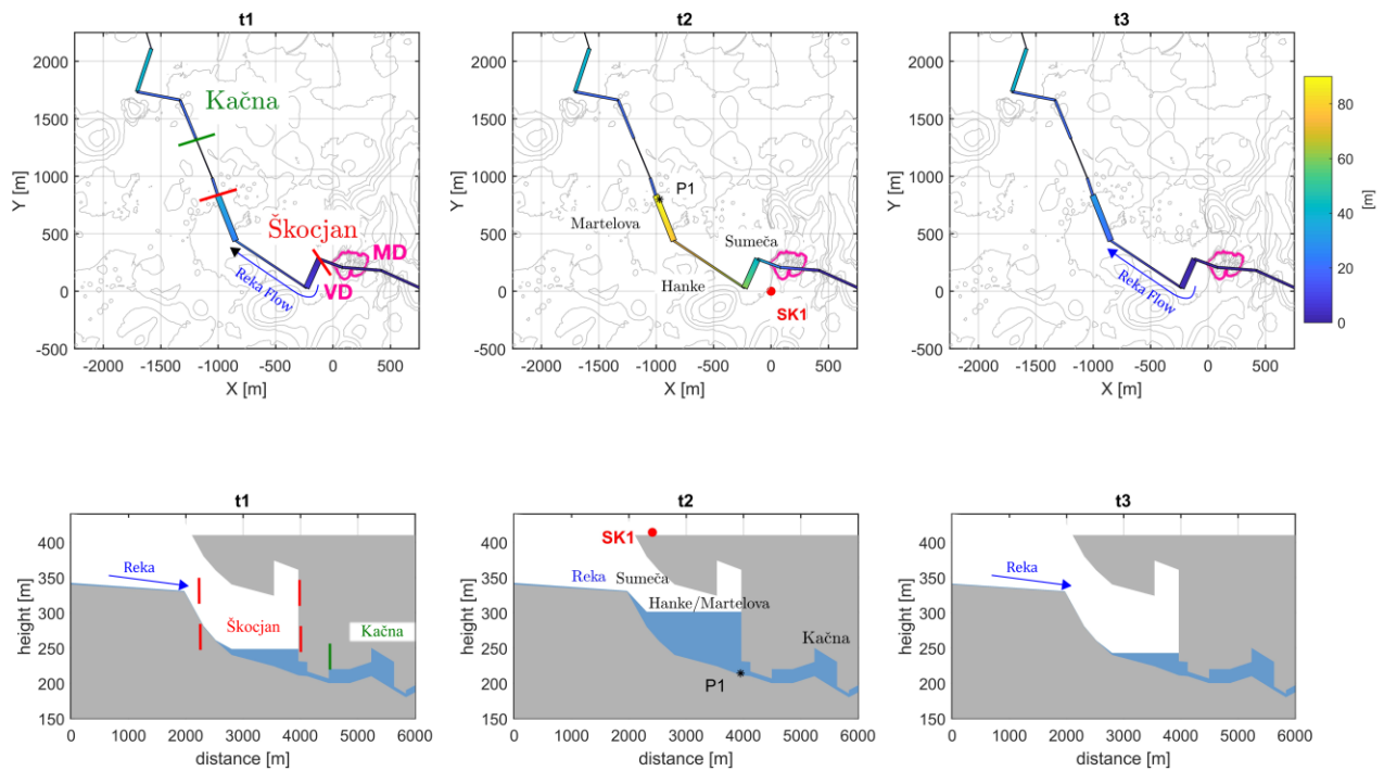
Figure 4 Water distribution in the caves at three snapshots t_1 , t_2 , t_3 (refer to Figure 2b): for each time-step, a cross section and a plan view of the water levels in the caves are displayed. Note that in the cross sections the vertical scale is exaggerated by a factor of about 10 and that the cross sections are plotted from east to west. The colour code is
