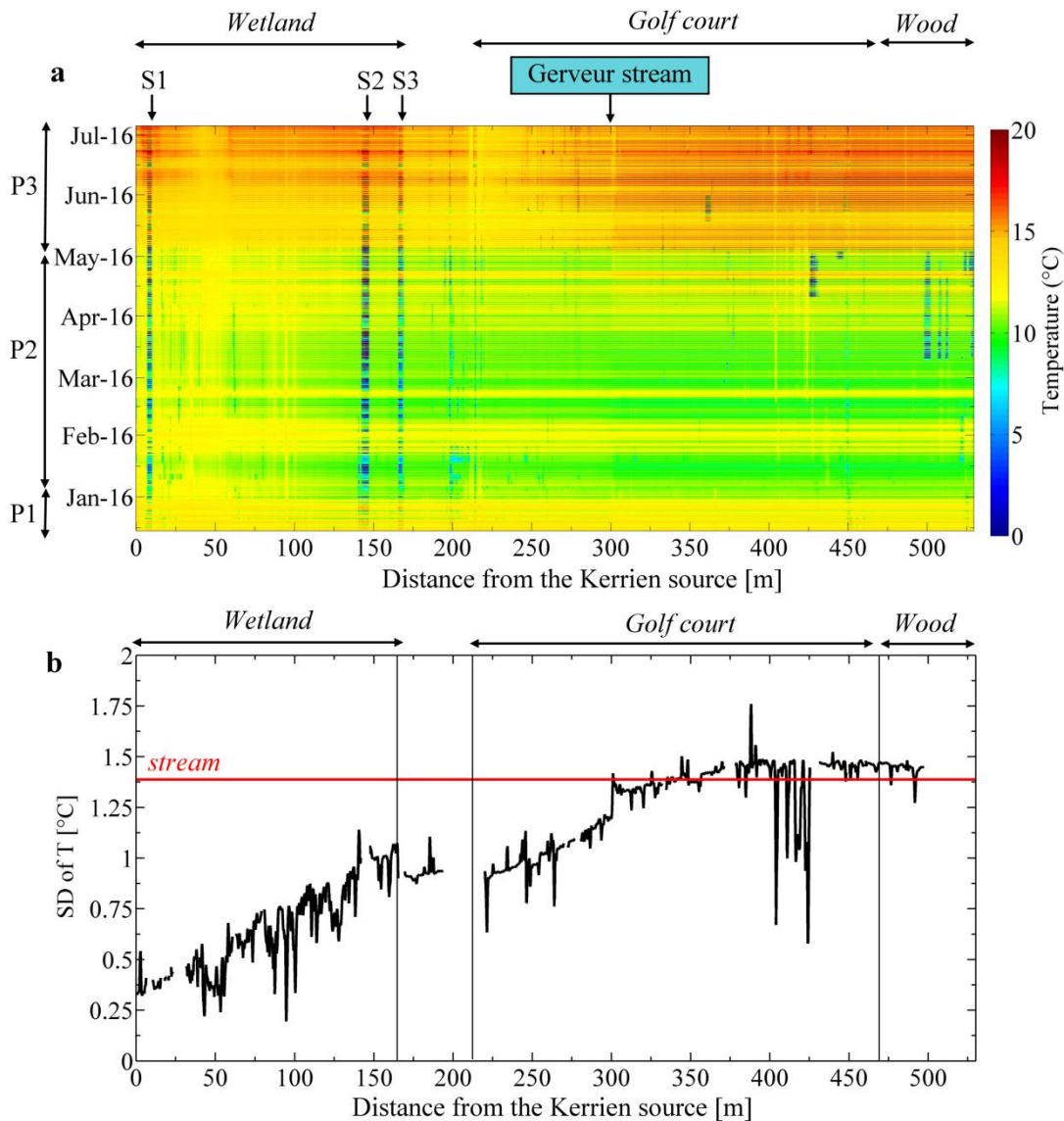
295 Figure 4: a. Long-term monitoring of streambed temperature along the river using DTS. Sections S1, S2 and S3 match with spots where the cable lies on the bank because of obstacles in the stream (gauging stations). Temporary thermal anomalies located for instance in 425 m and around 500 m correspond to air-exposed periods during which the cable was not held at the sediment/water interface. b. Standard Deviation (SD) of the temperature calculated over the experiment duration for each measurement point along the FO cable. Sections where the cable was outside the stream or punctually unburied were removed. The red line represents the SD of the stream temperature (1.38°C) measured at the gauging station E30.
