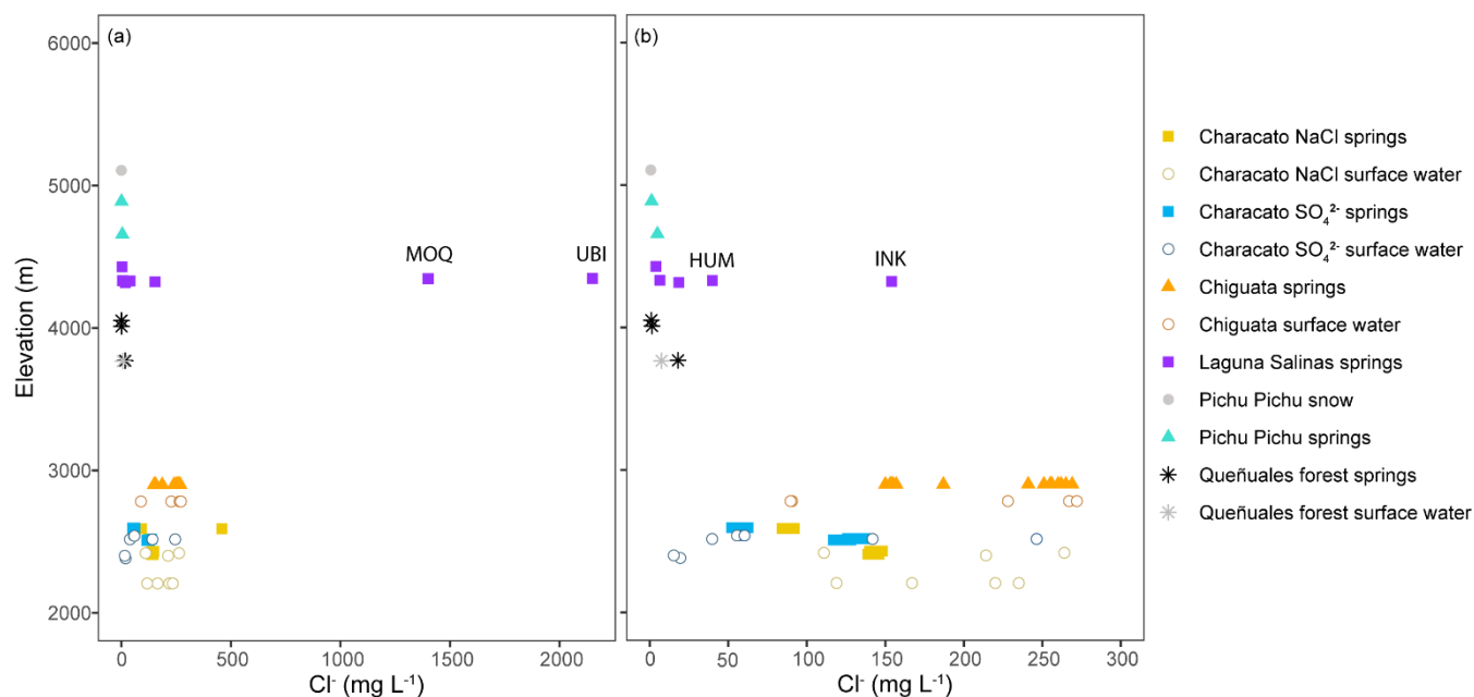
415 Figure 7. a) Chloride concentration of all water samples at different elevations, excluding Laguna Salinas surface water, and b) excluding two Laguna Salinas springs (UBI and MOQ) with high \text{Cl}^- .
