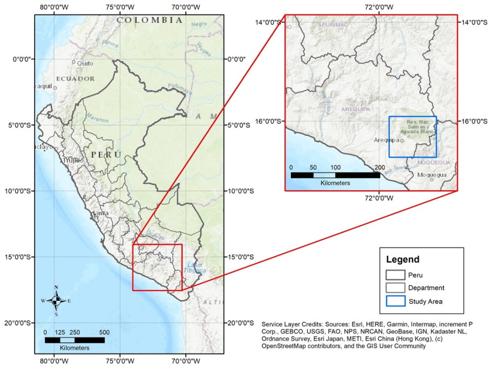
Figure 1: Map of the Arequipa department in southern Peru, the Quilca-Vitor-Chili rivers basin, and our study area in the northeastern part of this basin.
