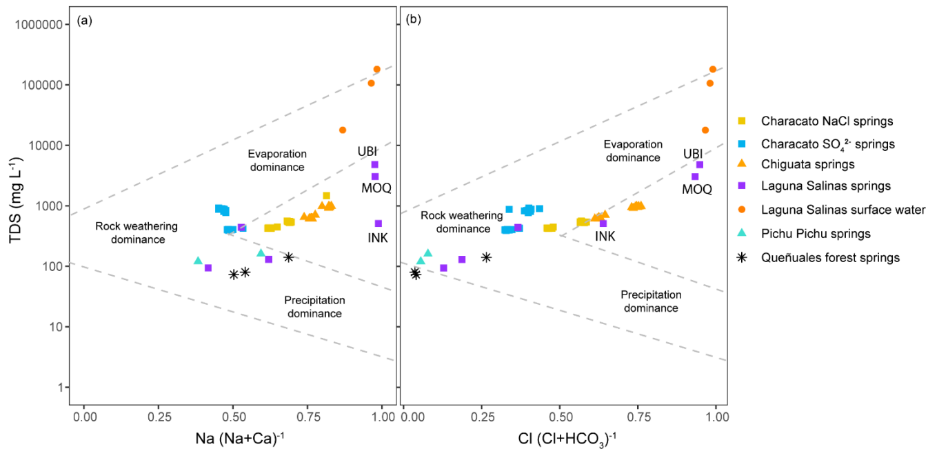
400 Figure 6. Gibbs a) cation and b) anion diagram for the ratios of major ion compositions calculated using ppm units. Springs in our study area show a distribution of evaporation, rock weathering, and precipitation influence on the groundwater chemistry. Select springs discussed in the text are labelled with their sample ID.
