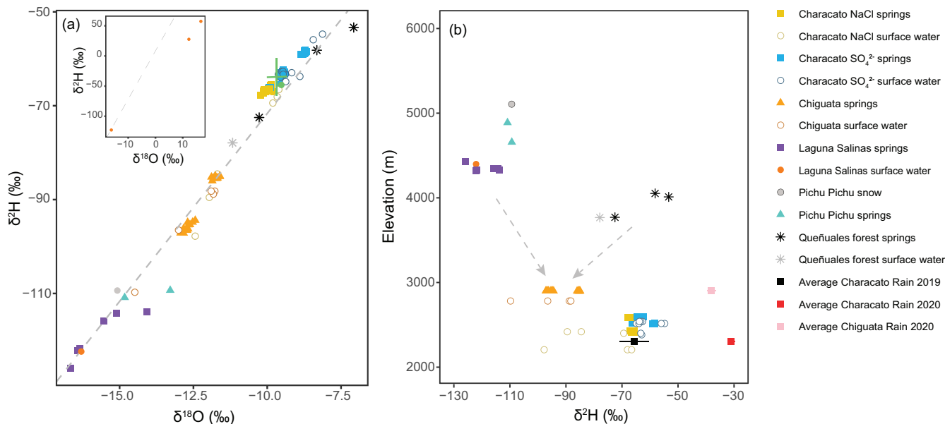
335 Figure 3: a) Isotopic composition of springs, rivers, and precipitation sampled in our study area. The LMWL (dashed grey line) estimated for this region was \delta^2\text{H} = 8.0 \delta^{18}\text{O} + 10.9 ‰. The inset is an adjusted scale to show isotopically enriched dry-season Laguna Salinas surface water (LSA: \delta^{18}\text{O} = 12.3 , \delta^2\text{H} = 28 and MAX: \delta^{18}\text{O} = 16.7 , \delta^2\text{H} = 57 ) and 2020 amount weighted average rain values. b) Deuterium composition with respect to elevation of springs, rivers, Laguna Salinas wet-season surface water, and precipitation. The isotopic composition of dry-season Laguna Salinas surface water has been omitted. Amount weighted average of rain are shown with amount weighted standard deviation error bars and do not show the full range of daily maximum and minimum values. Surface waters in open symbols with the exception of Lagunas Salinas surface waters which are closed for emphasis. Arrows indicate hypothesized mixing lines between high-elevation sources of recharge. Sample classification (NaCl and \text{SO}_4^{2-} ) based on 340 chemistry data presented in section 4.2.
