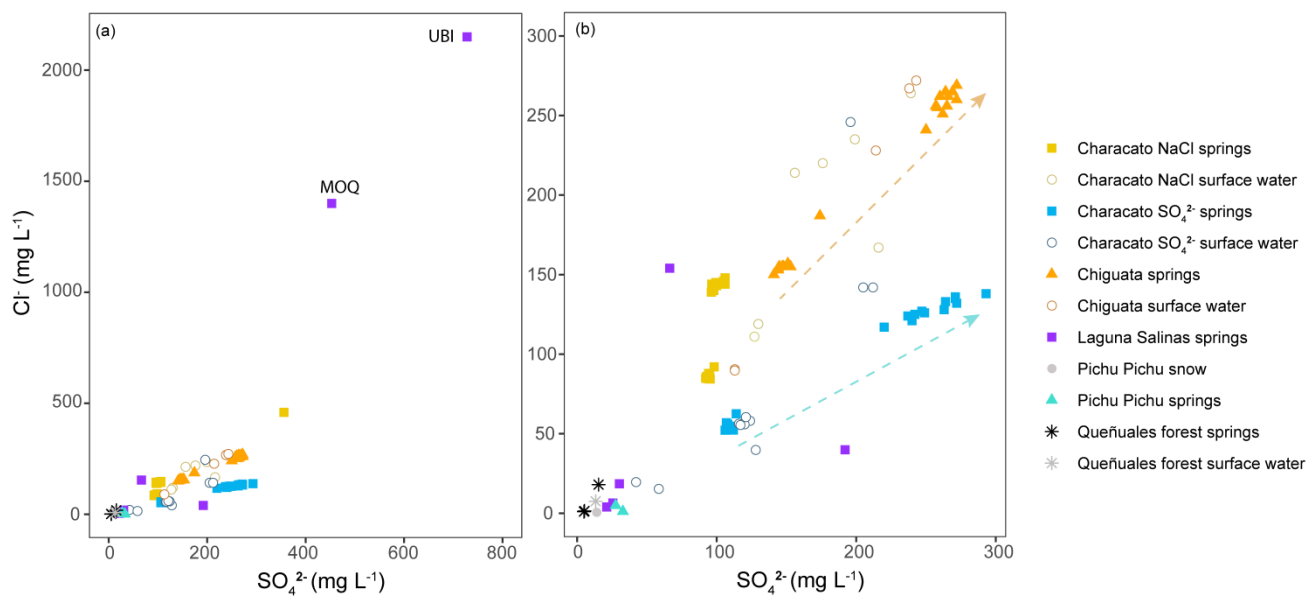
430 Figure 8. Relationships between \text{Cl}^- and \text{SO}_4^{2-} of a) all water samples, except Laguna Salinas surface water, and b) excluding two Laguna Salinas springs (UBI and MOQ) with high \text{Cl}^- . Dashed lines indicate patterns of chemical evolution or mixing and not statistical trend lines. The orange evolution line connects springs along the Río Andamayo fault system and the blue line connects springs in the Characato district furthest from the Río Andamayo in a separate cluster of shorter faults.
