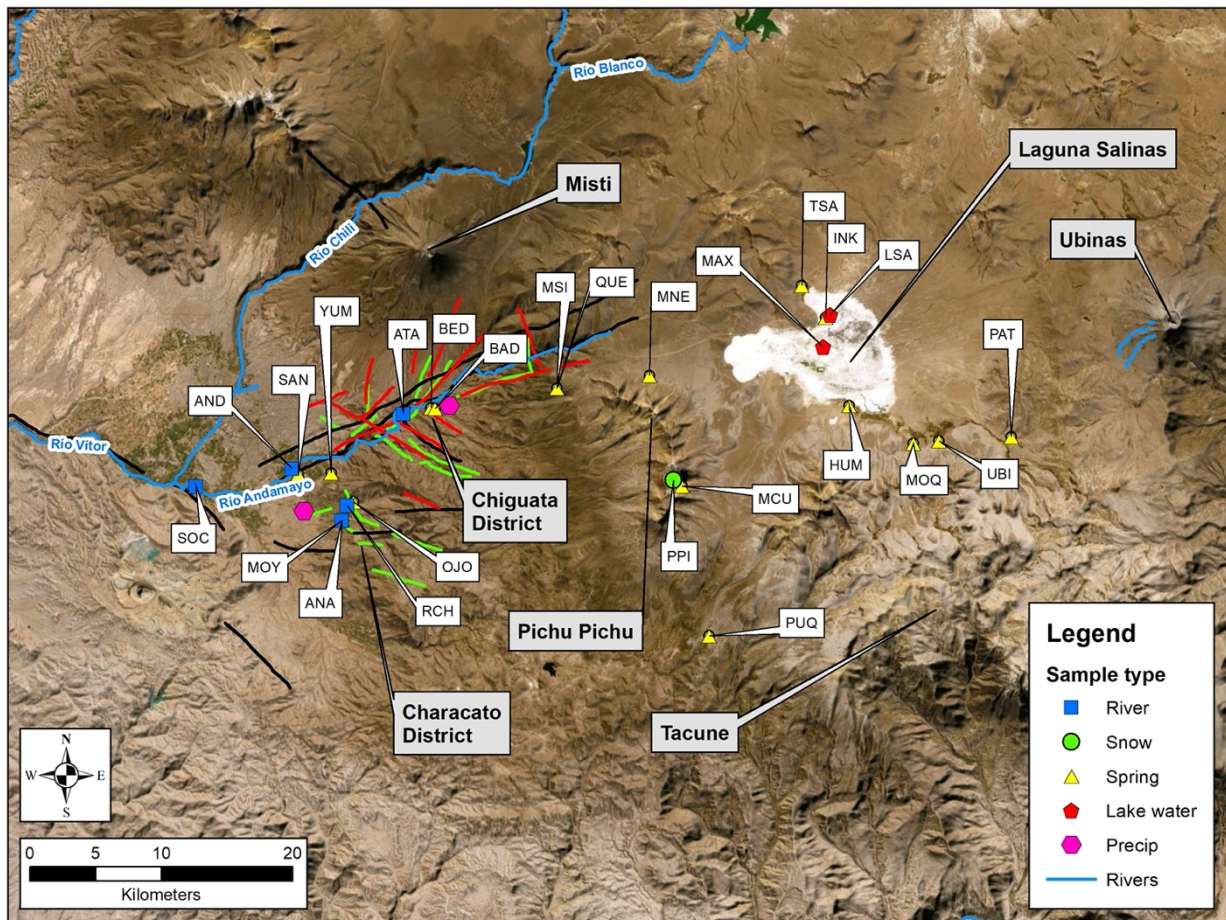
170 Figure 2: Map of the study area, sampling locations, and faults identified. The different types of water are indicated by different symbols in the legend. Green lines are faults identified in Bernard et al., 2019; black lines are faults identified in Lebti et al., 2006; and red lines are faults identified in Thouret et al., 2001. The Río Andamayo is fault-bounded (black lines running parallel to the river). The La Bedoya (BED) and El Badén (BAD) springs are located in the Chiguata District. The springs Sabandia (SAN), Yumina (YUM), Ojo de Characato (OJO), and Santa Ana (ANA) are located in the Characato district. Blue lines are rivers. (credit: Emily E. Frisbee).
