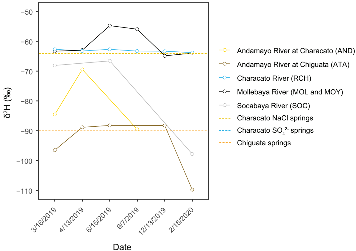
Figure 4: Deuterium composition time series of rivers in the Characato and Chiguata districts show isotopic compositions similar to nearby springs indicating strong groundwater influence on surface waters. MOL and MOY refer to Mollebaya river during the wet and dry seasons, respectively. Dashed lines indicate average deuterium compositions of low-elevation springs during the same sampling period. Characato NaCl springs minimum and maximum = -67.8‰ and -65.6‰; Characato sulfate springs minimum and maximum = -66.4‰ and -58.2‰; and Chiguata springs minimum and maximum = -97.2‰ and -85‰.
