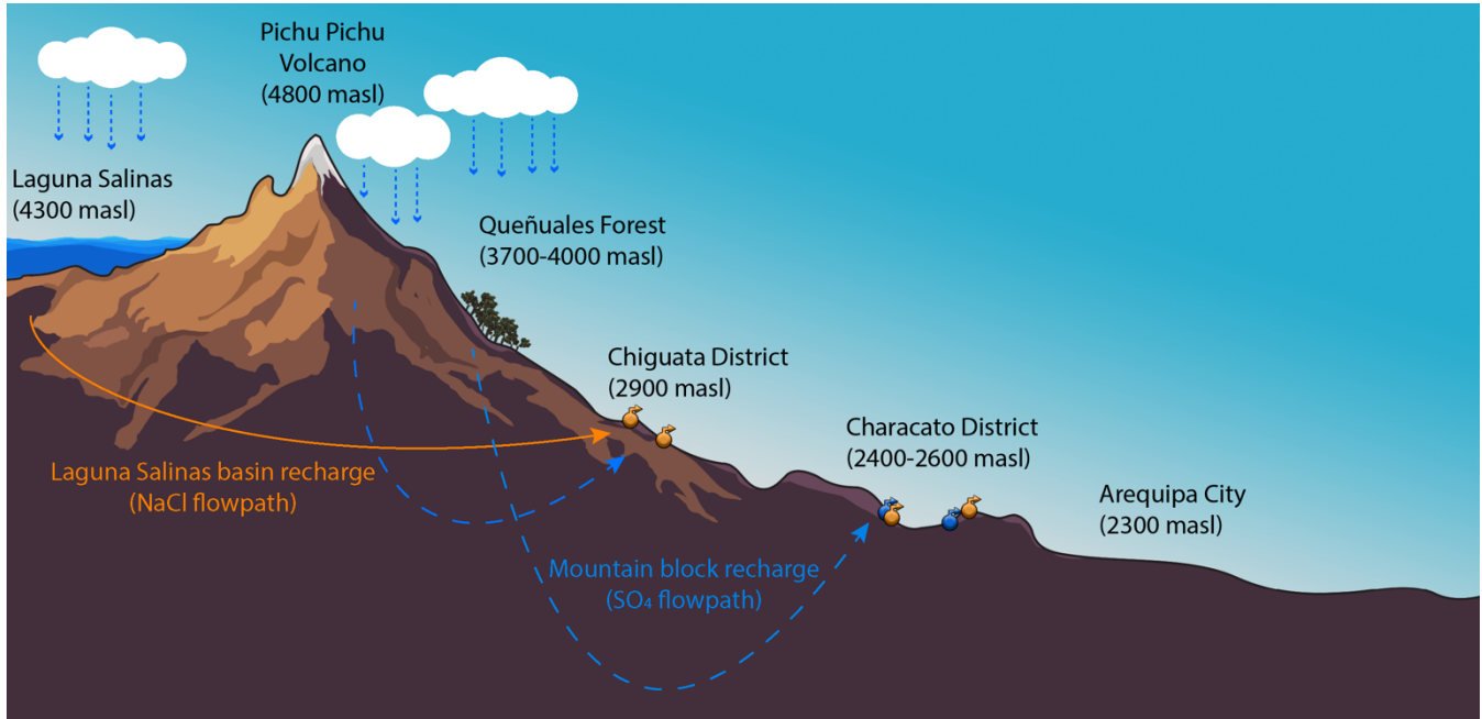
Figure 9. Cross section of our study area in the Quilca-Vitor-Chili basin, east of the city of Arequipa. Conceptual model identifying zones of recharge and flowpaths in Characato (Mountain block recharge (MBR) only) and Chiguata (salar basin recharge and MBR). Note, the conceptual groundwater flowpaths do not cross. (credit: Diego Alvarez)
