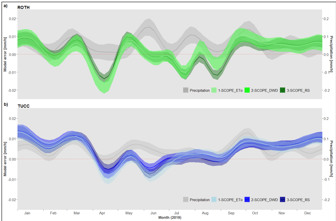
Figure 5. Smoothed time series of the volume (mm/h) of precipitation (grey line) and model error (observed-predicted) for the ROTH site (a) and the TUCC site (b). Smoothing function (formula = y \sim \text{splines}::\text{bs}(x,20) ).
