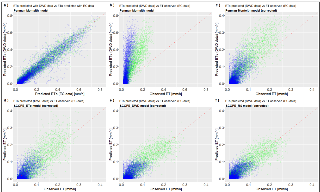
313 Figure 3. The relationship between ETo calculated using data from the meteorological stations and EC towers data (a), ETo from the DWD 314 data versus observed ET from the EC tower (b), ETo (corrected) versus observed ET (c), corrected SCOPE_ETo inputs versus observed ET 315 (d), corrected SCOPE_DWD versus observed ET (e), and corrected SCOPE_RS versus observed ET (e). The green dots represent the ROTH 316 site, and the blue dots represent the TUCC site. 317
