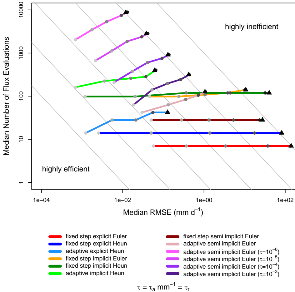
Figure 8. Relationship between computational efficiency and the numerical error, in the style of a Pareto front , where methods are more efficient if they have a low RMSE and a low number of flux evaluations. All medians are calculated across all 5 model structures, 20 parameter sets, and 3 spin up precipitation intensities. All six precipitation intensities for 5 day events are shown, where the light gray dot represents the lowest intensity event, darker gray dots represent increasingly intense precipitation events, and the dark gray 'x' black triangle represents the highest intensity event. Unless otherwise stated, adaptive methods use the FUSE default tolerances. Purple lines depict adaptive semi implicit Euler methods with error tolerances below the FUSE default, where the light brightest lightest purple method has the smallest error tolerance. Gray lines are visual aids of the form y = \frac{10^n}{x} , where n is an integer, such that moving and x and y respectively represent RMSE and number of flux evaluations (gray lines do not represent real data and are used only for visualization purposes) . Moving between adjacent gray lines represents an order of magnitude change in efficiency.
