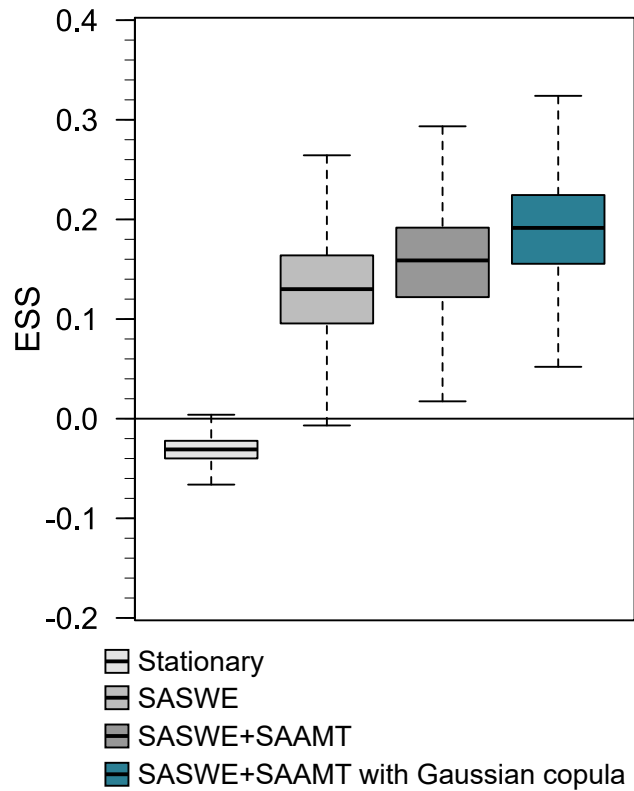
Figure 8. Energy Skill Score (ESS) distribution for four different BHM versions for a 0-month lead time for the calibration period (1965–2018). Higher values of the ESS indicate better model performance. The whiskers show the 95% credible intervals, boxes the inter-quartile range, and horizontal lines inside the boxes, the median. Outliers are not displayed. The light grey box denotes a stationary model, the grey box a nonstationary model with SASWE as a covariate, the dark grey box a nonstationary model with SASWE and SAAMT as covariates, and the dark turquoise model adds a Gaussian copula to model spatial dependence.
