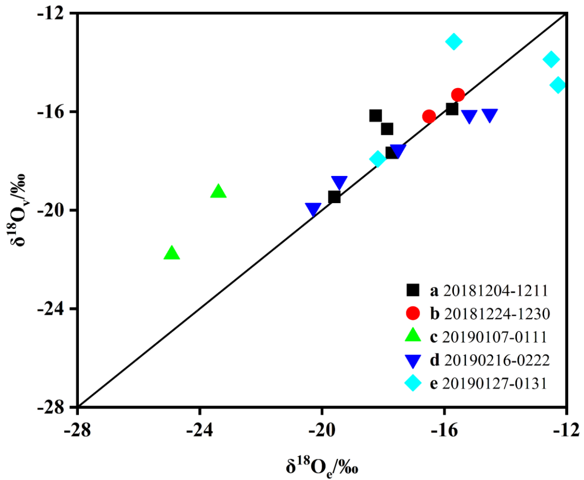
405 Fig 4. Relationship between observed ( \delta^{18}\text{O}_v ) and equilibrium ( \delta^{18}\text{O}_e ) vapor isotopic ratios in the five typical precipitation events. The isotopic composition of the water vapor theoretically in equilibrium with that of the precipitation ( \delta^{18}\text{O}_e ) is calculated by \delta_e = (\delta_p - \epsilon) / \alpha , where \epsilon is the equilibrium enrichment factor, and \alpha is the liquid-to-vapor equilibrium fractionation factor (Mercer et al., 2020). The solid black line is the line of equilibrium.
