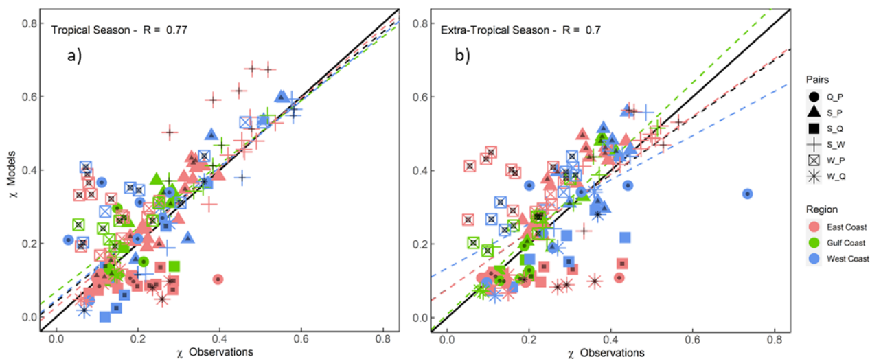
450 Figure 11: Scatter plot comparing dependence derived with Kendall's \tau and two-way sampling using seasonal maxima approach for tropical and extra-tropical seasons. Colours denote the location (separated into East, Gulf, and West coast) and markers represent the different variable pairs. Black dots on markers indicate significant difference in dependence between seasons. Dashed lines show linear regression fits corresponding to all data points (black) and for different subsets according to locations (coloured as outlined in the legend).
