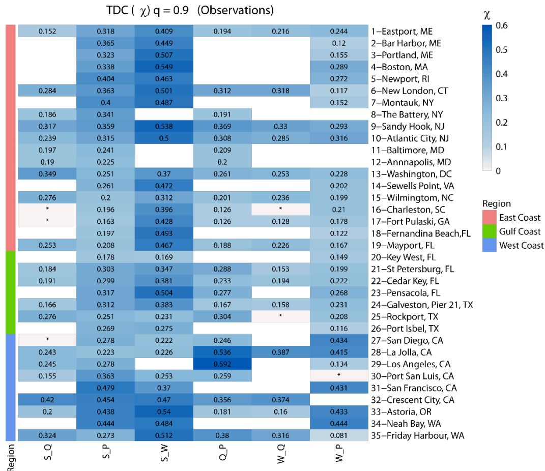
340 Figure 4: Tail dependence \chi between different pairs of flooding drivers for a threshold of q = 0.9 . Sites are grouped into East, Gulf, and West coast locations (see colours on the left and legend). The blue colour bar denotes tail dependence strength, blank squares indicate that data for the particular pair did not exist or that the number of overlapping years was less than 20, and squares with * indicate that dependence is not significant.
