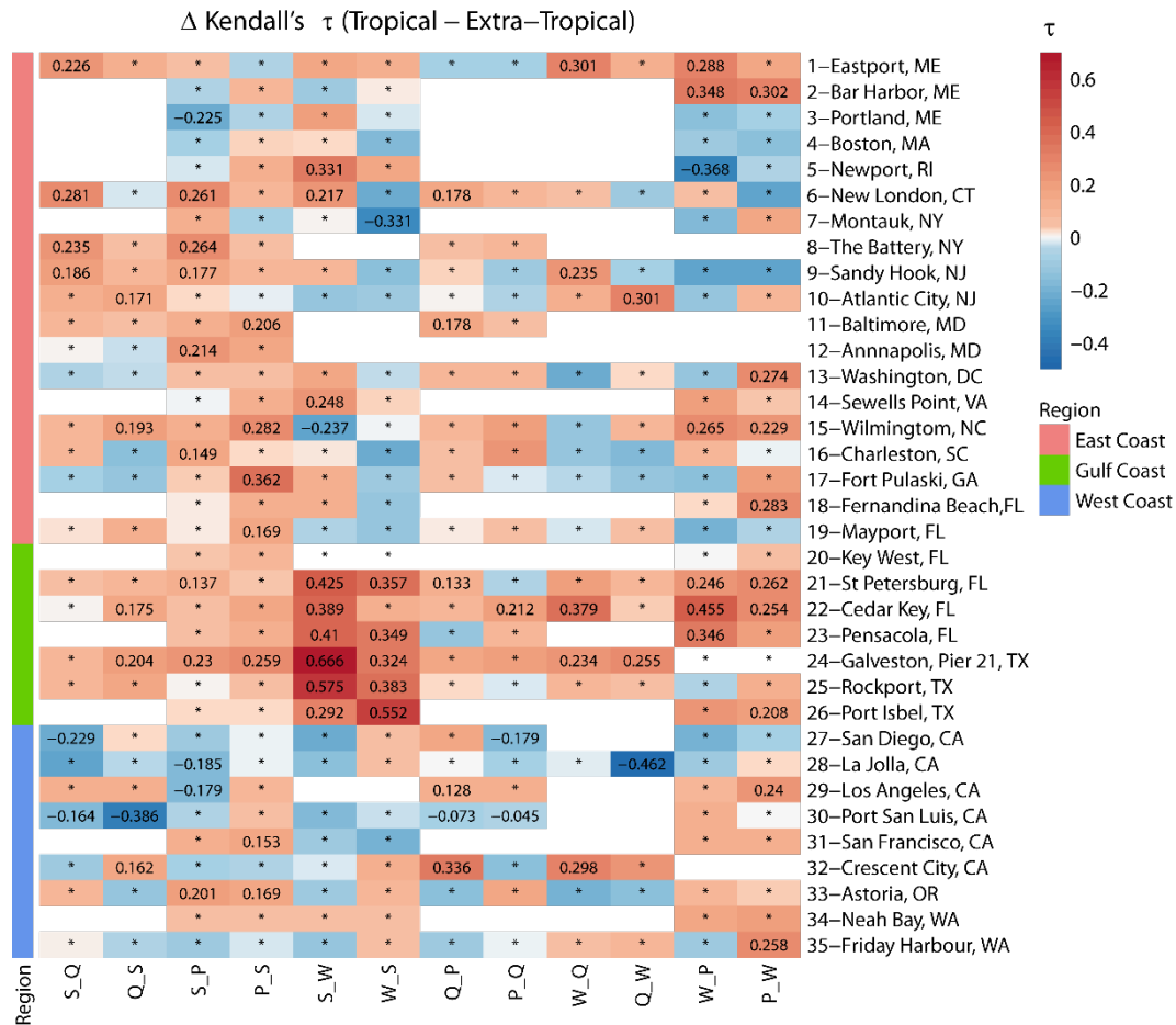
375 Figure 6: Heat map showing differences in Kendall's \tau derived from two-way sampling using seasonal maxima approach for tropical and extra-tropical seasons. Sites are grouped into East, Gulf, and West coast locations (see colours on the left and legend). The colour bar denotes the difference between \tau in the tropical versus extra-tropical season, where red colour denotes higher dependence in the tropical season, and blue colour denotes higher dependence in the extra-tropical season. Squares with * indicate that difference in dependence across seasons is not significant. Blank squares indicate that data for the particular pair did not exist or that the number of overlapping years was less than 20. 380
