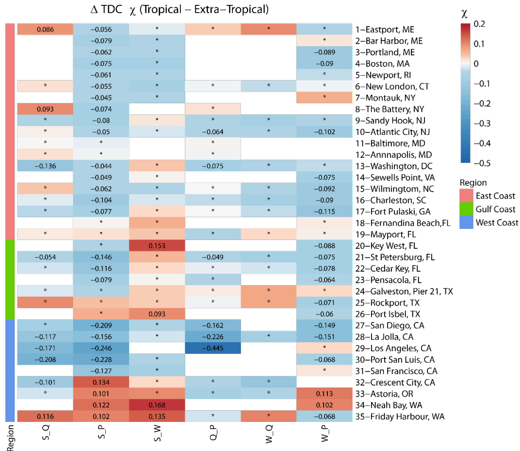
400 Figure 8: Heat map showing differences in tail dependence (for q=0.9 ) derived for tropical and extra-tropical seasons using daily time series of both variables. Sites are grouped into East, Gulf, and West coast locations (see colours on the left and legend). The colour bar denotes the difference between \chi in the tropical versus extra-tropical season, where red colour denotes higher dependence in the tropical season and blue colour denotes higher dependence in the extra-tropical season. Squares with * indicate that difference 405 in dependence across seasons is not significant. Blank squares indicate that data for the particular pair did not exist or that the number of overlapping years was less than 20.
