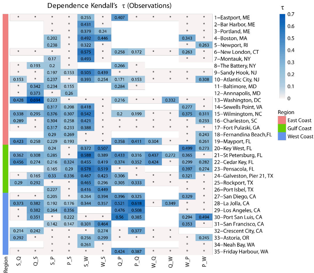
330 Figure 3: Dependence between different pairs of flooding drivers based on Kendall's \tau and two-way sampling using annual maxima. Sites are grouped into East, Gulf, and West coast locations (see colours on the left and legend). The blue colour bar denotes dependence strength, blank squares indicate that data for the particular pair didn't exist or that the number of overlapping years was less than 20 and squares with * indicate that correlation is not significant.
