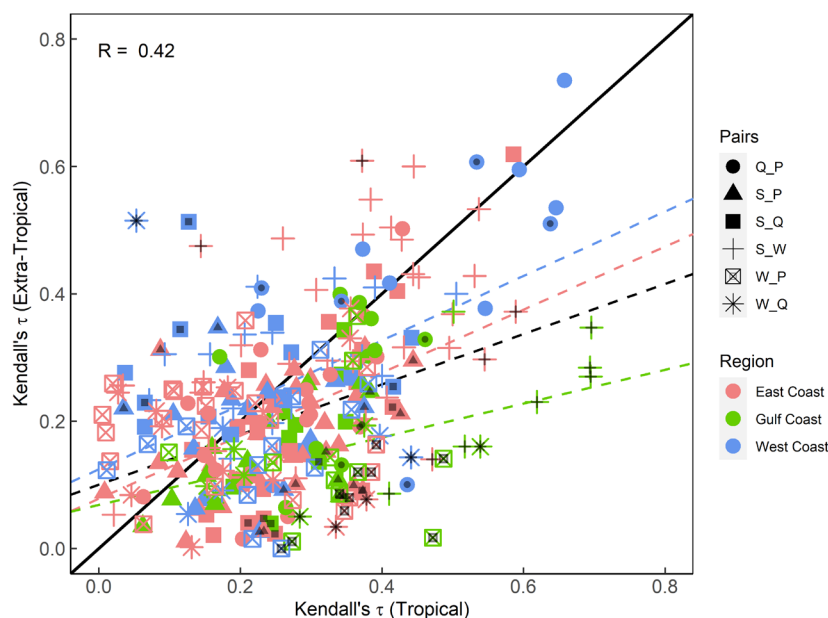
360 Figure 5: Scatter plot comparing dependence derived with Kendall's \tau and two-way sampling using seasonal maxima approach for tropical and extra-tropical seasons. Colours denote the location (separated into East, Gulf, and West coast) and markers represent the different variable pairs. Black dots on markers indicate significant difference in dependence between seasons. Dashed lines show linear regression fits corresponding to all data points (black) and for different subsets according to locations (coloured as outlined in the legend).
