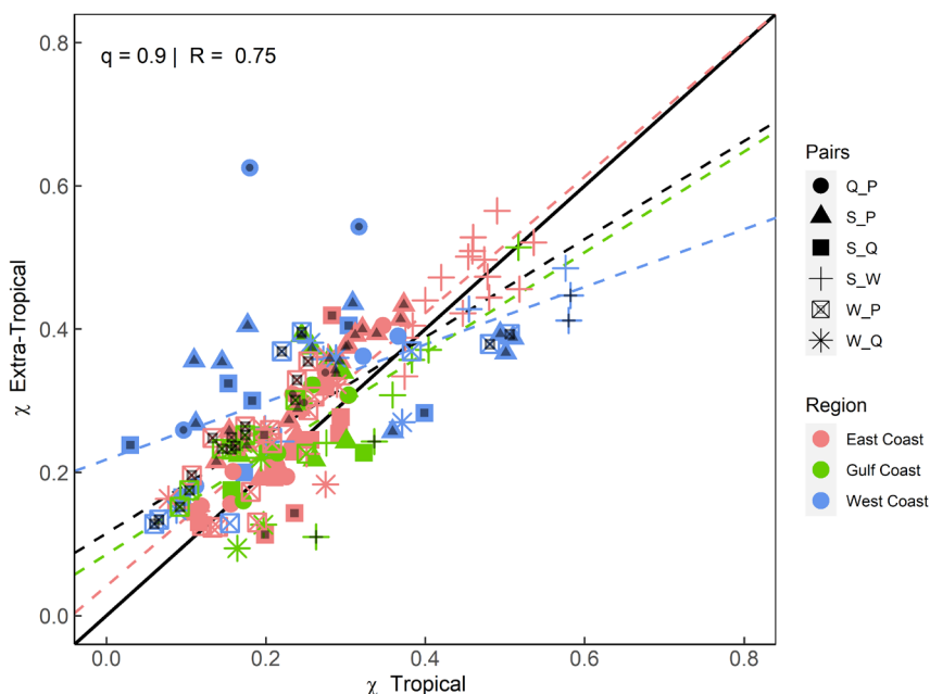
395 Figure 7: Scatter plot comparing tail dependence (for q=0.9 ) derived for tropical and extra-tropical seasons using daily time series of both variables. Colours denote the location (separated into East, Gulf, and West coast) and markers represent the different variable pairs. Black dots on markers indicate significant difference in tail dependence between seasons. Dashed lines show linear regression fits corresponding to all data points (black) and for different subsets according to locations (coloured as outlined in the legend).
