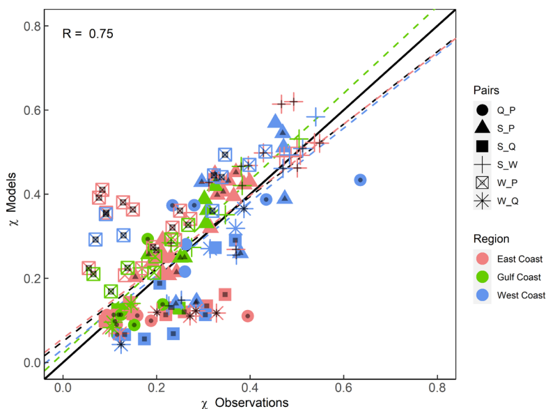
430 Figure 9: Scatter plot comparing extremal (tail) dependence (for q=0.9 ) derived using observations (x-axis) and models (y-axis) using daily time series of both variables. Colours denote the location (separated into East, Gulf, and West coast) and markers represent the different variable pairs. Black dots on markers indicate significant difference in tail dependence structure between observations and models. Dashed lines show linear regression fits corresponding to all data points (black) and for different subsets according to locations (coloured as outlined in the legend).
