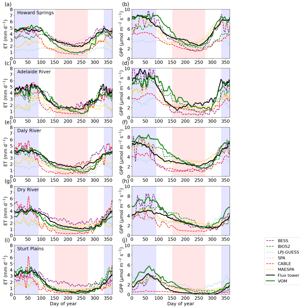
Figure 2. Ensemble years of evapo-transpiration (ET) and gross primary productivity (GPP) for the VOM (darkgreen), flux tower observations (black) and the models BESS (dashed purple), BIOS2 (dashed green), LPJ-GUESS (dashed lightblue), SPA (dashed pink), CABLE (dashed red) and MAESPA (dashed yellow) from Whitley et al. (2016), all smoothed by a 7-day moving average. The ensemble years are calculated for the overlapping time periods with the flux tower observations (see Table S8.1 in Supplement S8). The dry season (June-Sept.) is indicated by a red shading, the wet season (Dec.-March) by a blue shading.
