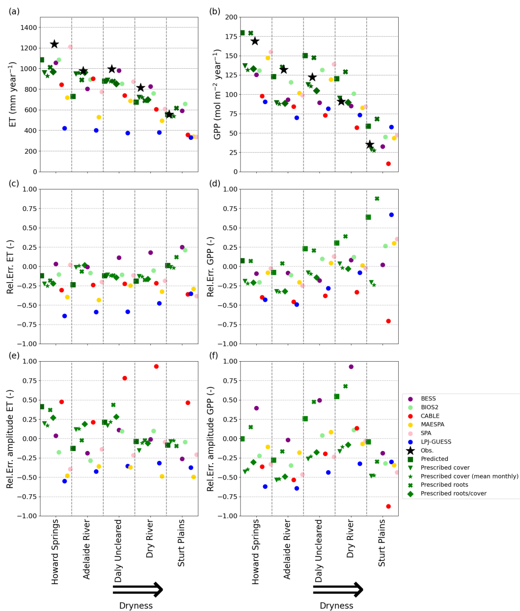
Figure 3. Performance of the VOM, the VOM with prescribed cover, prescribed roots, prescribed roots and cover, and the models analyzed by Whitley et al. (2016) in comparison with flux tower observations. a) and b): Mean annual evapo-transpiration (ET) and gross primary productivity (GPP); c) and d): the relative error of the mean annual ET and GPP; e) and f): the relative error for the mean seasonal amplitude of ET and GPP. All metrics for all models are calculated for the overlapping time period of the model time period and the flux tower time period for each site (see Table Table S8.1 in Supplement S8).
