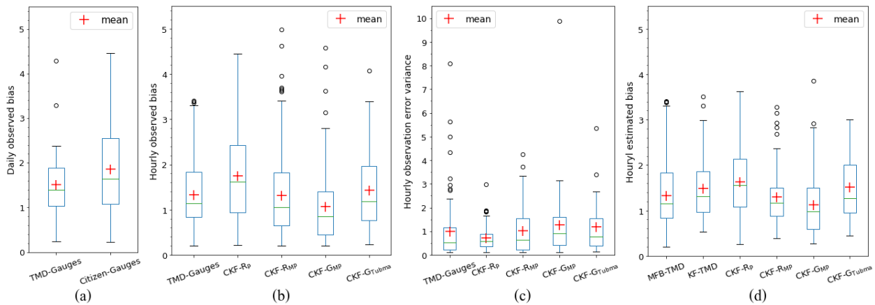
455 Figure 56: Comparison of (a) daily observed mean field bias based on TMD rain gauges in the region and the citizen rain gauges in the Tubma basin, (b) hourly observed mean field bias based on TMD rain gauge observations and downscaled citizen rain gauge observations, (c) hourly observation error variances and (d) hourly estimated mean field bias obtained based on MFB and the five different KF approaches. Bias calculations cover 16 citizen gauges in the Tubma basin and 14 TMD gauges within 100-90 km radius from the Tubma basin. Hourly scale calculations for the citizen gauges (CKF) are based on 4four different sub-daily interpolation scenarios ( R_P , R_{MP} , G_{MP} and G_{Tubma} , Table 3). 460
