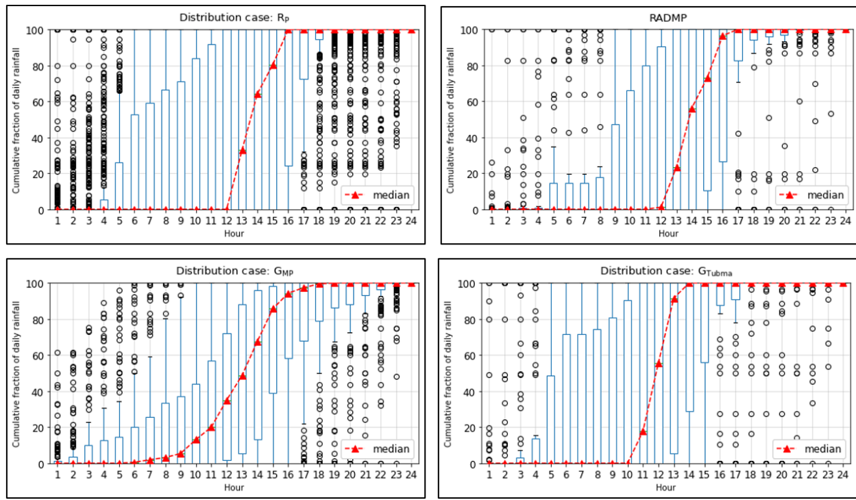
Figure 45: Variation of fraction of 24-hour rainfall for each rainfall distribution scenario.
