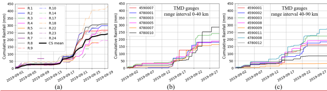
550 Figure 910: Comparison of mass curves of hourly rainfall among various rain-gauge locations (a) the citizen rain gauges located in the Tubma (b) TMD rain gauges within 0-40 km radius from the Tubma basin (c) TMD rain gauges within 40-90 km radius from the Tubma basin.
