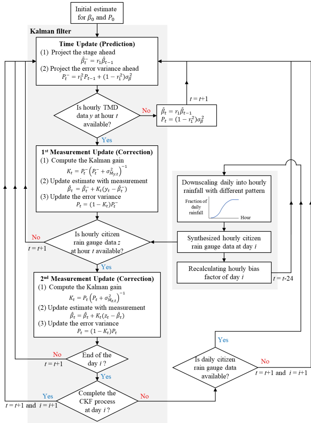
Figure 34: A diagram of the procedure of Kalman filter combined with the citizen rain gauge data (CKF)
