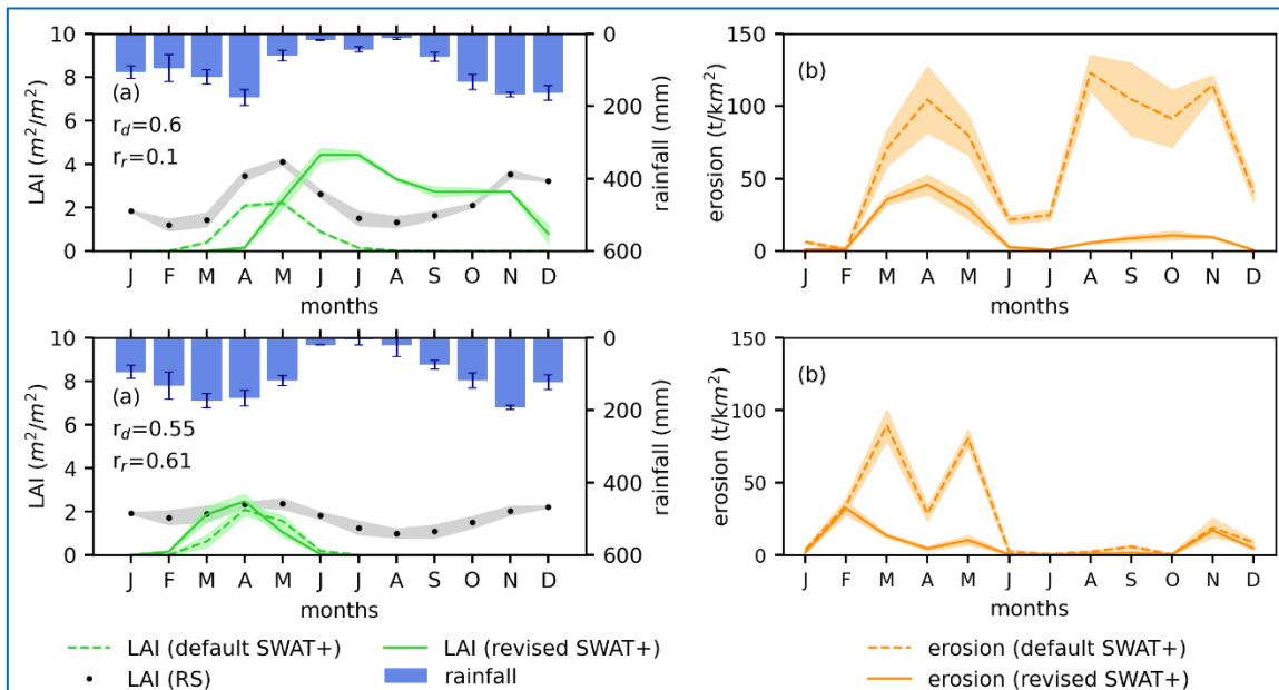
475 Figure A4: (a) Monthly mean and standard deviation (bands) of (a) LAI and (b) erosion comparison for rainfed maize; Monthly mean and standard deviation (bands) of (a) LAI and (b) erosion comparison for rainfed soy; in the Victoria basin. The LAI correlation coefficients ( r_d for the default SWAT+ model and r_r for the revised SWAT+ model)
