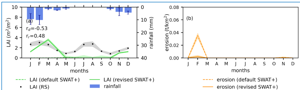
305 Figure 8: Monthly mean and standard deviation (bands) of LAI (a) and erosion (b) comparison for irrigated wheat; in the Nile delta. The LAI correlation coefficients ( r_d for the default SWAT+ model and r_r for the revised SWAT+ model)
