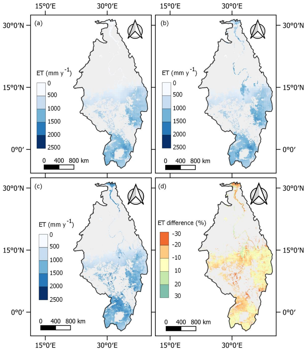
365 Figure 10: Spatial distribution of agricultural ET; a) default SWAT+ model ET, b) revised SWAT+ model ET, c) WaPOR ET, d) ET difference (WaPOR ET – revised SWAT+ model ET)
