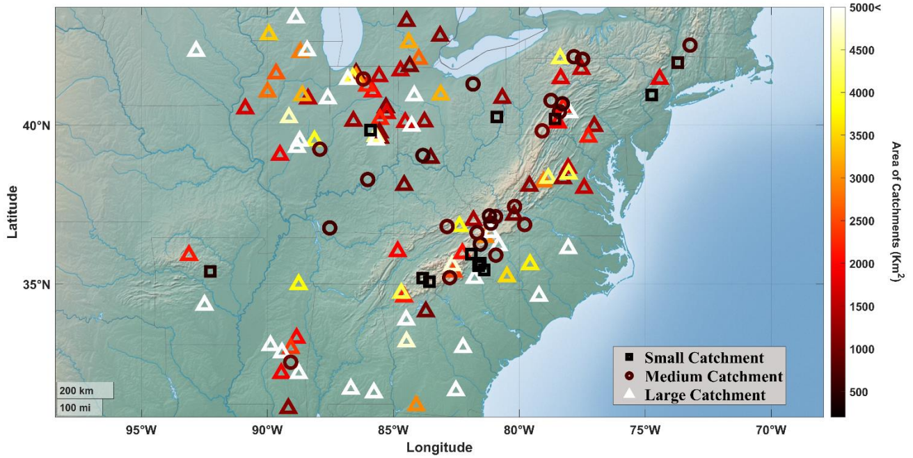
Figure 1: Distribution of catchments across North Eastern America. Squares, Circles and triangles symbols correspond to small, medium and large catchments respectively.
