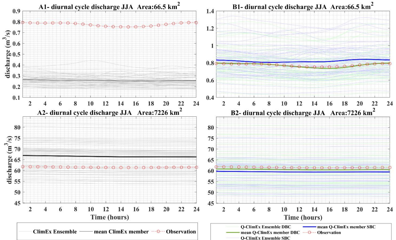
Figure 10: Annual diurnal cycle of discharge in JJA (Jun, July, August) before bias correction (first column: A1 and A2) and after bias correction (second column: B1 and B2) for two selected catchments. First row is for catchment 02143040 (small size classification) and second row is for catchment 02156500 (large size classification). The observations are shown in red. Streamflow simulations using uncorrected ClimEx members are shown in light grey, and the ensemble mean is in black. Simulations using bias corrected data are in light blue (SBC) and light green (DBC) with the corresponding dark colours showing the ensemble mean. Time is local with 24h corresponding to midnight.
