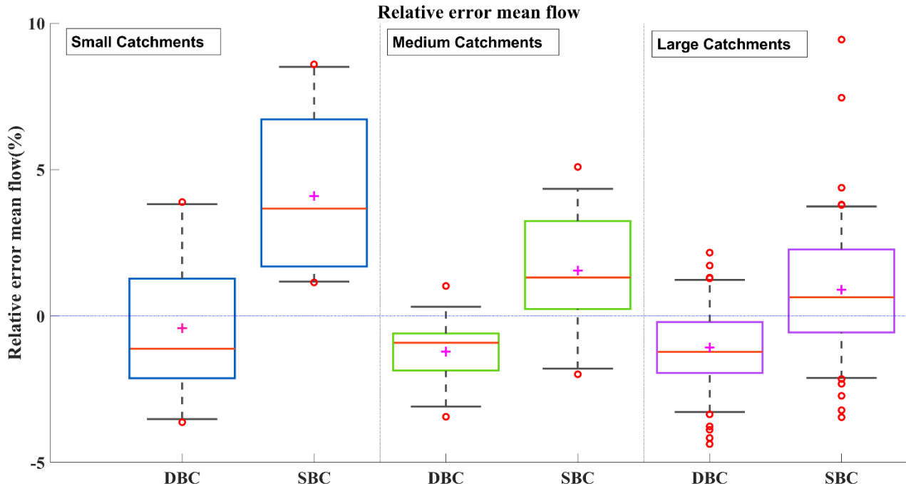
865 Figure 7: Comparing relative error of mean flow with diurnal cycle bias correction (DBC) and standard bias correction (SBC) in three area categories.
