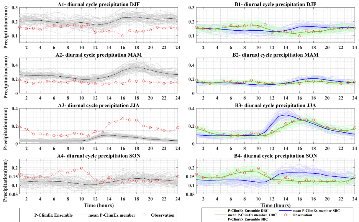
845 Figure 4: Annual diurnal cycle of precipitation before bias correction (first column: A1 to A4) and after bias correction (second column: B1 to B4) for catchment 02143040. Each row corresponds to a different season: DJF (December, January, February), MAM (March, April, May), JJA (Jun, July, August), SON (September, October, November). The right-hand side shows both bias correction methods: Standard Bias Correction (SBC) and Diurnal Bias Correction (DBC). The observations are shown in red. Raw (uncorrected) ClimEx data is in grey, SBC is in blue and DBC is in green. The envelope defined by all 50 ClimEx members are shown in the corresponding light colours, whereas the dark coloured lines display the ensemble mean. Time is local with 24h corresponding to midnight.
