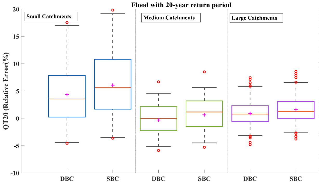
880 Figure 9: Distribution of the relative error ((\text{model-obs})/\text{obs} \times 100\%) for the 20-year flood QT20. Boxplots for both bias correction methods (DBC and SBC) are constructed from the distribution of relative errors from all catchments within each size class (small, medium, and large).
