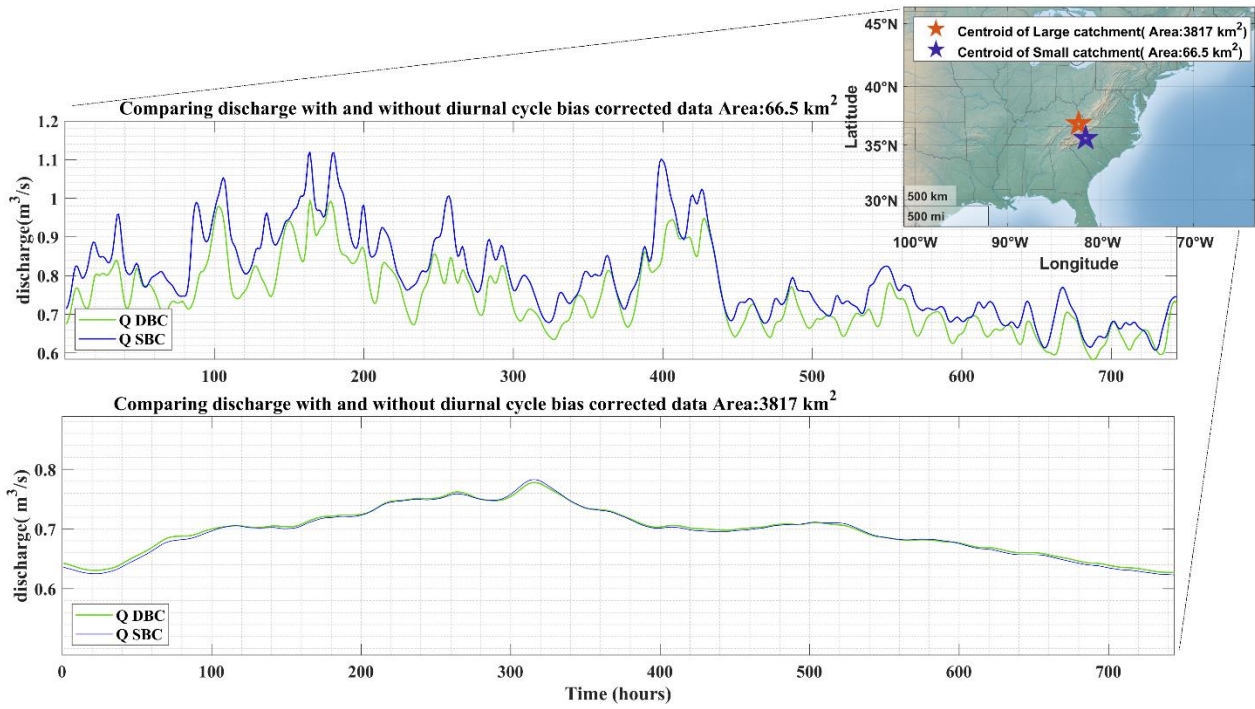
Figure 6: Hydrographs of two sampled catchments (small and large size surface area) for the month of July (744 hours = 31 days × 24 hours).
