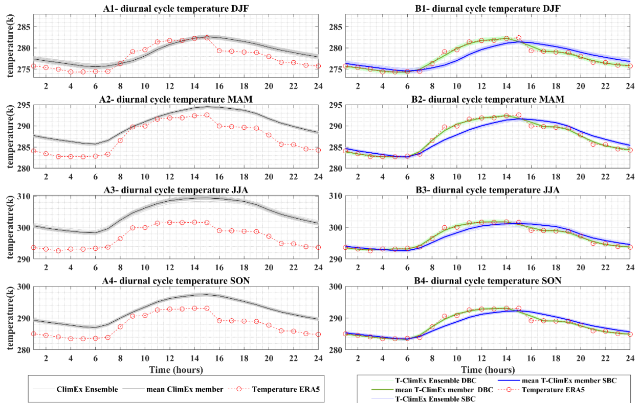
825 Figure 3: Annual diurnal cycle of temperature before bias correction (first column: A1 to A4) and after bias correction (second column: B1 to B4) for catchment 02143040. Each row corresponds to a different season: DJF (December, January, February), MAM (March, April, May), JJA (Jun, July, August), SON (September, October, November). The right hand side shows both bias correction methods: Standard Bias Correction (SBC) and Diurnal Bias Correction (DBC). The observations (ERA5) are shown in red. Raw (uncorrected) ClimEx data is in grey, SBC is in blue and DBC is in green. The envelope defined by all 50 ClimEx members are shown in the corresponding light colours, whereas the dark coloured lines display the ensemble mean. Time is local with 24h 830 corresponding to midnight.
