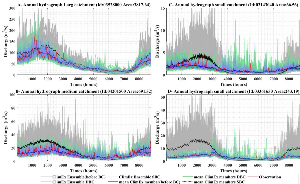
855 Figure 5: Hydrograph annual cycles for four selected catchments. Catchments A and B are classified as large and medium size respectively. Catchments C and D are classified as small. 0 represents January first at 0h00, and 8760 is December 31st at 24h00.
