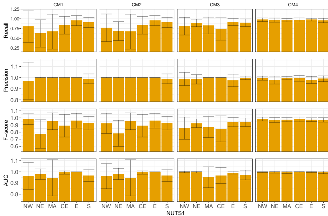
Figure 8. Performance metrics (recall, precision, F-score and AUC) of the classification Random Forest model when performing a repeated 10-fold cross-validation using all the data. All counting methods are shown. The error bars show the standard deviation of these metrics.
