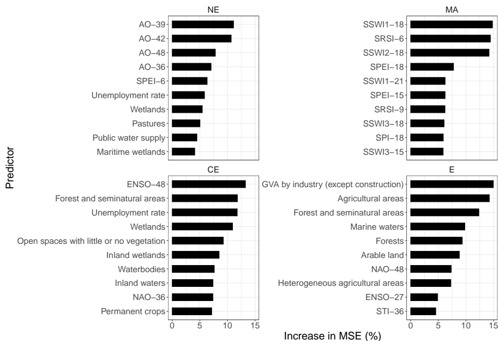
Figure 12. Predictor importance when using regression Random Forest models built with vulnerability factors in addition to the drought indices. Counting method CM1 is used.
