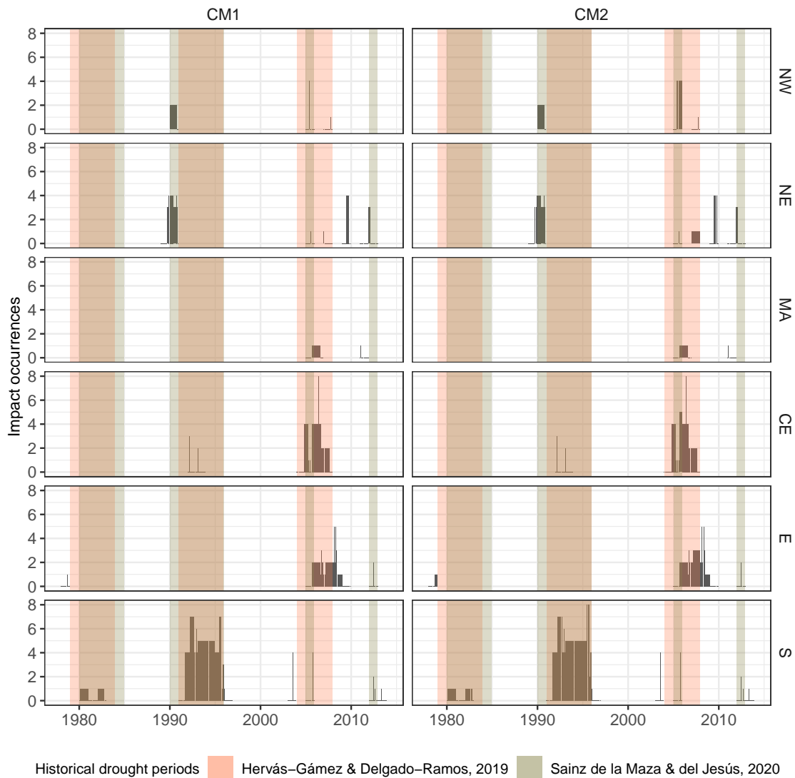
Figure 3. Monthly DIOs in each sub-region from 1975 to 2013 using the most censoring counting methods (CM1 and CM2). Important historical drought periods identified in other studies are highlighted.
