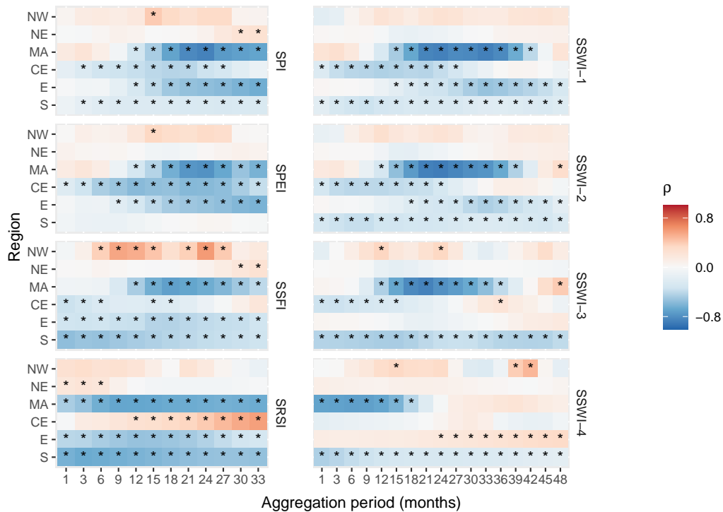
Figure 5. Correlation coefficients ( \rho ) between time series of drought indicators and impact occurrences for each sub-region using a more censoring counting method (CM3). Stars indicate significance ( p < 0.05 ).
