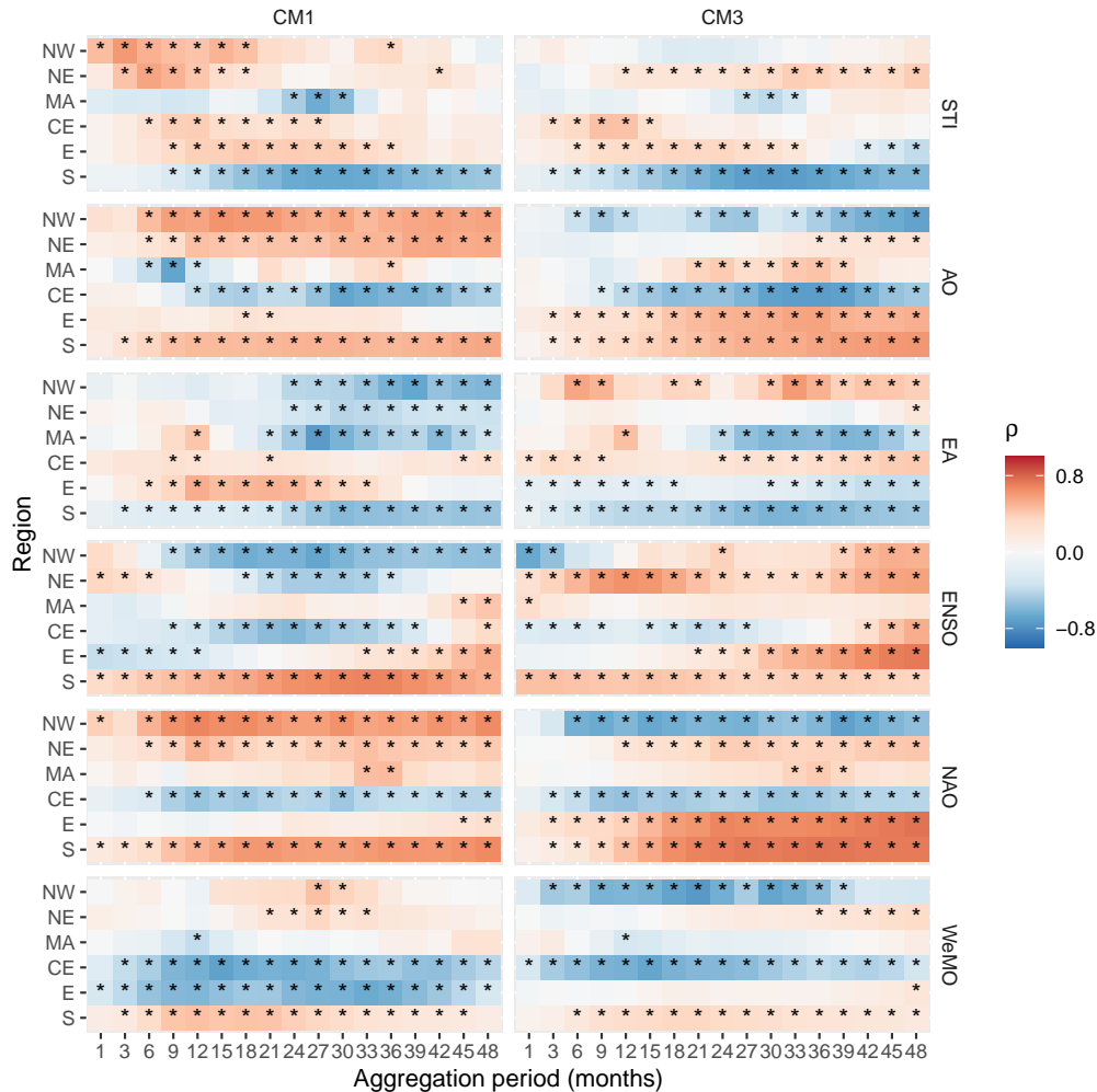
Figure 6. Correlation coefficients ( \rho ) between time series of climate indices and impact occurrences for each sub-region using one of the most (CM1) and third most (CM3) censoring counting methods. Stars indicate significance ( p < 0.05 ).
