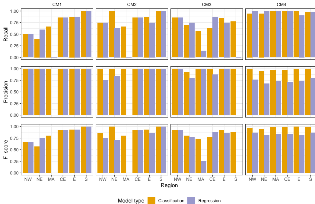
Figure 9. Performance metrics (recall, precision and F-score) of the Random Forest models when training and validating the models on 75% and 25% of the data. All counting methods are shown. The regression model test predictions were converted into binary outcomes using a threshold of 1.25 DIOs.
