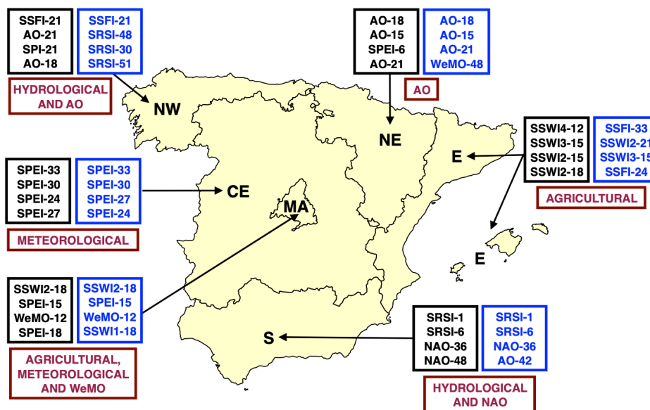
Figure 11. Map with the top four predictors for each sub-region when using the regression Random Forest models and the two most censoring counting methods, in blue and black respectively. The “best” type of predictors for each sub-region are in red.
