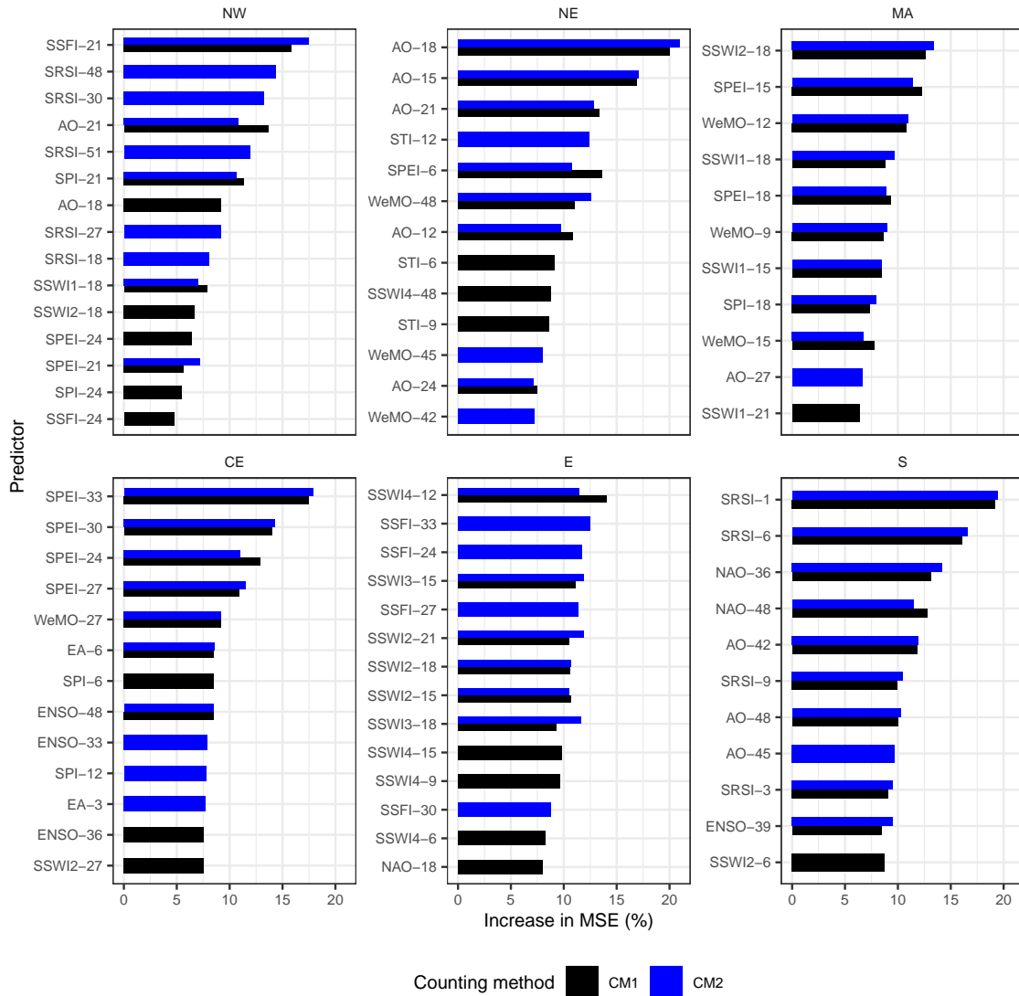
Figure 10. Predictor importance when using the regression Random Forest models and the two most censoring counting methods. The top 10 predictors for each counting method and sub-region are shown.
