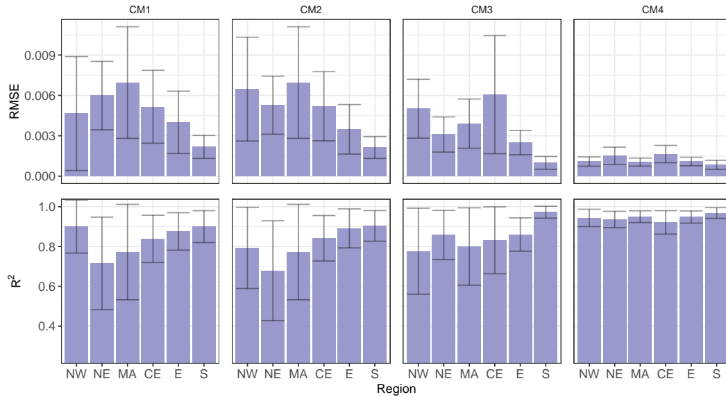
Figure 7. Performance metrics (RMSE and R^2 ) of the regression Random Forest model when performing a repeated 10-fold cross-validation using all the data. All counting methods are shown. The error bars show the standard deviation of these metrics.
