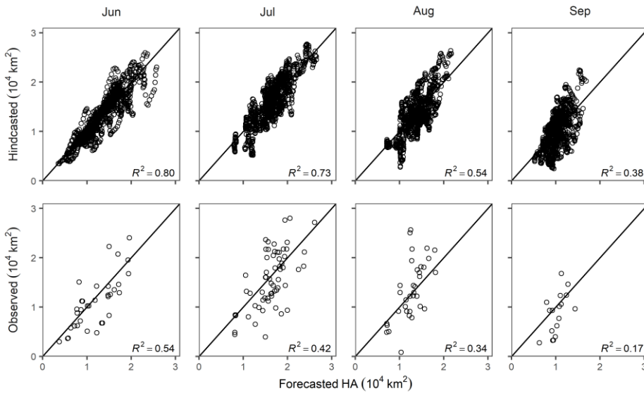
255 Figure 34: Month-by-month comparison of the daily hindcasted (top) and observed (geostatistically estimated, bottom) shelfwide HA versus pseudo-forecasted HA. Diagonal line represents perfect prediction.
