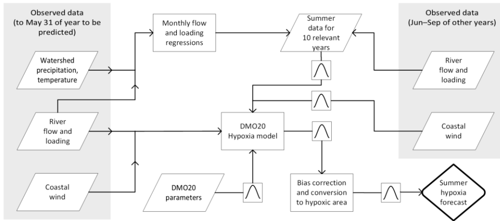
Figure 12: Flowchart summarizing processes and data inputs required to generate the hypoxia hindcast (A) and pseudo-forecast (B) for a given year. Parallelograms represent data inputs and Bayesian posterior parameter distributions. Rectangles represent forecasting computations. Squares with bell-shaped curves indicate steps that propagate uncertainty (including stochastic hydrometeorology).
