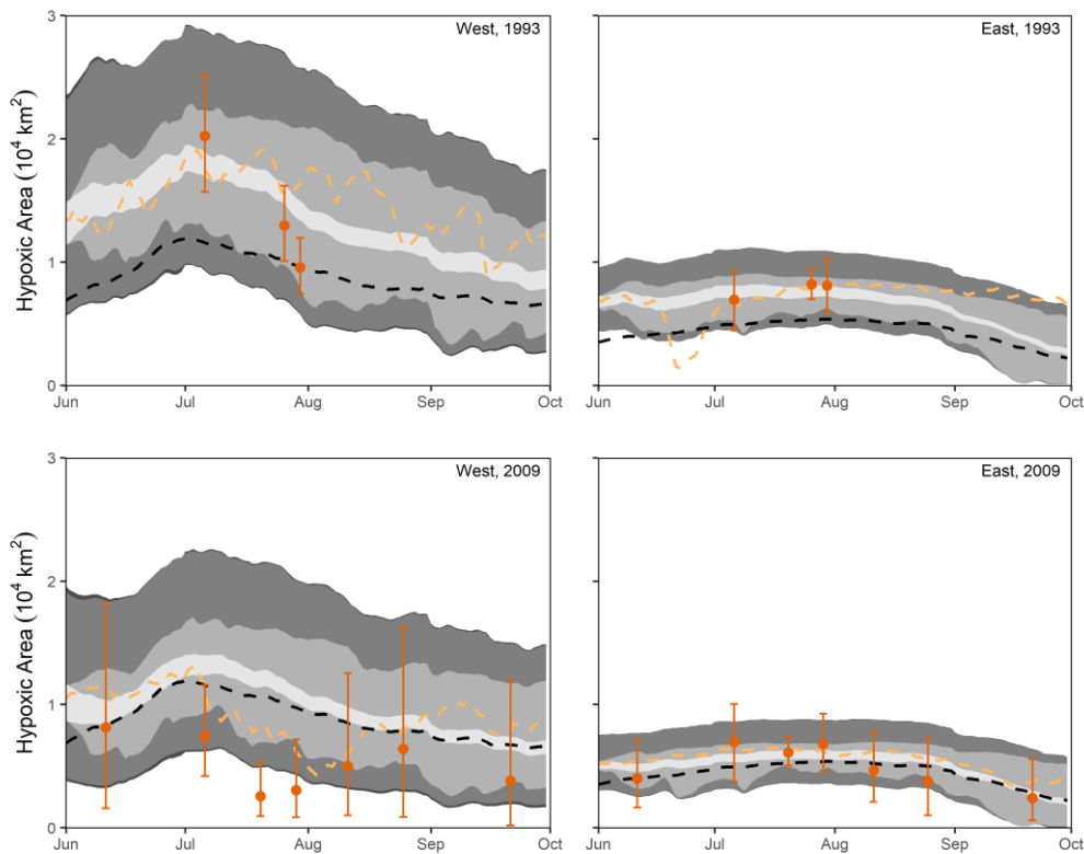
295 Figure 45: Daily pseudo-forecasts of HA for the west and east sections in 1993 (top) and 2009 (bottom), including 95% IQR of the predictive distribution, distinguishing between i) parameter, ii) riverine and meteorological inputs, iii) mechanistic model residual error and iv) regression regressions related to transformation of BWDO to HA and bias adjustment uncertainties (shades of gray from darkest to lightest to darkest). Yellow dashed line is hindcasted estimate, black dashed line is the 32 year average hindcast, orange points and error bars represent the mean and associated 95% 300 confidence interval of the (geostatistically estimated) hypoxia observations.
