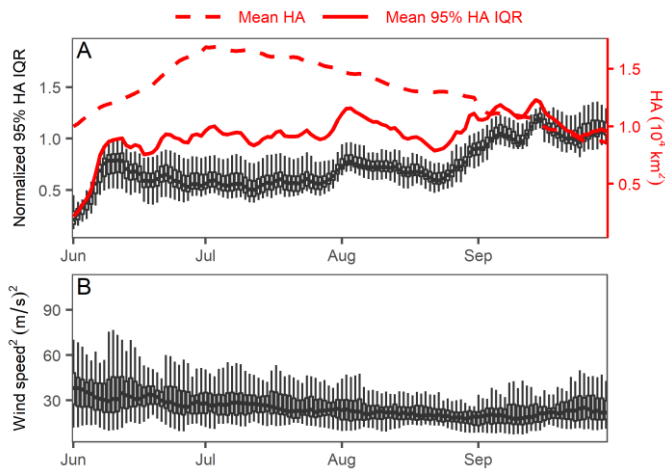
Figure 56: (A) Boxplots represent daily pseudo-forecasted normalized IQR (IQR/HA) including uncertainty due to variability in parameters, riverine inputs and meteorology. Red dashed and solid lines show the daily mean HA and (non-normalized) IQR, respectively; (B) Boxplots show 14 day weighted average squared wind speed near the west shelf section. Boxplots represent interannual variability in the results. The center of each box is the median, while whiskers extend to the extreme value or 1.5 times the IQR of the corresponding variable (whichever is less).
