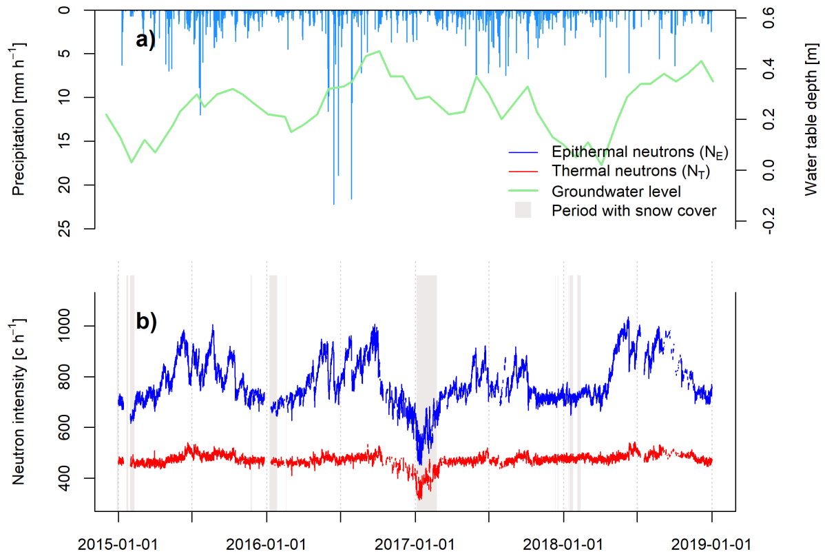
Figure 2. Field observations for the period from January 2015 to December 2018: a) hourly rainfall and approximate monthly groundwater level measurements table depth in far-field peatland soils , b) the corrected neutron intensities in the thermal ( N_T ) and epithermal energy range ( N_E ) (b).
