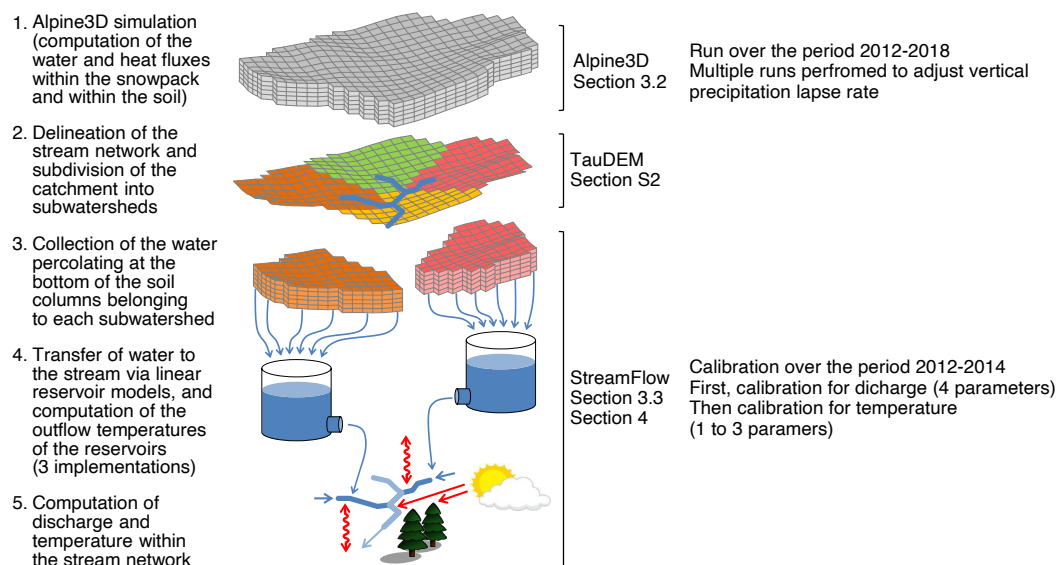
Figure 2. Details of the models' workflow. The calibration and validation periods indicated hold-are valid for all catchments except for the Eulach catchment (where the periods 2015-2016 and 2017-2018 are used instead). Figure adapted from (Gallice et al., 2016).
