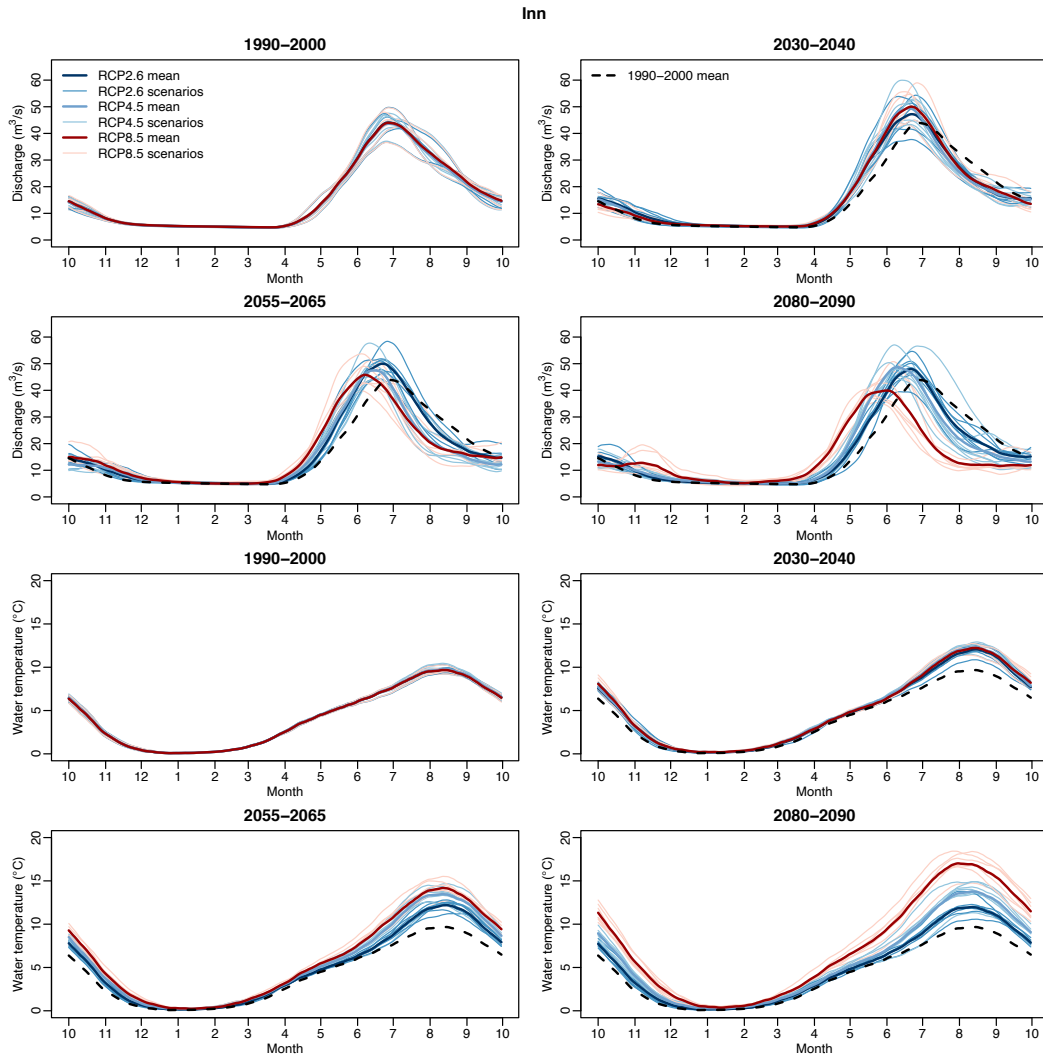
Figure 7. Annual cycle of discharge (top) and river temperature (bottom) for of the Inn catchment. The cycles are obtained by computing the average for each day of the year and by applying a circular moving average of 30 days. Dark lines show the mean for each RCP over each period, light lines show individual scenarios. Black dashed lines indicate the mean over the reference period 1990-2000 (only shown in subsequent periods to ease comparison).
