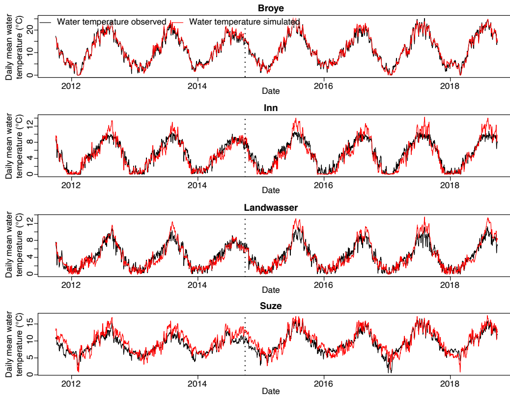
Figure 3. Daily mean water temperature observed (black) and simulated (red) over the calibration periods (left of the dashed-dotted line) and over the validation period (right of the dashed-dotted line) for four catchments: the Broye (Swiss Plateau), the Inn (Alpine), the Landwasser (Alpine), and the Suze (Swiss Plateau). These four catchments were chosen to represent the variation in the catchment type. Note that the extent of the y-axes (daily mean water temperature range) is different for every panel. Other catchments are shown in Section S6.
