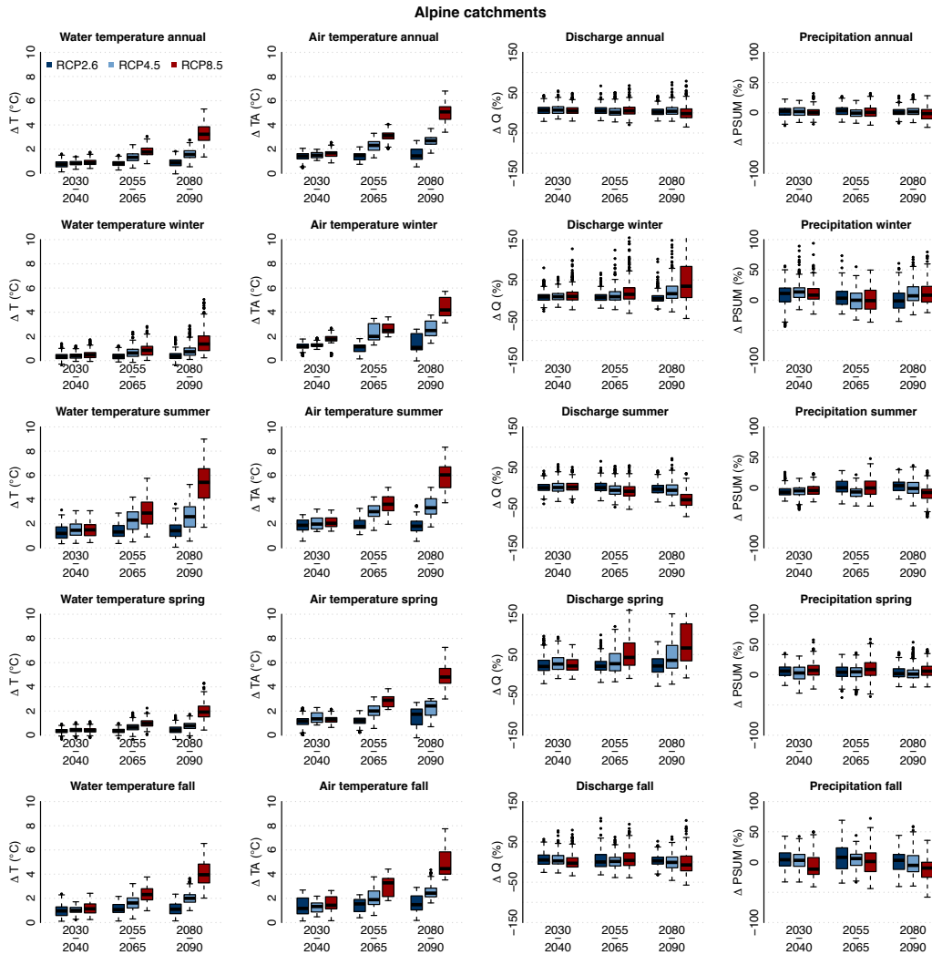
Figure 5. Changes in water-river temperature ( \Delta T ), air temperature ( \Delta TA ), discharge ( \Delta Q ), and precipitation ( \Delta PSUM ), from left to right column, over the periods 2030-2040, 2055-2065, and 2080-2090 and for the 3 RCPs, compared to the reference period 1990-2000, averaged over all considered Alpine catchments. Row 1 shows the annual change, row 2 the winter seasonal change, row 3 the summer seasonal change, row 4 the spring seasonal change, and row 5 the fall seasonal change.
