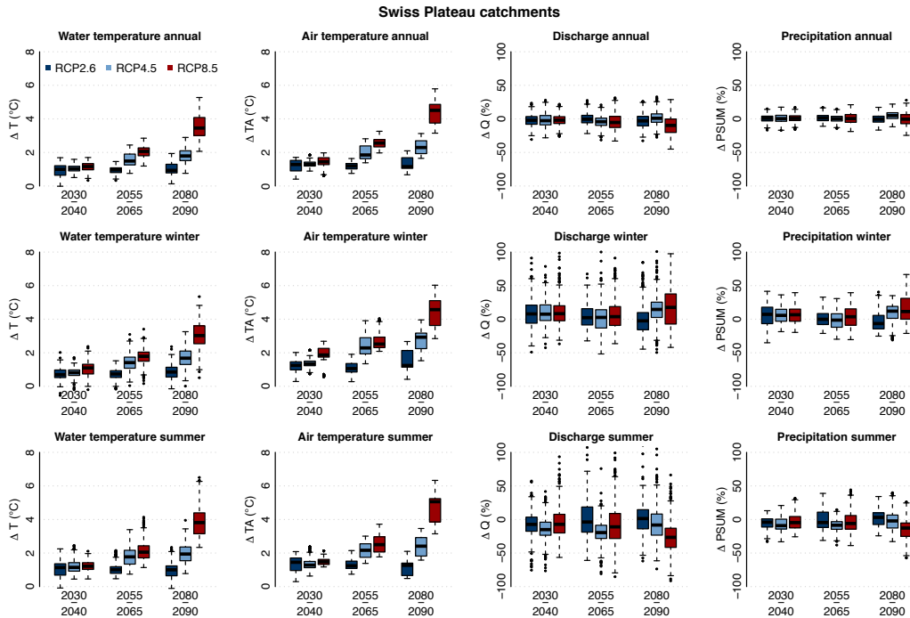
Figure 4. Changes in water-river temperature ( \Delta T ), air temperature ( \Delta TA ), discharge ( \Delta Q ), and precipitation ( \Delta PSUM ), from left to right column), over the periods 2030-2040, 2055-2065, and 2080-2090, compared to the reference period 1990-2000 for the Swiss Plateau catchments and for the 3 RCPs. The first row shows the annual changes, the second row the winter seasonal changes, and the last row the summer seasonal changes.
