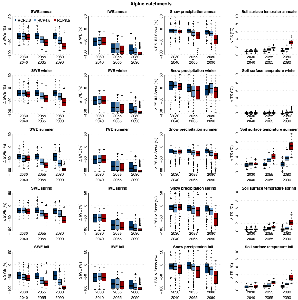
Figure 6. Change-Changes in snow water equivalent in the catchments ( \Delta SWE ), in ice water equivalent (mass stored-in-glaciers-of-glacier ice and in-snow in glacier pixels) in the catchments ( \Delta IWE ), in solid precipitation ( \Delta PSUM snow), and in soil surface temperature ( \Delta TS ), from left to right column over the periods 2030-2040, 2055-2065, and 2080-2090 and for the 3 RCP scenarios, compared to the reference period 1990-2000, averaged over all considered Alpine catchments. Row 1 shows the annual change, row 2 the winter seasonal change, row 3 the summer seasonal change, row 4 the spring seasonal change, and row 5 the fall seasonal change.
