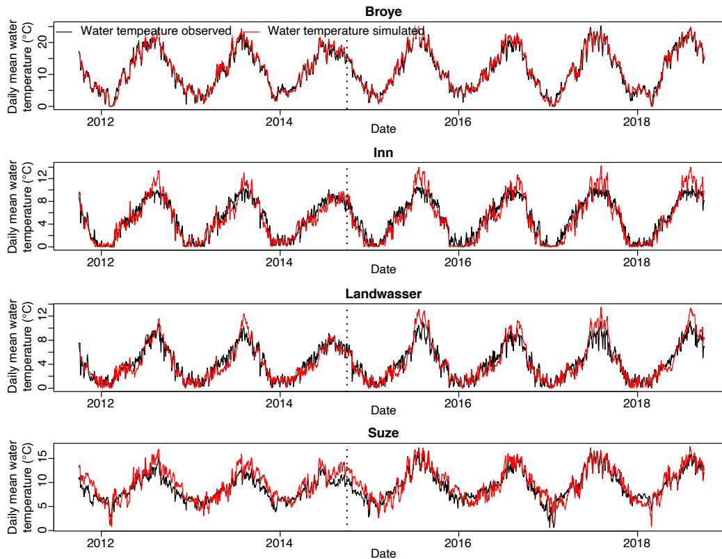
Figure 3. [PREVIOUSLY FIGURE 2] Water-Daily mean water temperature observed (black) and simulated (red) over the calibration periods (left of the dashed line) and over the validation period (right of the dashed line) for four catchments: the Broye (Swiss Plateau), the Inn (Alpine), the Landwasser (Alpine), and the Suze (Swiss Plateau). These four catchments were chosen to represent the variation in the catchment type. Note that the extent of the y-axes (daily mean water temperature range) is different for every panel. Other catchments are shown in Section S6.
