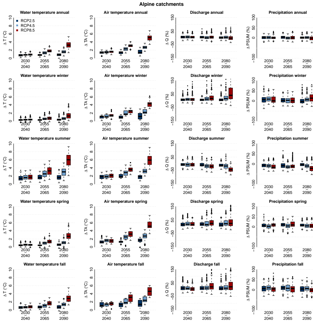
Figure 6. [PREVIOUSLY FIGURE 10] Changes in water temperature ( \Delta T ), air temperature ( \Delta TA ), discharge ( \Delta Q ), and precipitation ( \Delta PSUM , from left to right column) over the periods 2030-2040, 2055-2065, and 2080-2090 and for the 3 RCPs, compared to the reference period 1990-2000, averaged over all considered Alpine catchments. Row 1 shows the annual change, row 2 the winter seasonal change, row 3 the summer seasonal change, row 4 the spring seasonal change, and row 5 the fall seasonal change.
