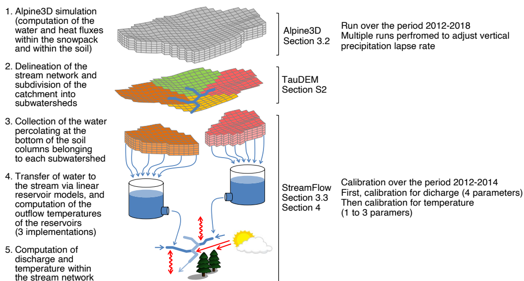
Figure 2. [NEW FIGURE] Details of the models' workflow. The calibration and validation periods indicated hold for all catchments except for the Eulach catchment (where the periods 2015-2016 and 2017-2018 are used instead). Figure adapted from (Gallice et al., 2016).
