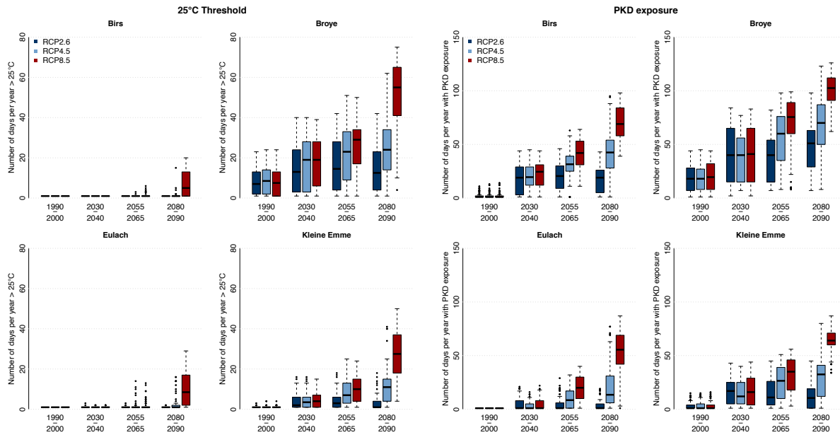
Figure 5. [PREVIOUSLY FIGURE 8 AND 9, FIGURES 6 AND 7 OF THE ORIGINAL MANUSCRIPT HAVE BEEN MOVED TO SUPPLEMENTARY MATERIAL FIGURES S73 AND S72] Left: Number of days per year when the temperature is above the threshold of 25°C, for each year in each time period and for each scenario, for 4 Swiss Plateau catchments. These four catchments were chosen to represent the variation in the Swiss Plateau catchment type. Right: Number of days per year when salmonid populations are exposed to PKD, based on the metric presented in the work of Michel et al. (2020), for each year in each time period and for each scenario, for 4 Swiss Plateau catchments. These four catchments were chosen to represent the variation in the Swiss Plateau catchment type.
