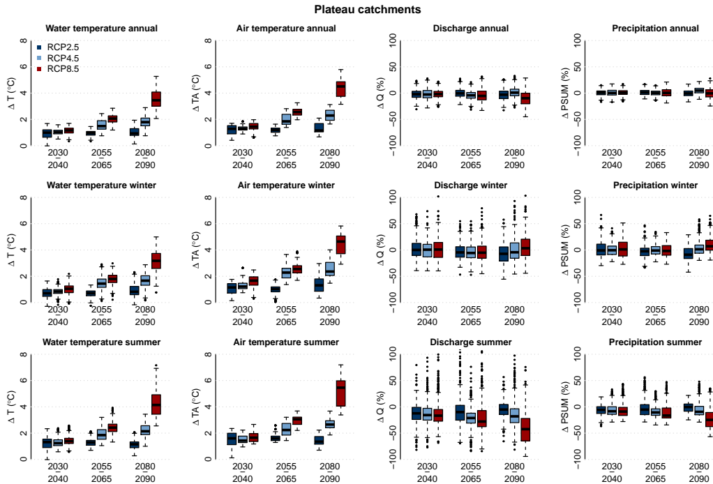
Figure 4. [PREVIOUSLY FIGURE 5, FIGURES 3 AND 4 OF THE ORIGINAL MANUSCRIPT HAVE BEEN MOVED TO SUPPLEMENTARY MATERIAL FIGURES S52 AND S34] Changes in water temperature ( \Delta T ), air temperature ( \Delta TA ), discharge ( \Delta Q ), and precipitation ( \Delta PSUM , from left to right column) over the periods 2030-2040, 2055-2065, and 2080-2090, compared to the reference period 1990-2000 for the Swiss Plateau catchments and for the 3 RCPs. The first row shows the annual changes, the second row the winter seasonal changes, and the last row the summer seasonal changes.
