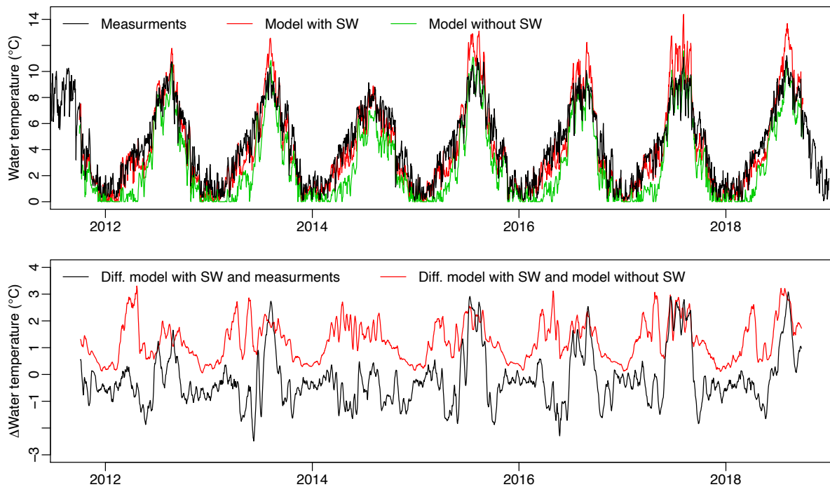
Figure 8 – Top: Measured (black) and simulated water temperature (red with shortwave radiation, green without shortwave radiation) for the Alpine Lonza catchment. Bottom: Difference between measured and modeled (with shortwave radiation) water temperature (black), and difference between water temperature modeled with and without shortwave radiation (red).
