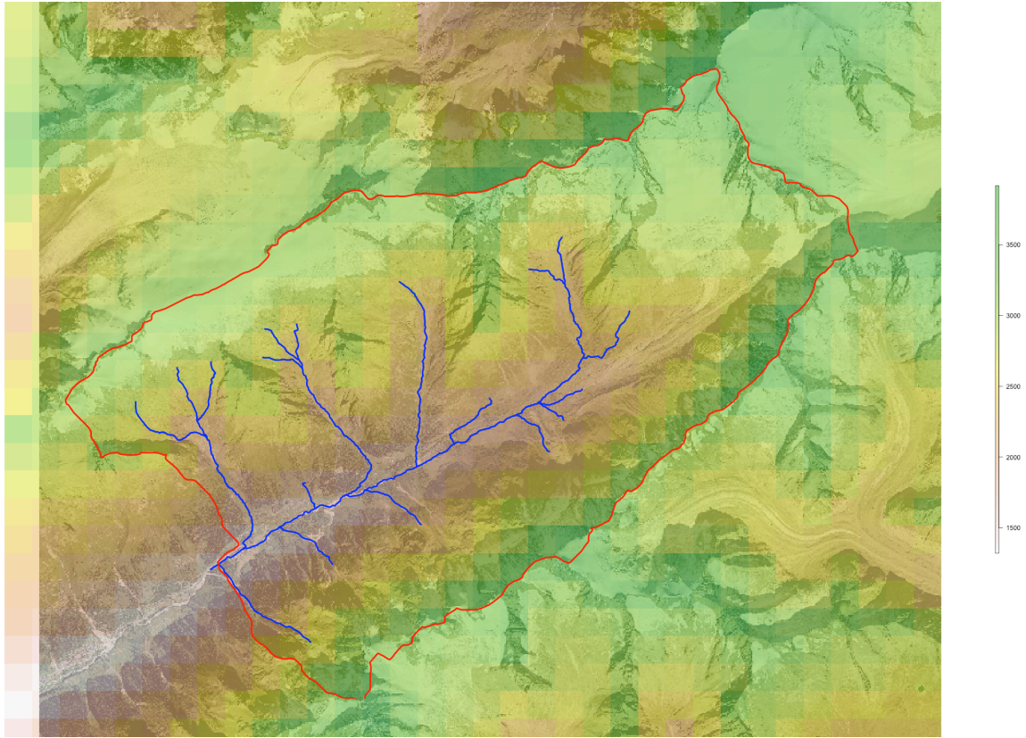
Figure 7 – Lonza catchment (red) and river course (blue) with DEM added on top. Source: Swisstopo
