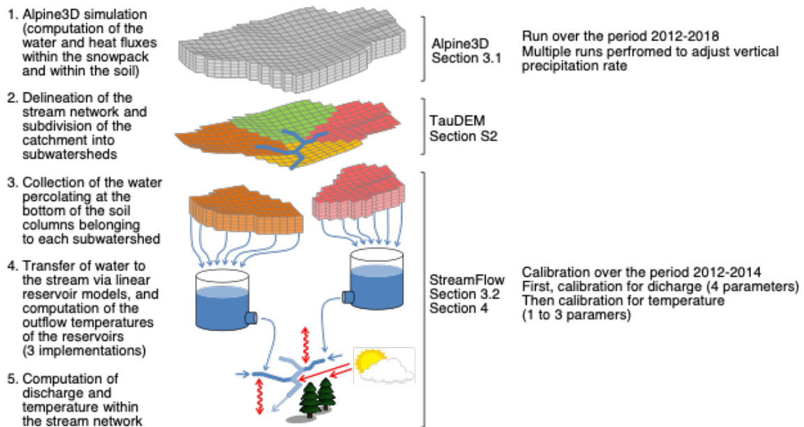
Figure 1 – Details of the models' workflow. The calibration and validation periods indicated hold for all catchments except for the Eulach catchment (where the periods 2015-2016 and 2017-2018 are used). Figure adapted from Gallice et al. (2016)
