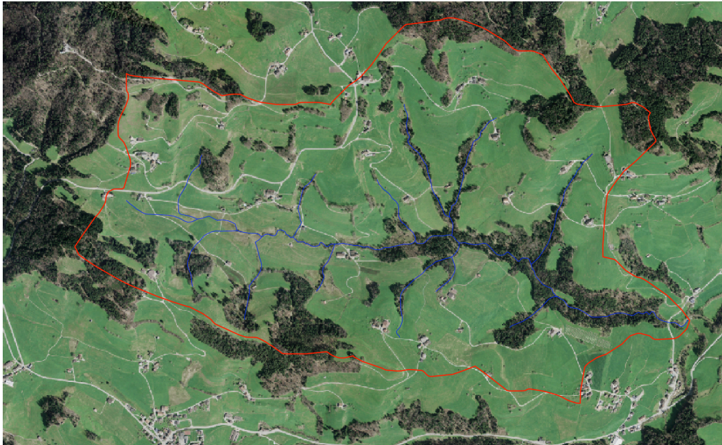
Figure 4 – Rietholzbach catchment (red) and river course (blue). Source: Swisstopo
