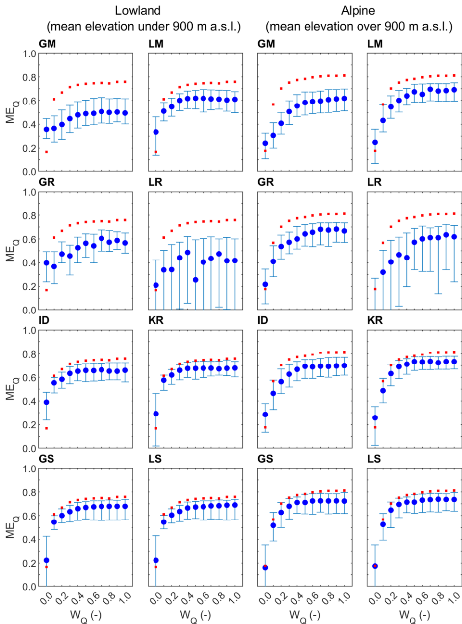
720 Figure 2: Median and regional scatter of leave-one-out runoff model efficiency (Eq. 5) obtained by eight groups of parameter transfer methods and eleven calibration weights for lowland (94) and alpine (119) catchments in the calibration (2000-2010, blue symbols) period. Blue circles represent the median, whiskers the 25- and 75% quantiles of leave-one-out efficiency. Red symbols show the median of at site runoff model efficiency.
