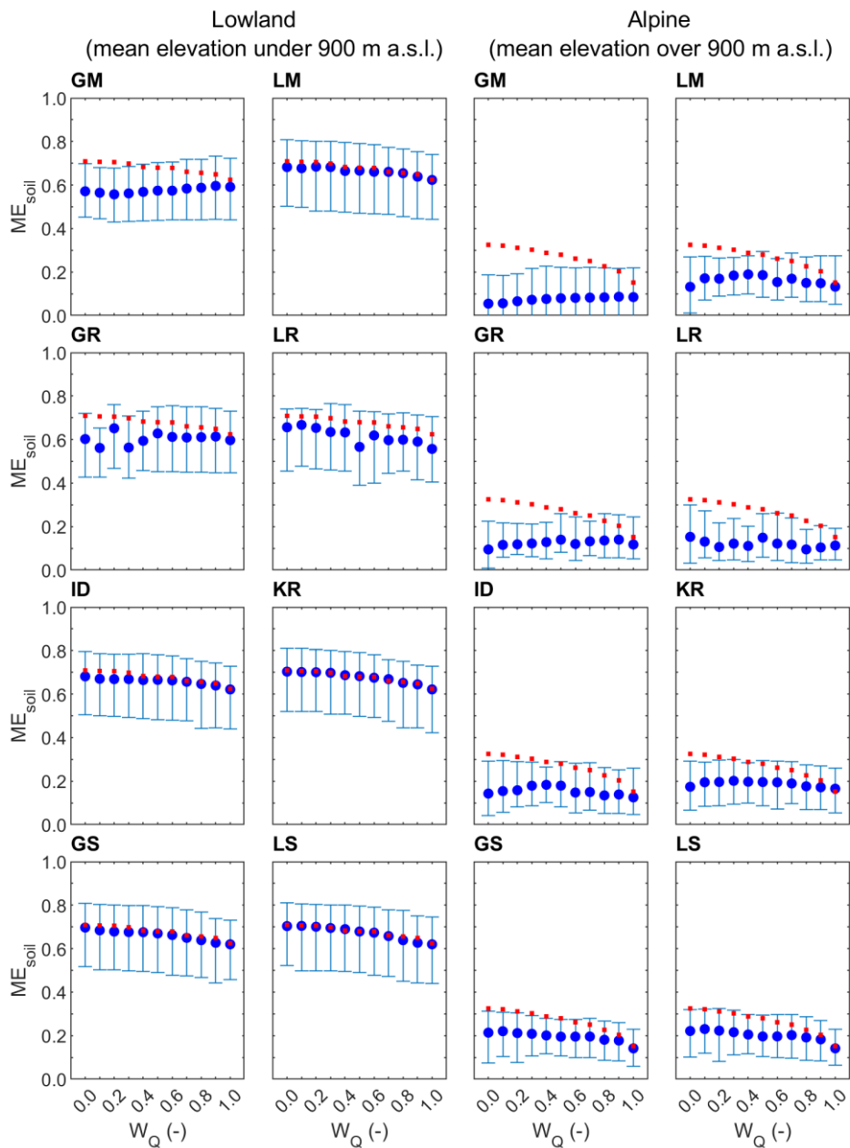
730 Figure 4: Median and regional scatter of leave-one-out soil moisture correlation (Eq. 8) obtained by eight groups of parameter transfer methods and eleven calibration weights for lowland (94) and alpine (119) catchments in the calibration (2007-2010, blue symbols) period. Blue circles represent the median, whiskers the 25- and 75% quantiles of leave-one-out efficiency. Red symbols show the median of at site soil moisture correlations.
