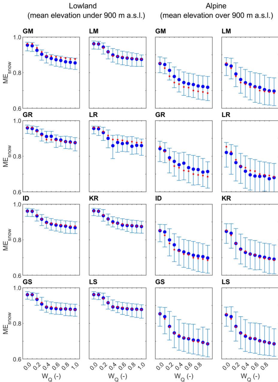
740 Figure 6: Median and regional scatter of leave-one-out snow model efficiency (Eq. 9) obtained by eight groups of parameter transfer methods and eleven calibration weights for lowland (94) and alpine (119) catchments in the calibration (2000-2010, blue symbols) period. Blue circles represent the median, whiskers the 25- and 75% quantiles of leave-one out efficiency. Red symbols show the median of at site snow model efficiency.
