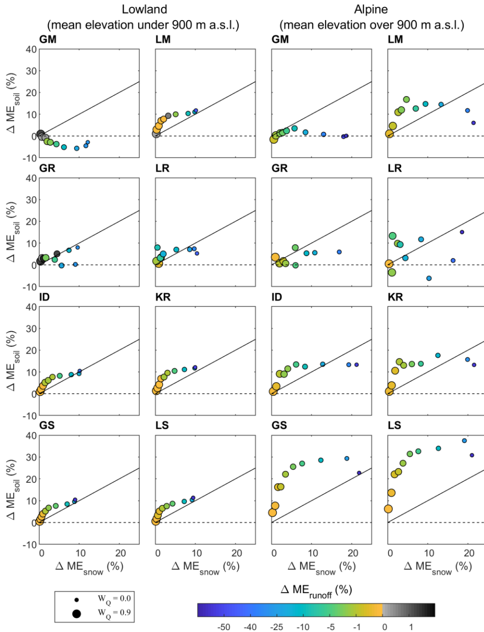
Figure 8: Relative difference (%) in the median of snow cover (horizontal axis), soil moisture (vertical axis) and runoff (colour of symbols) efficiency between model simulations obtained by transferring model parameters calibrated by multiple-objective calibration and calibration to runoff only. The relative difference is estimated for eight model transfer methods (panels) applied in the lowland (left panels) and alpine (right panels) catchments in the calibration period 2000-2010 (soil moisture: 2007-2010).
