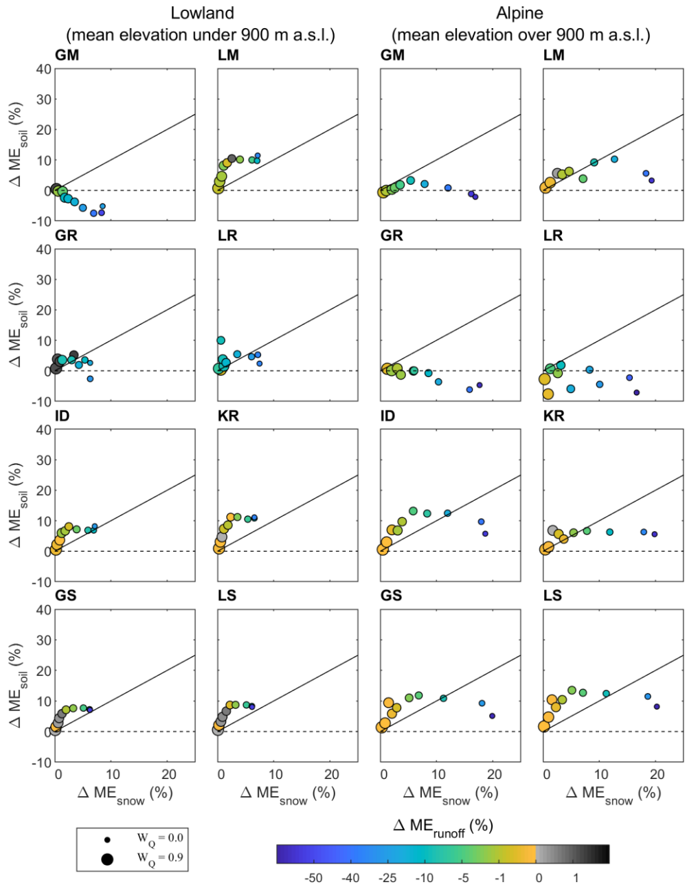
Figure 9: Same as Fig. 8, but for the validation period (2010-2014)
