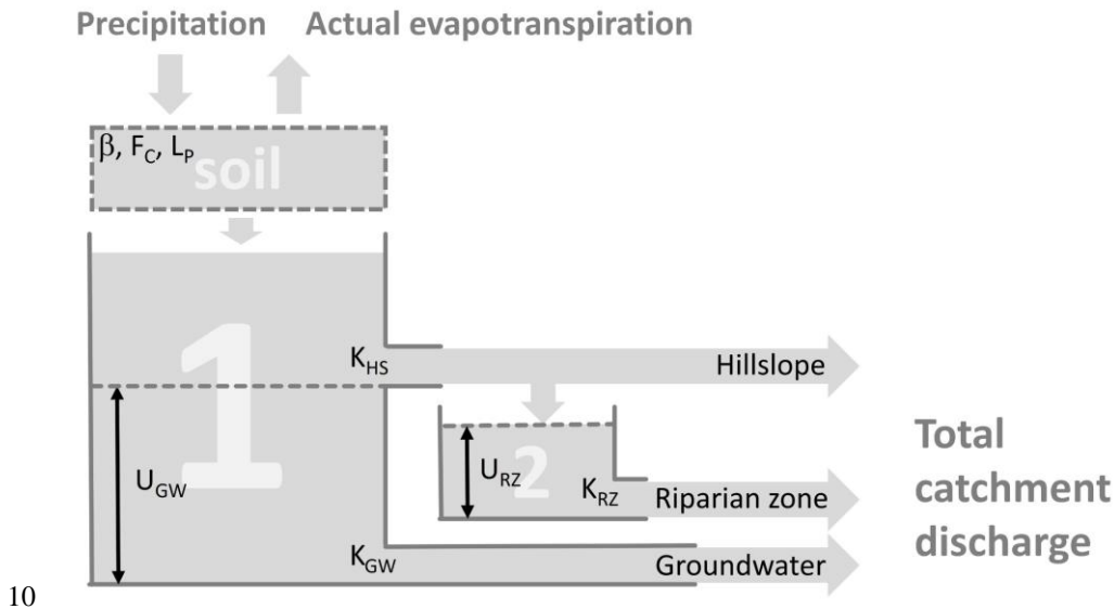
Figure 7: Structure of the modified HBV model. The three components hillslope, riparian zone and groundwater sum up to total catchment discharge.
