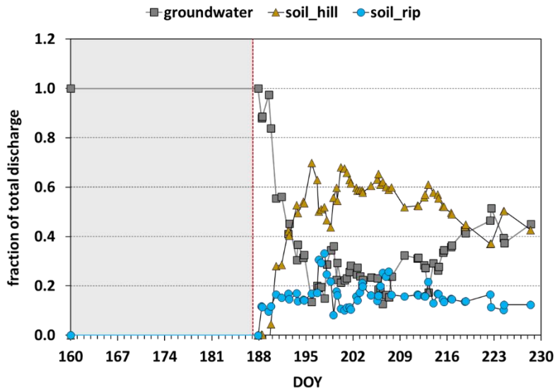
Figure 6: Contributions of the three selected end-members to total discharge for the period DOY 188-230. The red dashed line indicates the onset of the main period of the monsoon. Prior to DOY 188, streamflow was primarily composed of groundwater.
