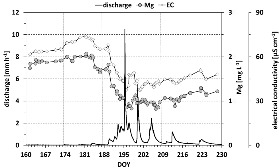
Figure 3: Time series of discharge and of EC and Mg in streamflow. Vertical dashed grey lines separate the four monsoon periods (see also Figure 2).
