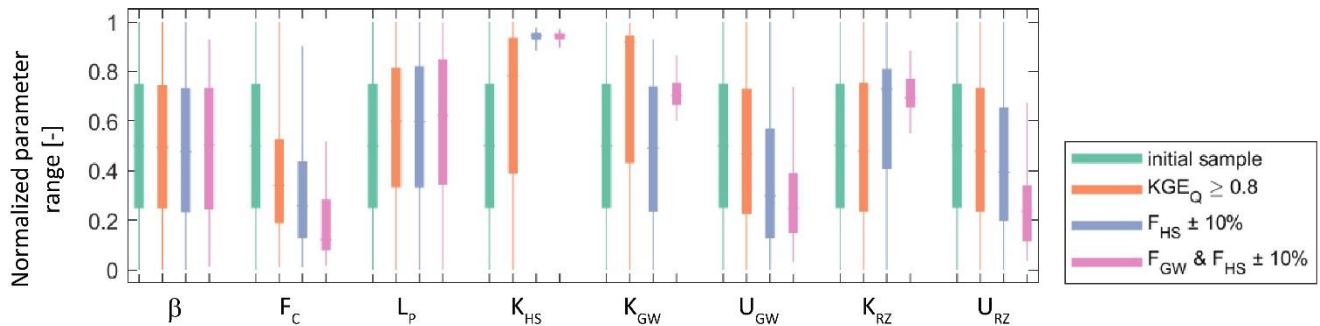
Figure 9: Initial parameter distribution and their modification along the three parameter estimation steps for the individual years 2013 and 2014, as well as for both years together. Boxes indicate the range between the 25 th and 75 th percentile, lower and upper whiskers show the 5 th and 95 th percentile, respectively.
