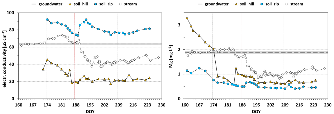
Figure 4: Time series of electrical conductivity (left) and magnesium (right) in streamflow and in the end-members hillslope soil water (soil_hill) and riparian zone soil water (soil_rip). For the groundwater end-member, the mean of baseflow concentrations during the pre-monsoon period (DOY 160-173) is shown, as well as the standard deviation (n=11) as grey band. Vertical dashed grey lines separate the four monsoon periods (see also Figure 2). The red dashed line signifies the onset of the main period of the monsoon.
