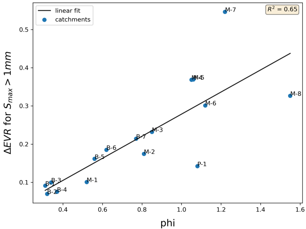
Figure 4: Linear correlation between evaporation ratio (EVR) range and dryness index
