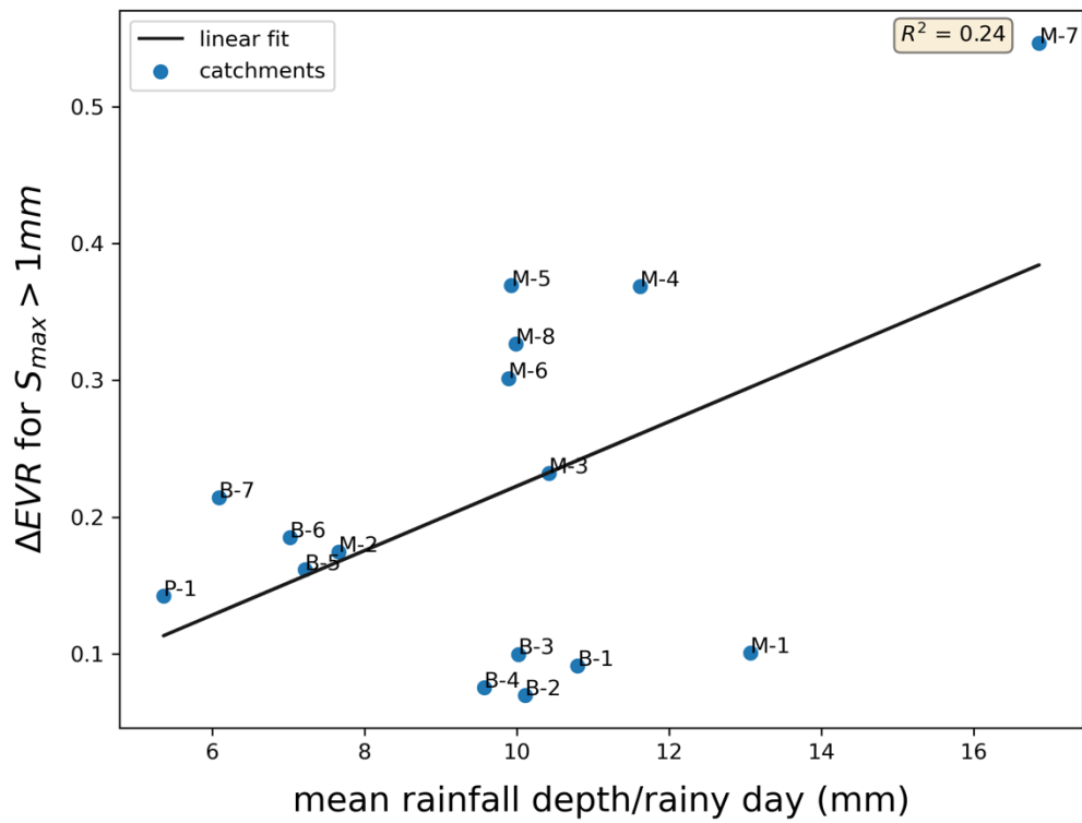
Figure 2: Linear correlation between evaporation ratio (EVR) range and mean daily precipitation
