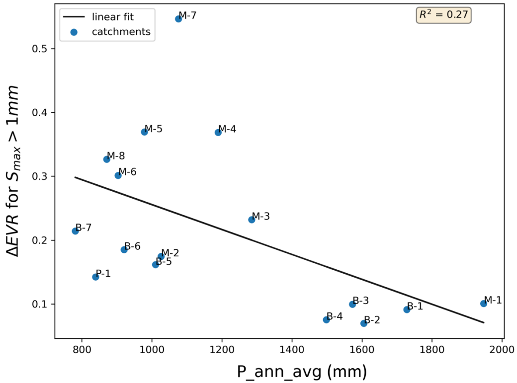
Figure 3: Linear correlation between evaporation ratio (EVR) range and annual average precipitation
