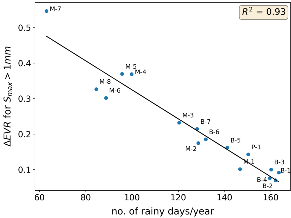
Figure 1: Linear correlation between evaporation ratio (EVR) range and no. of rainy days/year (Figure 9 in the manuscript)
