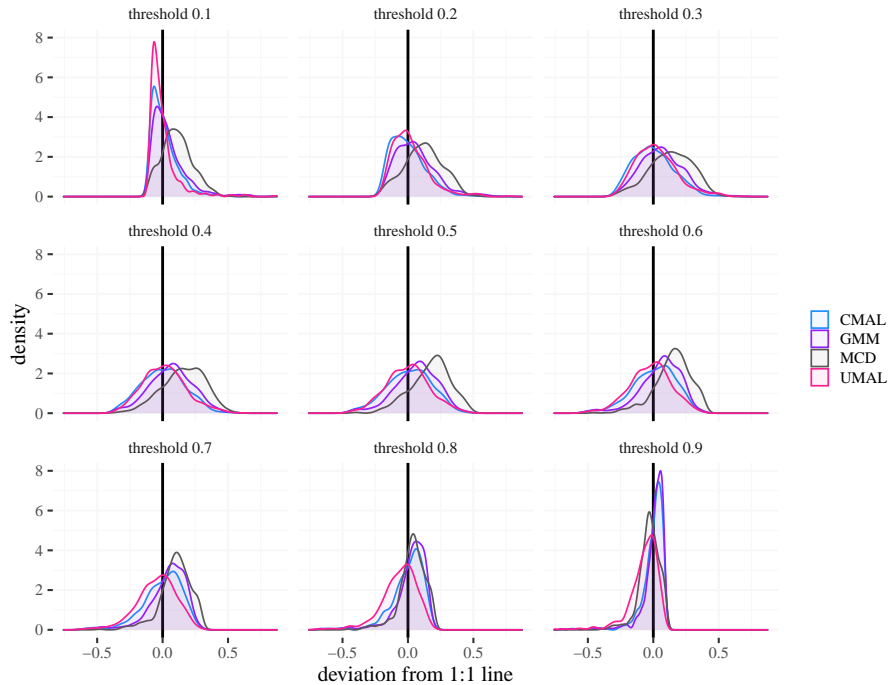
Reliability benchmark: basin-wise deviation evaluation Basin-wise deviations from the 1:1 line for the different probability plot thresholds
