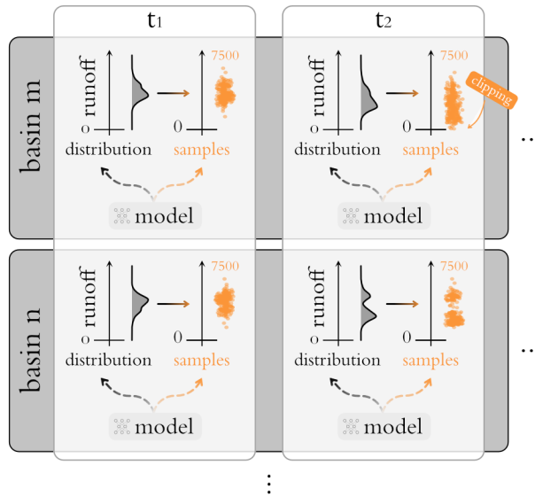
Figure 7. Schemata of the general setup. Vertically the procedure is illustrated for two arbitrary basins, m and n , horizontally the corresponding timesteps are depicted. In total we have 531 basin with approximately 3650 data points in time each. For And, for each time step we compute 7500 samples. In the case of MCD we achieve this by either directly sampling from the model (MCD) or by. In the case of the MDNs we first estimating a conditional distribution first and then sampling sample from it (all MDNs). The "clipping" sign emphasizes our choice to set samples that would be below zero back to the zero-runoff baseline.
