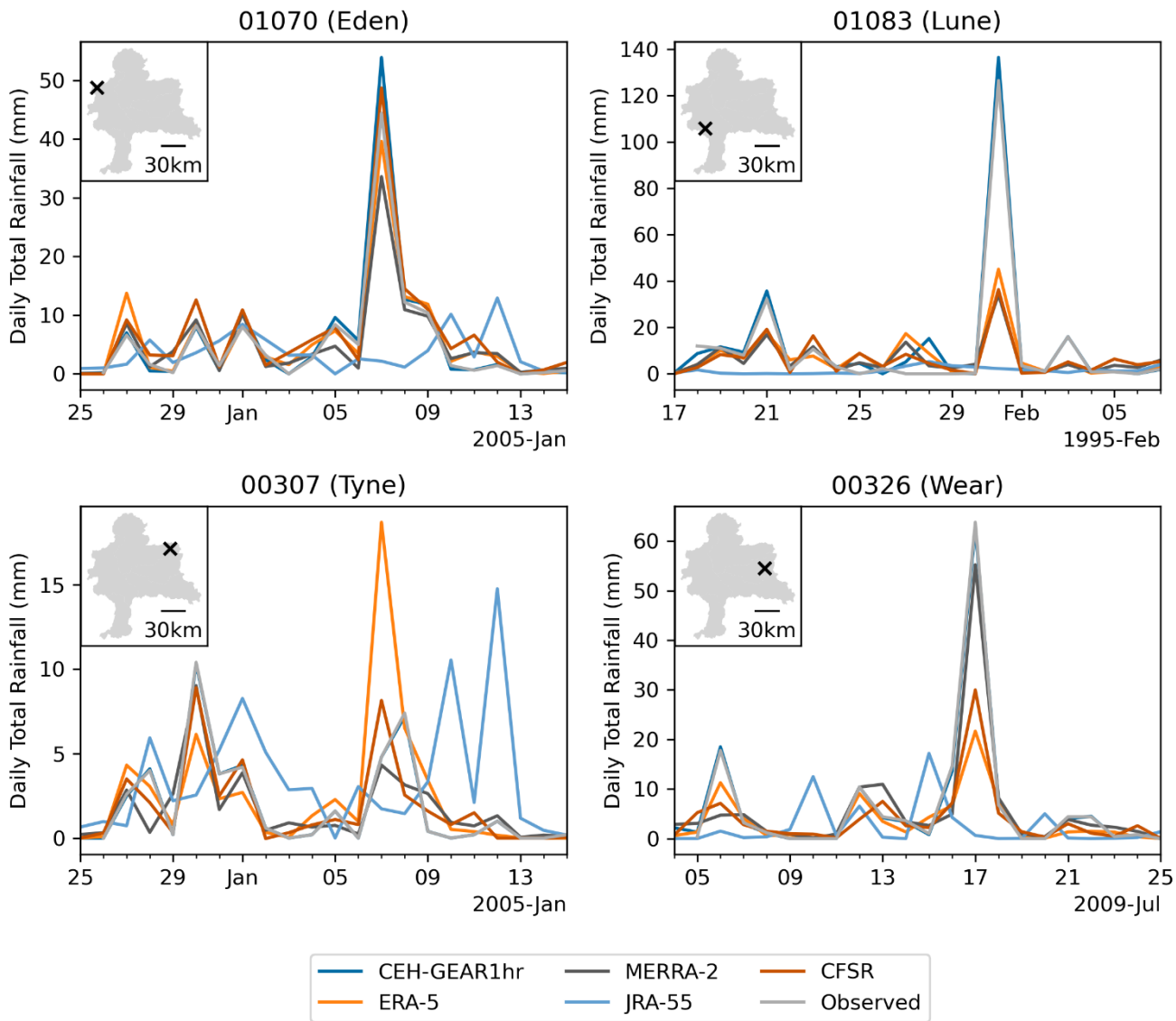
650 Figure 2 – Comparison of daily rainfall totals from each dataset with observed values at selected gauges. The observations were obtained from MIDAS Open (Met Office, 2019). The MIDAS station ID of each gauge is shown in the title of each subplot. The series were converted from hourly to daily to improve clarity. CEH-GEAR1hr becomes obscured in places due to it precisely following the observed series.
