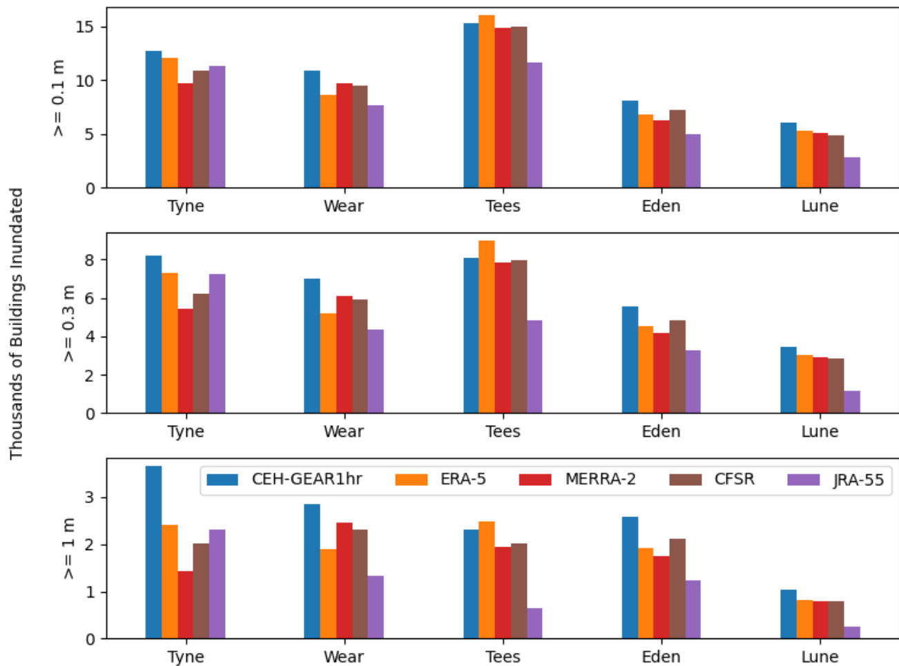
Figure 8 Number of buildings inundated above given thresholds threshold (0.3 m) per basin by each model.
