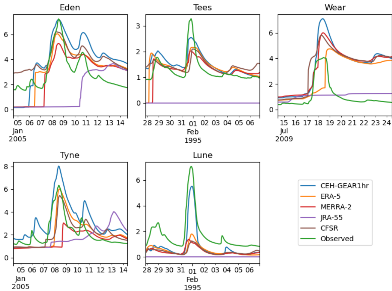
Figure 7 Stage hydrographs comparing water depths (m) from model results and observed values at each gauge.
