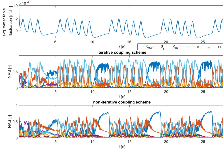
Figure 17. Upper plot: Averaged water table fluctuation of the iteratively coupled model. Lower plots: Transient normalized activity scores for the two coupling methods.
