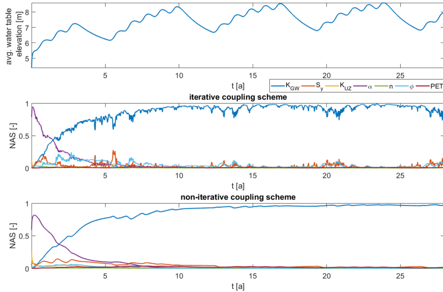
Figure 16. Upper plot: Averaged water table elevation of the iteratively coupled model. Lower plots: Transient normalized activity scores for the two coupling methods.
