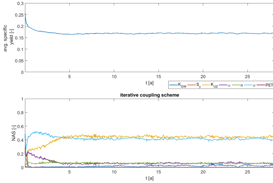
Figure 19. Upper: Averaged specific yield values of the iteratively coupled model. Lower: Transient normalized activity scores for the iterative coupling method.
