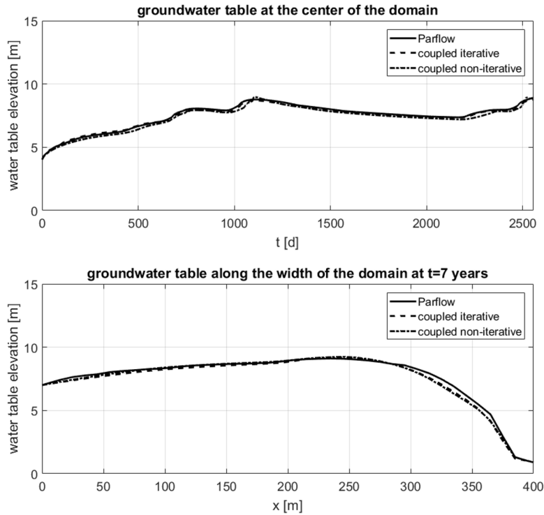
Figure 12. Results of the 3D flow problem. Upper: Groundwater table elevation over time in the center of the domain. Lower: Groundwater table along the width of the domain ( y = 400 m) at the final time step.
