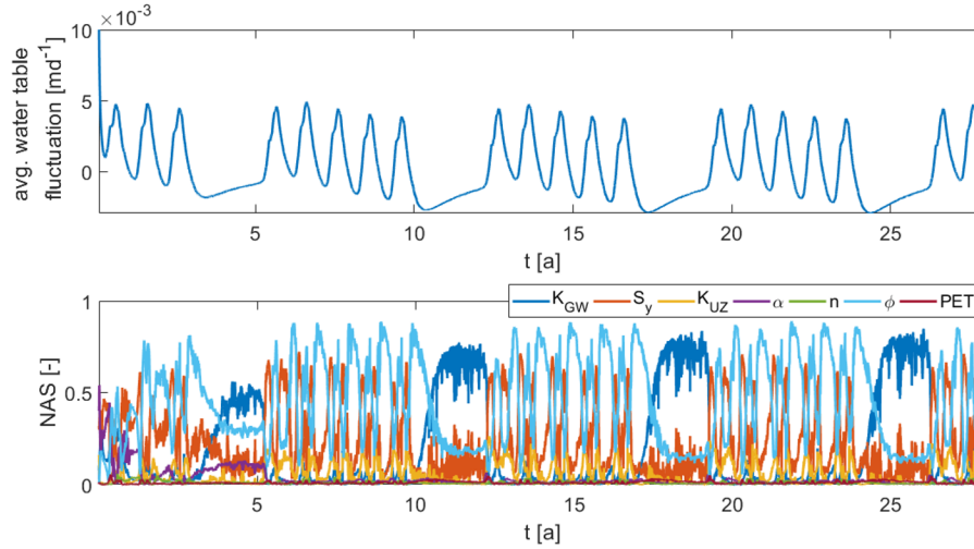
Figure 17. Upper-plot: Averaged water table fluctuation of the iteratively coupled model. Lower-plots: Transient normalized activity scores for the two coupling methods.
