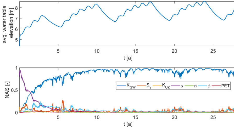
Figure 16. Upper plot: Averaged water table elevation of the iteratively coupled model. Lower plots: Transient normalized activity scores for the two coupling methods.
