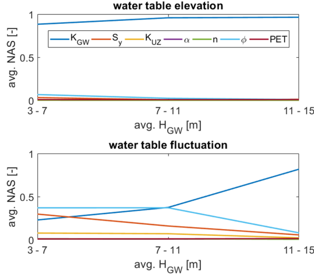
Figure 18. Averaged normalized activity scores of the last seven year cycle for the iteratively-coupled model over the average water table position during that period. Upper: Normalized activity scores for the water table position H_{GW} . Lower: Normalized activity scores for the water table fluctuation \Delta H_{GW} .
