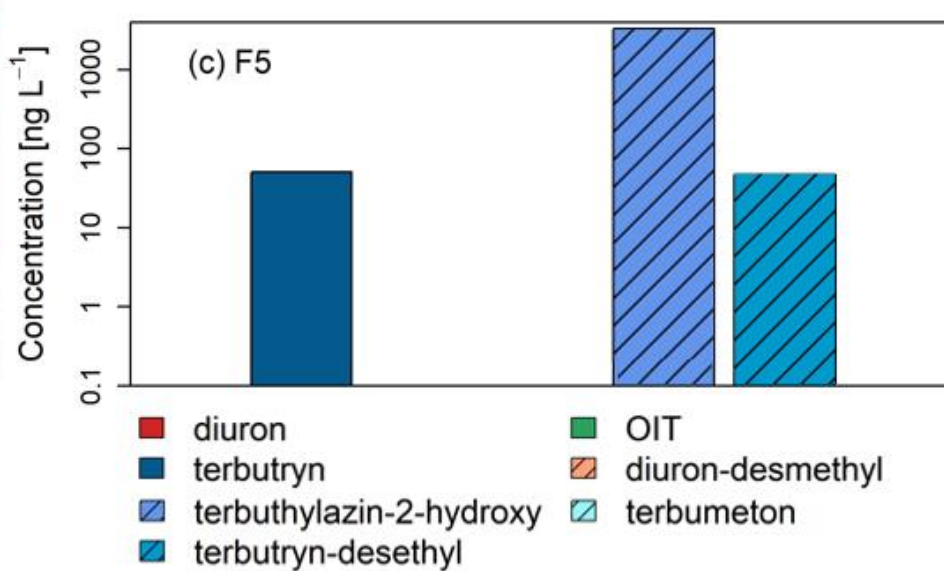
Figure 6: Photos of sampled facade sides and results of facade elution experiments at houses 2, 4 and 5.
