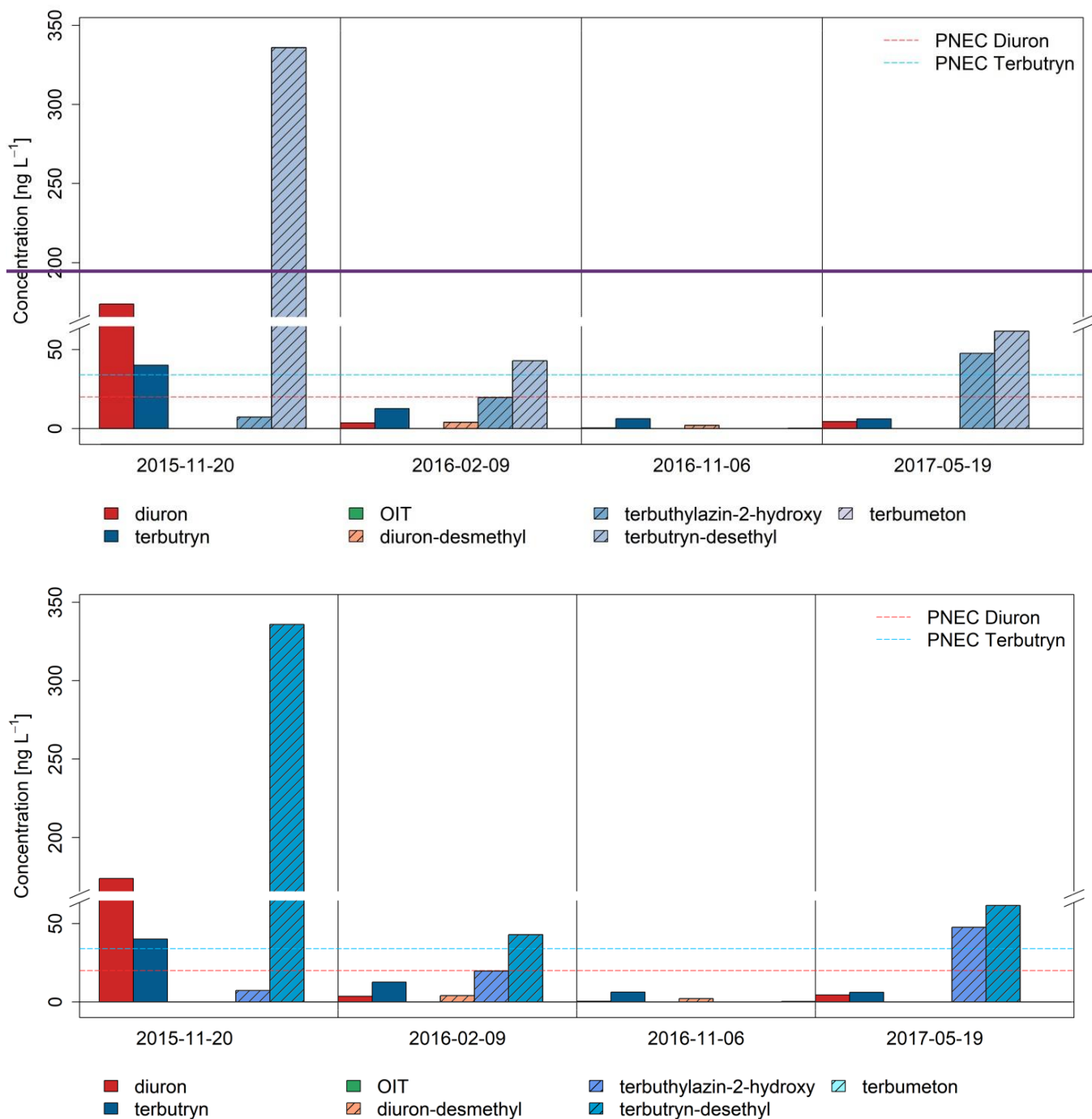
325 Figure 5: Concentrations of monitored biocides of standing water in the swale during four events.
