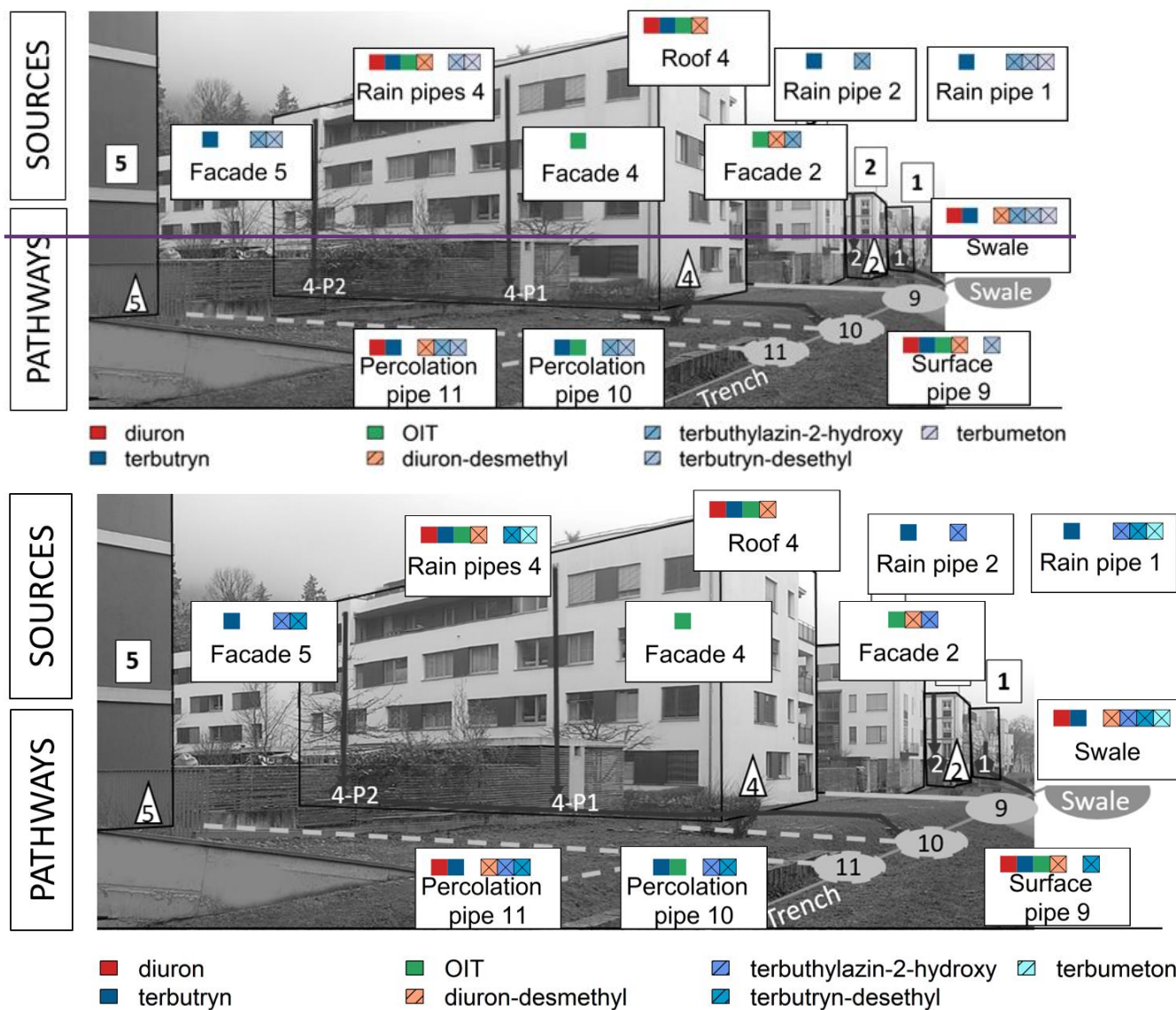
485 Figure 10: Qualitative overview of biocides and their TPs in the investigated water infrastructures. Shown colors at sampling points represent detected substances. For legend of background picture, refer to Fig. 3.
