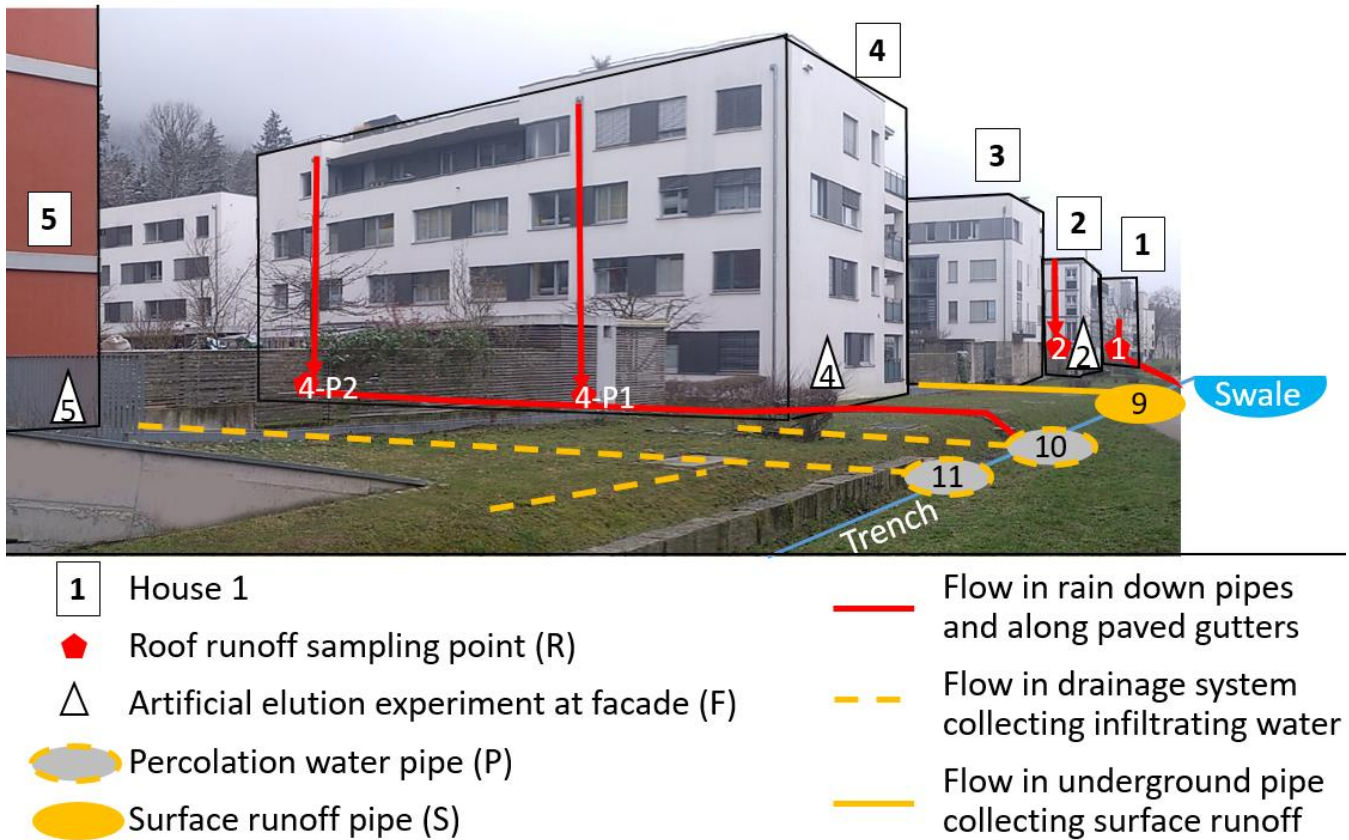
170 Figure 3: Side view of storm water management infrastructure and sampling points.
