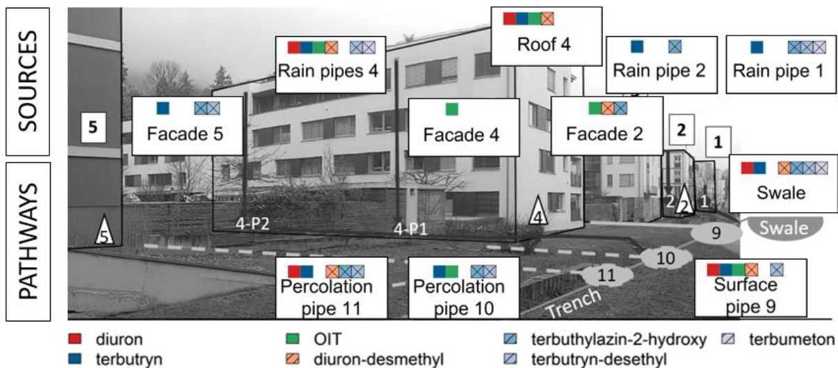
480 Figure 10: Qualitative overview of biocides and their TPs in the investigated water infrastructures. Shown colors at sampling points represent detected substances. For legend of background picture, refer to Fig. 3.
