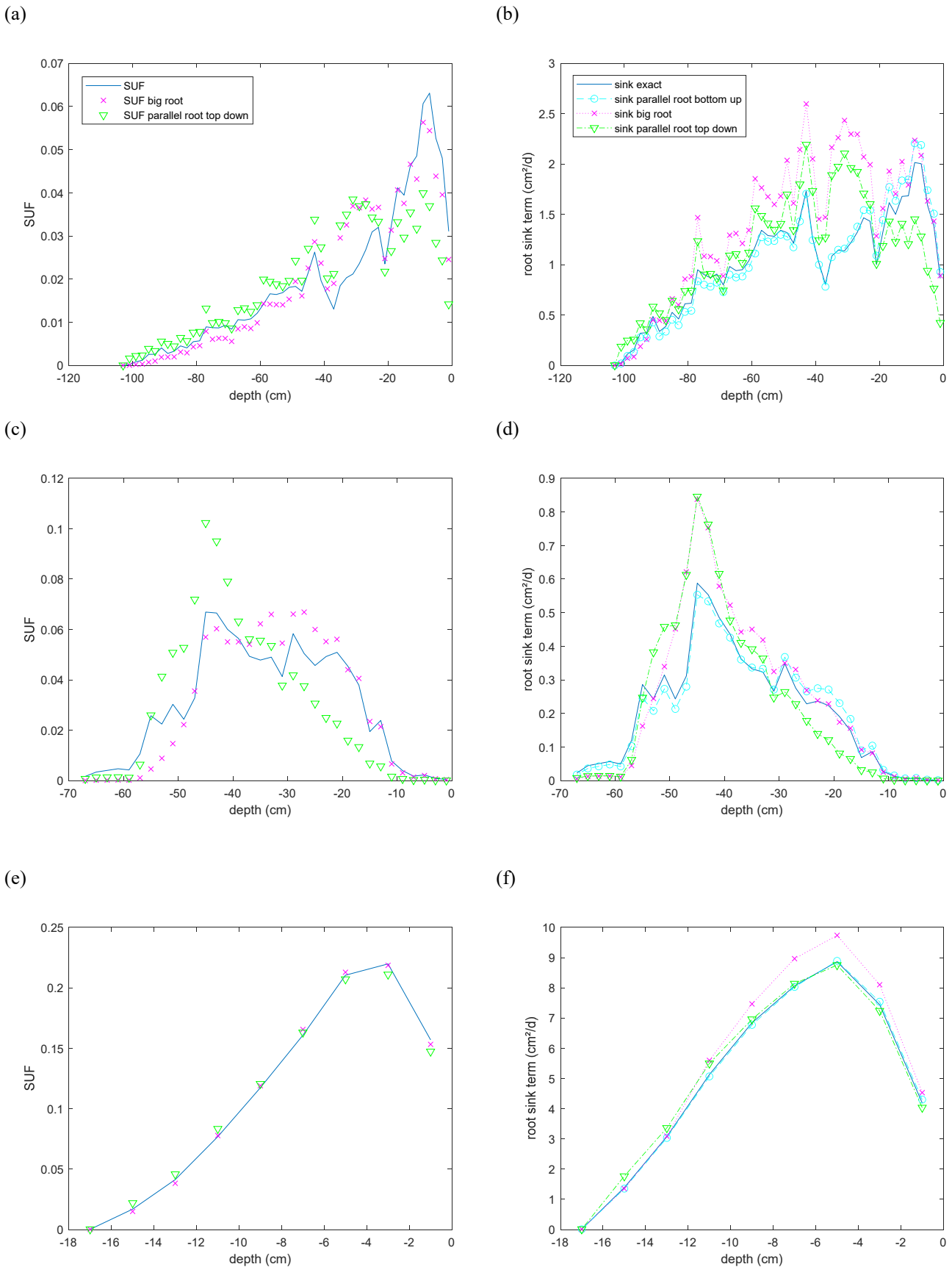
950 Figure 10: Depth profiles of scaled up Standardized Uptake Fractions (SUF) (a,c,e) and sink term distribution normalized by the considered soil layer thickness (2 cm) for a non-uniform soil water potential distribution (-3000 cm at the soil surface and 0 cm at the maximal root depth) (b,d, f) for maize (a,b), sunflower (c,d) and grass (e,f) root systems shown in Fig. 9. Approximations are calculated for the parallel root with a bottom-up parameterization using the exact SUF and K_{rs} , the big root model, and parallel root model with a top-down parameterization with SUF estimated from the radial root segment conductivities. Sink terms are 955 divided by the thickness of the soil layer, 2cm, over which the root segment sink terms are summed.
