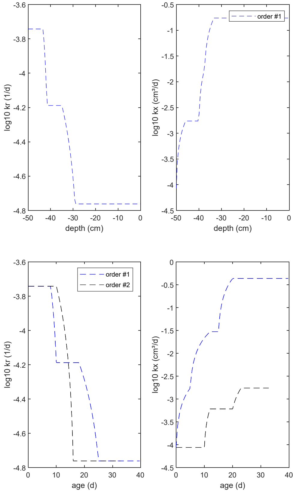
Figure 6: Radial (left), k_r , and axial (right), k_x , intrinsic root conductances for the single root (top) and root system architectures (bottom). For the single root, conductances are plotted versus depth and for the root system architectures versus root segment age.
