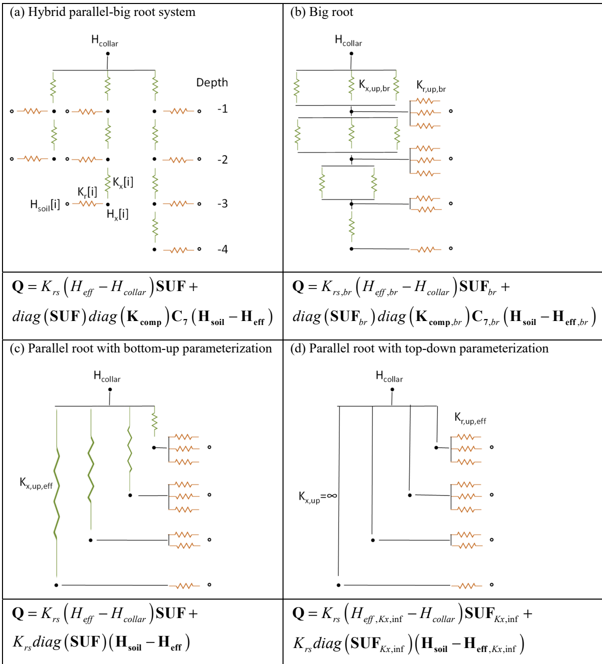
Figure 3: Resistance nets representing the hybrid parallel-big root system consisting of three primary root branches of different length (a); and approximations by: the big root model (b); the parallel root model using a bottom-up parameterization (c); and the parallel root model with a top-down parameterization (d). The closed circles represent root nodes and the open circles soil nodes; the brown and green resistors represent radial and axial root segment conductances, respectively. The approximate models describe upscaled root water uptake from 4 depths. The \text{SUF}_{br} , K_{rs,br} , \mathbf{K}_{comp,br} and C_{7,br} of the big root model are calculated from the segment axial and radial conductances that are arranged following the big root topology in parallel within a soil layer from which upscaled big root segment conductances K_{r,up,br} and K_{x,up,br} are calculated (top-down parameterization). The \text{SUF} and K_{rs} of the parallel root model with bottom-up parameterization (c) are matched to those of the upscaled hybrid model by adapting the axial conductance K_{x,up,eff} of the segment that connects the xylem node at a certain depth to the collar node. The \text{SUF} of the parallel root model with top-down parameterization assuming infinite K_{x,up} (d) is derived from the distribution of radial root segment conductances with depth, which are scaled to K_{r,up,eff} so that K_{rs} matches that of the hybrid root system. The equations below the resistance nets represent the equations that calculate the upscaled water uptake Q in a horizontal layer.
