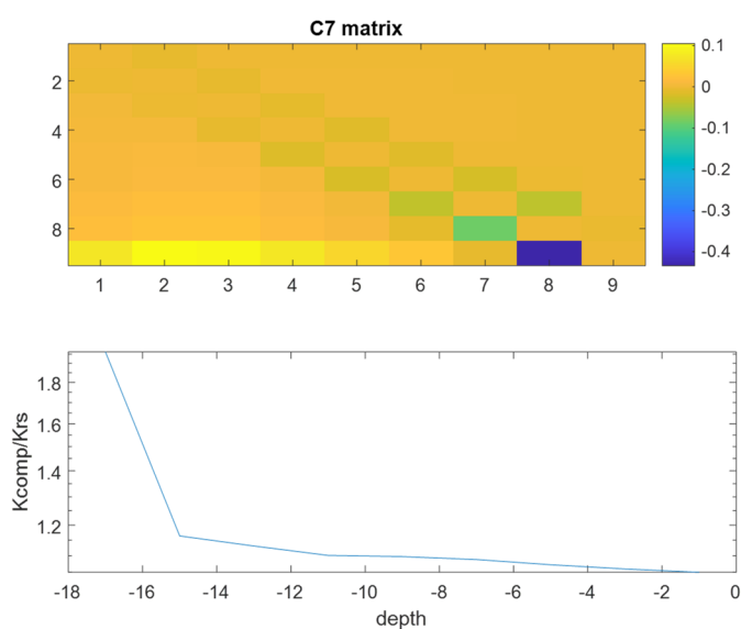
520 Figure 11: C 7 matrices and ratios of Kcomp/Krs of the exact model for the maize a), sunflower b), and grass c) root systems
