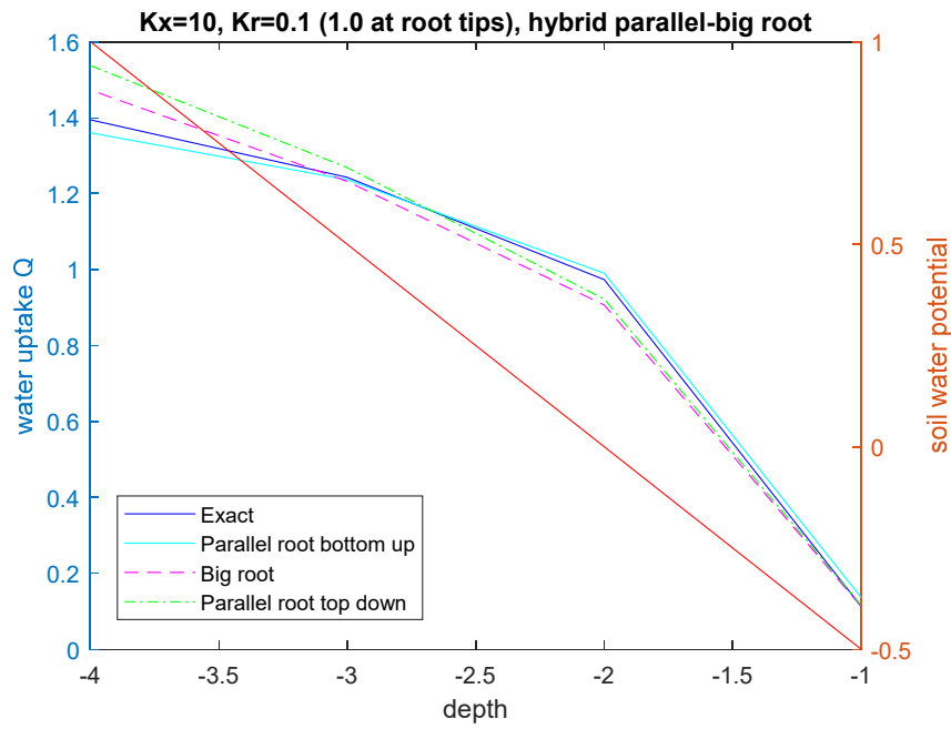
375 Figure 5: Upscaled water uptake profiles (left axis) and soil water potential distribution (right axis, red line) for the hybrid parallel-big root system with radial conductances along the primary root branches that vary along the branches (radial conductance is 1 at root tips and 0.1 at other nodes); the parallel root model with bottom-up parameterization (SUF and K_{rs} derived from exact model); the big root model; and the parallel root model with top-down parameterization.
