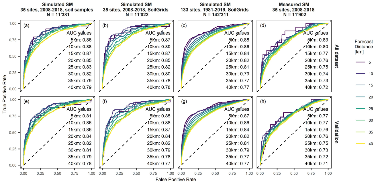
600 Figure 6: ROC plots and AUC values of landslide forecast model fits based on simulated soil moisture (SM) at the 35 monitoring sites including soil hydrological properties from soil samples (a, e) and SoilGrids (b, f), at all 133 sites including soil hydrological properties from SoilGrids (c, g) and based on measured soil moisture at the 35 monitoring sites (d, h). All CoupModel set-ups include a lower boundary condition with groundwater. Upper panels (a-d) show landslide forecast model fits using all the dataset whereas lower panels (e-h) show model fits based on the 5-fold cross-validation scheme.
