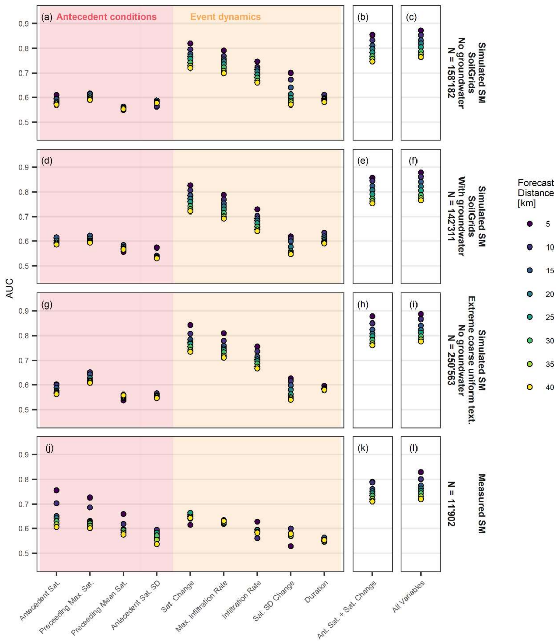
615 Figure 9: AUC values of model fits based on simulated soil moisture (SM) at all 133 sites (upper three rows) and based on measured soil moisture at the 35 monitoring sites (lowest row). Model fits include individual explanatory variables only (a, d, g, j), the explanatory variables antecedent saturation and saturation change only (b, e, h, k) and all nine explanatory variables (c, f, i, l).
