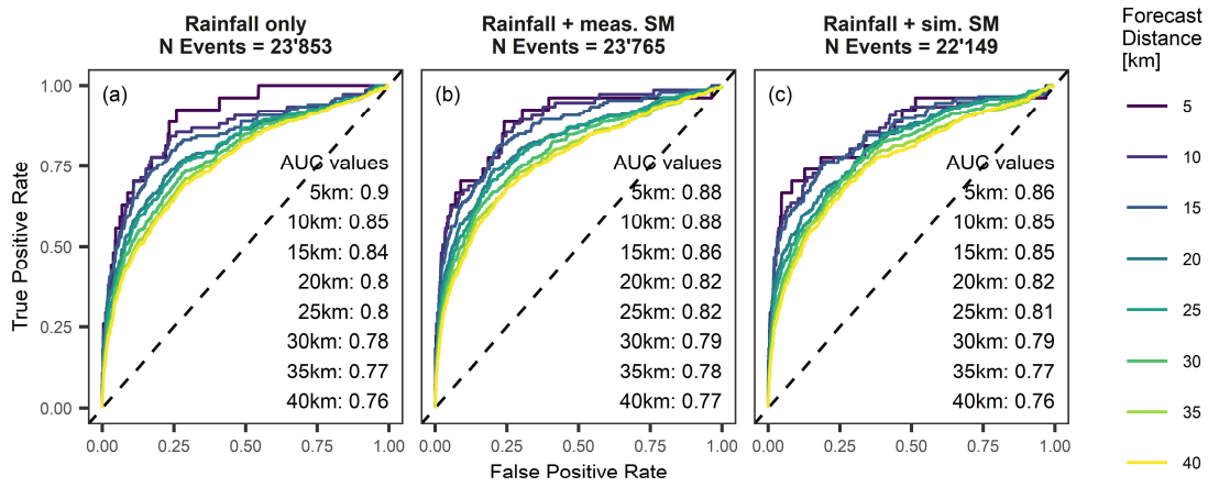
625 Figure 12: ROC curves and AUC values of model fits (a) based on normalized rainfall information only, (b) based on normalized rainfall and measured antecedent saturation, and (c) based on normalized rainfall and simulated antecedent saturation for all 35 monitoring sites and the period of 2008 to 2019.
