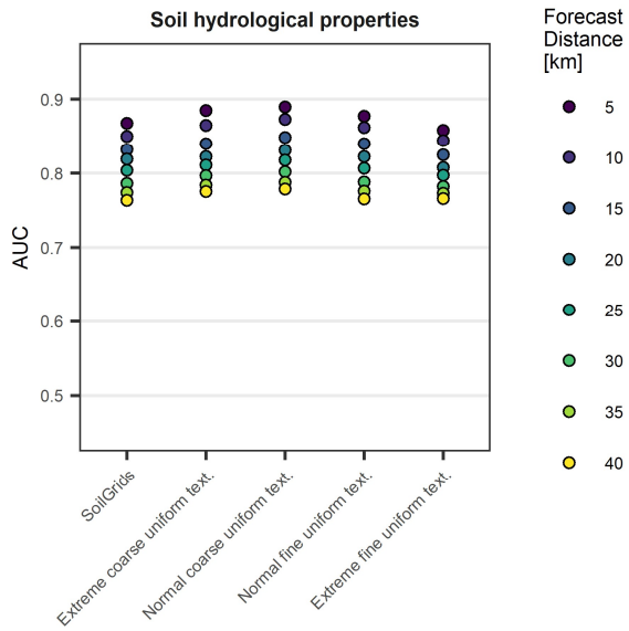
610 Figure 8: AUC values of landslide forecast model fits based on CoupModel set-ups with varying soil hydrological properties (derived from SoilGrids and uniform-texture profiles) and a lower boundary condition with groundwater.
