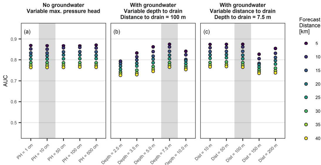
605 Figure 7: AUC values of landslide forecast model fits with different parametrizations of the lower boundary condition by varying (a) the maximum pressure head of the lowest layer above which exfiltration occurs, (b) depth to the drain, and (c) the distance to the drain. Grey shaded model runs correspond to the CoupModel parametrization used in all other analyses.
