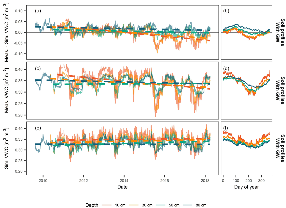
595 Figure 5: Temporal evolution and seasonal variation of mean daily residual VWC (a, b), i.e. deviation between simulated and observed soil water content, and mean daily measured (c, d) and simulated VWC (e, f). Means are calculated across all 14 reference sites by sensor depths (different colours) for a CoupModel set-up using soil hydrological properties derived from SoilGrids and a lower boundary condition with groundwater.
