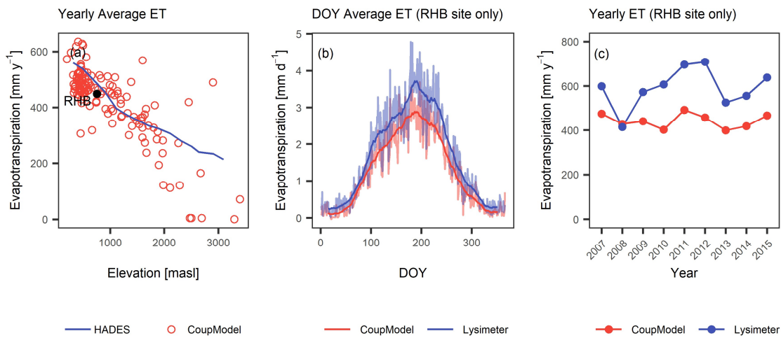
Figure 10: Simulated evapotranspiration (ET) from the CoupModel versus validation data. (a) Yearly average ET versus elevation function from the Swiss Hydrological Atlas, (b) day of the year average ET and (c) yearly ET at the Rietholzbach site (RHB) vs. lysimeter data measured at this site.
