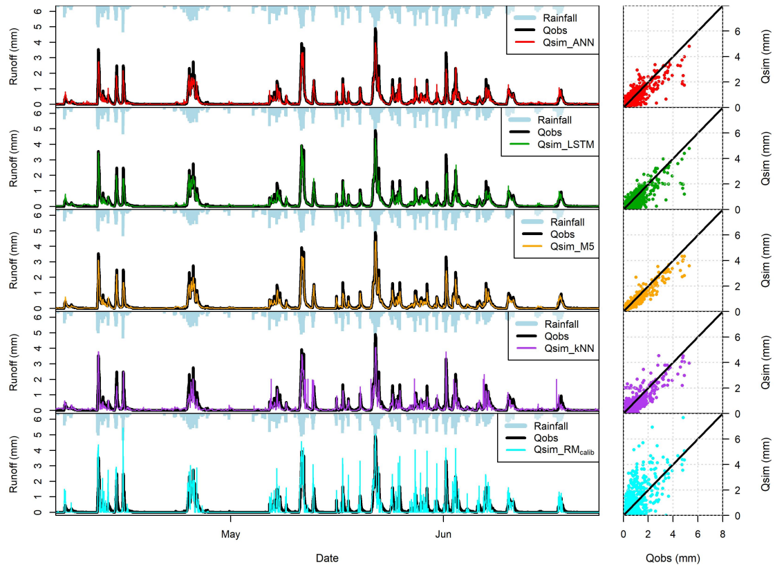
Figure 6. Performance of ML models on the testing period (BERG 2). The hydrographs were plotted for around three months period (2000 hours), while the Q-Q plots were plotted for the entire testing period
