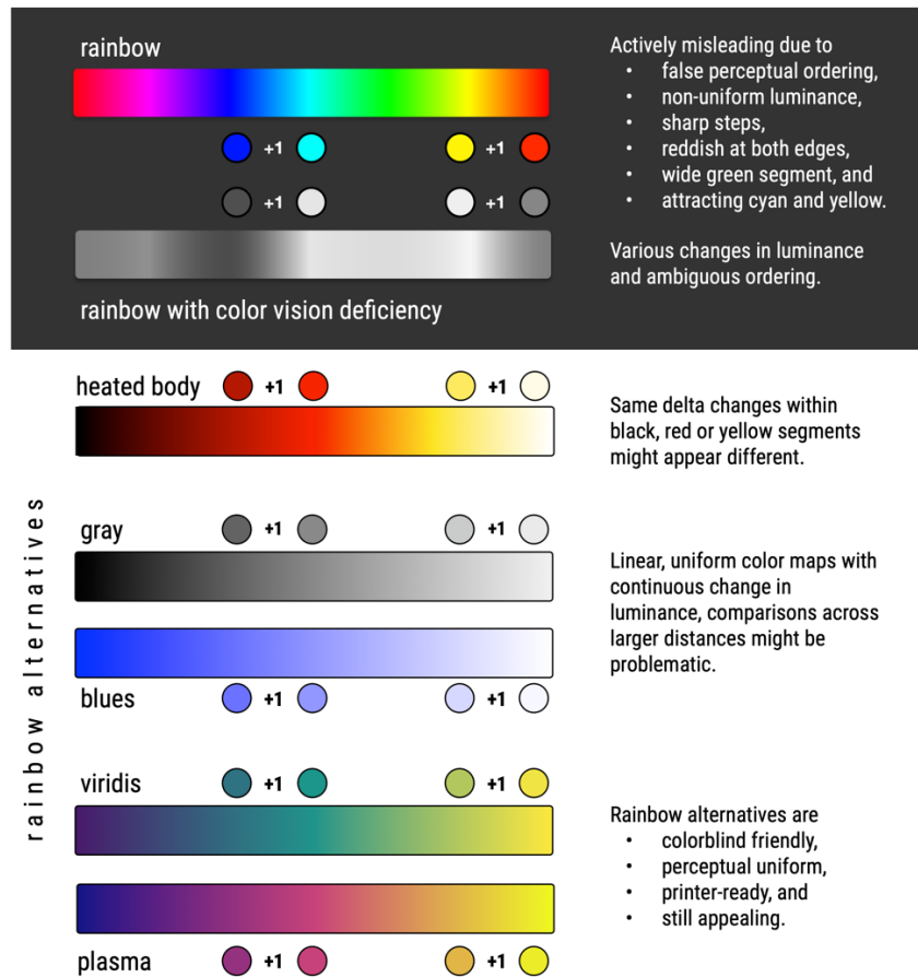
Figure 1: Comparison of different color maps along an arbitrary scale (0-6). The same delta changes in x-values (denoted with +1) are not represented uniformly in the rainbow or heated body color map due to unordered luminance. Alternatives are monochromatic, single-hue color maps (greys, blues) or perceptually uniform designed multi-hue color maps like viridis or plasma. Diverging color maps highlight data extremes and the data direction (e.g., positive/negative data values) if a meaningful midpoint is apparent in the data. Visualization inspired by literature (Crameri et al., 2020; Wong, 2011b).
