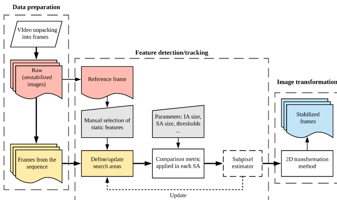
Figure 1: General outline of the manual feature selection/tracking approach. SA = Search Area, IA = Interrogation Area
