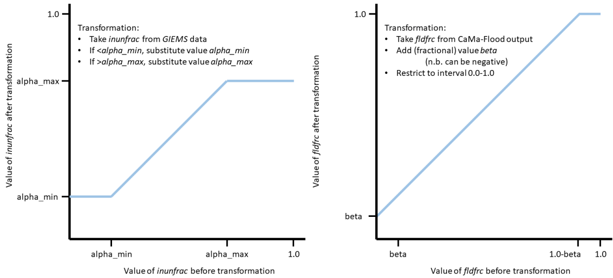
470 Figure 2: Transforming the GIEMS inundated fraction ( inunfrac ) data (left) and CaMa-Flood output flooded fraction ( fldfrc ) variable (right). Note that values \alpha_{min} = \beta = 0.0 and \alpha_{max} = 1.0 are equivalent to making no modification.
