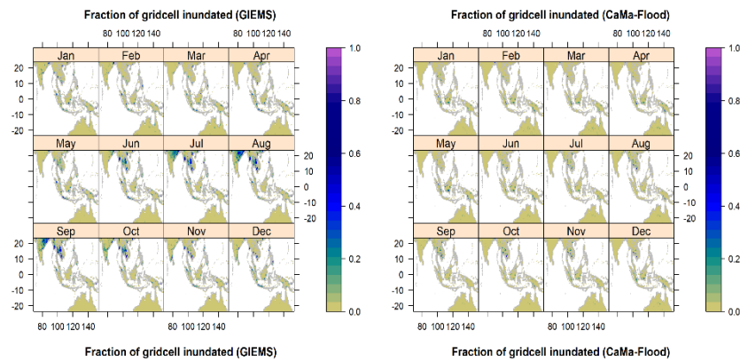
475 Figure 3: Fraction of gridcell inundated (in addition to water contained in channels and watercourses, which are not shown) in each study area. Superposed lakes and reservoirs are from the Global Lakes and Wetlands Database GLWD (Lehner and Döll, 2004). Resolution is 0.25^\circ in both latitude and longitude (n.b. the Tonlé Sap is our smallest wetland, therefore the gridcells are relatively large in that plot). View window extent is taken from references in Table 1. Cities with populations >100\,000 480 are shown (SimpleMaps, 2019) for view extents up to 2\,000\,000\text{ km}^2 . Data shown are an average for 1992-2014 from GIEMS-2 observations (left) and equivalent JULES-CaMa-Flood simulations (right).
