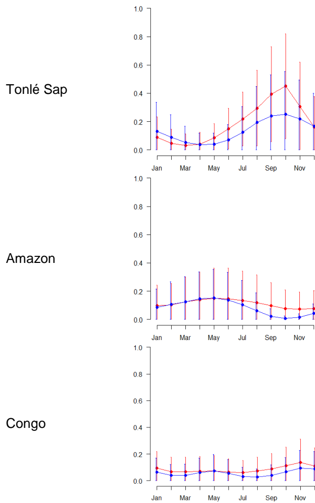
485 Figure 4: Seasonal variation in inundation across the study wetlands, averaged across the years 1992-2014: Red = Observations ( GIEMS ), Blue= Simulated ( JULES-CaMa-Flood ). The three main tropical zones are not shown because they include areas both north and south of the Equator.
