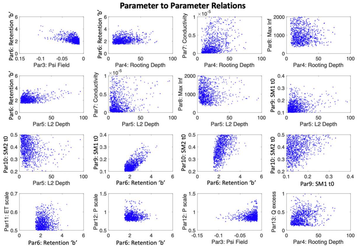
Figure S2: Scatter plots showing correlation of the posterior parameter values with other parameter posteriors. These plots portray the relationship and correlation between pairs of model parameters in the posterior space as inferred by GRACE.
