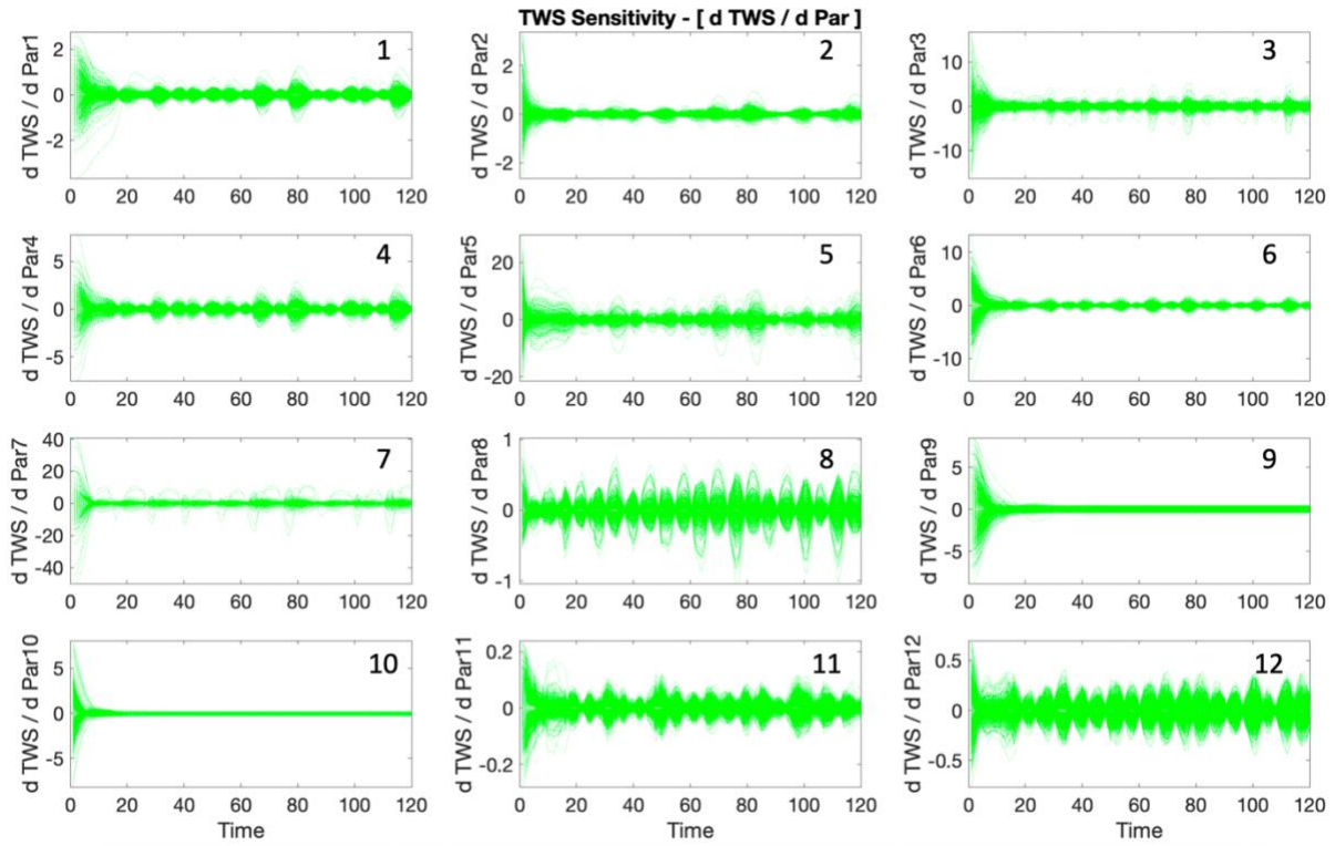
Figure S3: Sensitivity of the model simulated TWS to minor perturbations in parameter values. Shown here in green are the changes in simulated TWS (d TWS) when each parameter is perturbed (d Par) by 1% of its prior range, indicating the magnitude and the time steps of model sensitivity.
