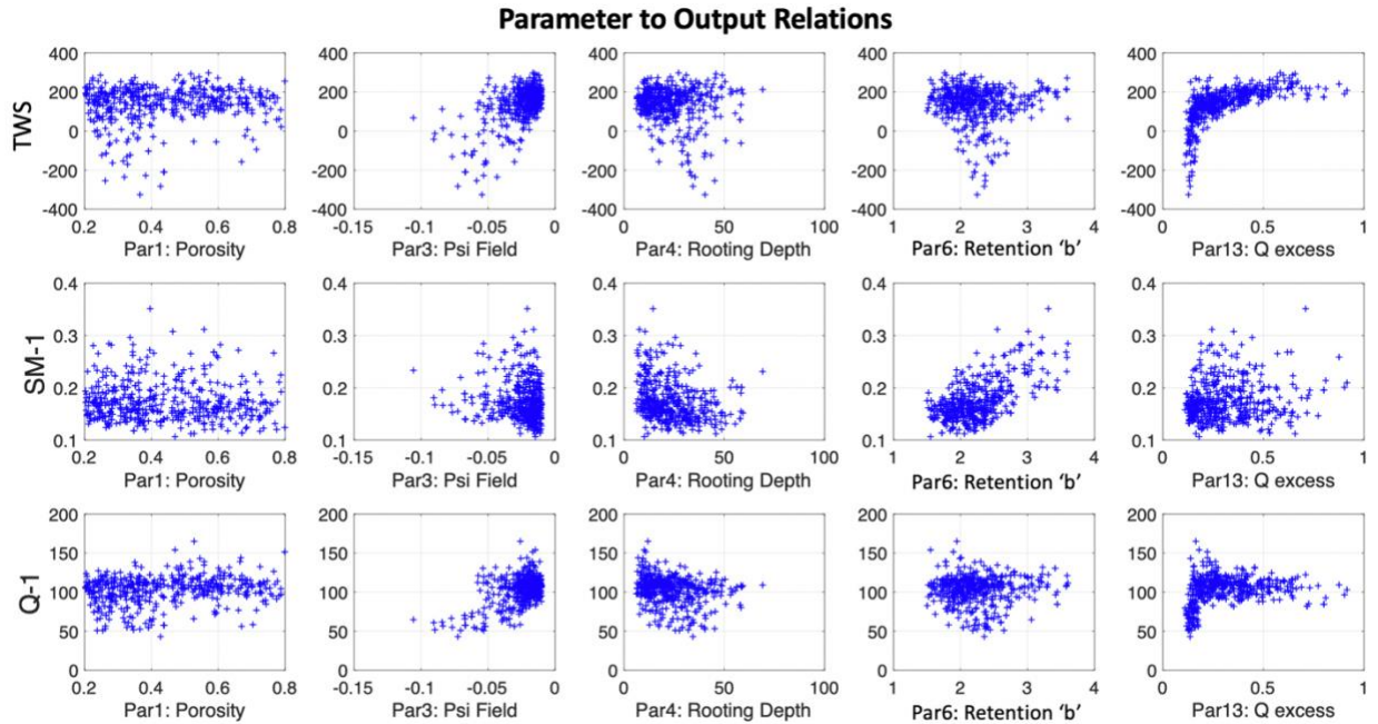
Figure S1: Scatter plots showing correlation of the posterior parameter values with corresponding model simulated values for Terrestrial Water Storage (TWS), soil moisture (SM-1), and discharge (Q-1). These plots portray the relationship and correlation between select estimated parameters and simulated model processes of interest as inferred by GRACE.
