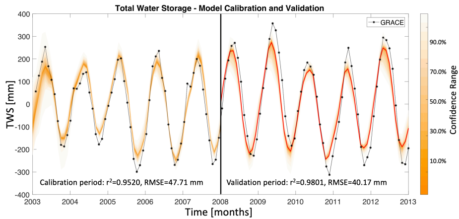
740 Figure 6: Model calibration and validation for monthly TWS anomaly estimates in the Gavião watershed, for the period January 2003 through December 2012. The plot shows the first 5 years of the data for calibration and the remaining 5 years for validation. GRACE-informed posterior ranges of the model simulated TWS are shown here in the orange envelopes for the calibration and validation years, and the red line is used to represent the mean estimates for the validation period.
