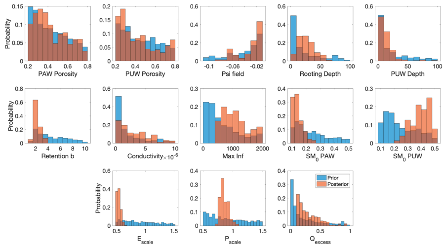
715 Figure 3: Histograms of the prior (blue) and posterior (orange) distributions of the GRACE-informed parameters for the Gavião watershed.
