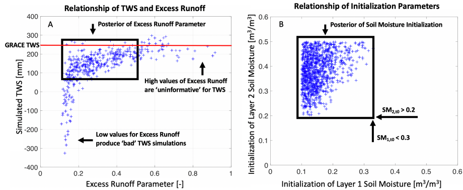
755 Figure 8: A) Posterior relationship of the model simulated TWS [mm] during April 2003 and the runoff excess parameter [uniltess]. The region inside the black box indicates the posterior region with high density, i.e., plausible solutions with high likelihood. The red line shows the ‘true’ TWS value seen in the GRACE data for this period. B) Posterior relationship of the 760 initialization parameters for soil moisture in layers 1 and 2, respectively. Initial SM in layer 2 is larger than 0.2 [m 3 /m 3 ], initial SM in layer 1 is less than 0.3 [m 3 /m 3 ], and SM 2,10 is generally larger than SM 1,10 , as indicated in this plot. See Table 1 and Section 3.4 for details.
