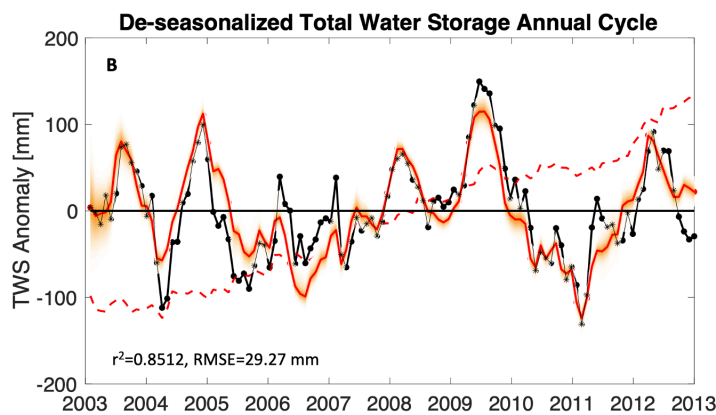
745 Figure 7: A) Annual cycle of the monthly TWS anomalies [mm], from satellite data (GRACE), the prior simulation from the model (Prior), and the data-constrained version of the model simulations (Posterior) for the Gavião watershed. GRACE-informed posterior ranges of the model simulated TWS annual cycle are shown here in the orange envelopes. B) To obtain the de-seasonalized values of TWS for the Gavião watershed shown in Panel B, we subtract the annual cycle in Panel A from each month's estimate shown in Figure 4. This shows whether the anomaly values in each time step of Panel B portrays an extremely dry or wet period relative to what is expected in the annual cycle. Hence, the data-constrained model can capture the 2005-2006 and 2010-2011 droughts that are shown in the GRACE data.
