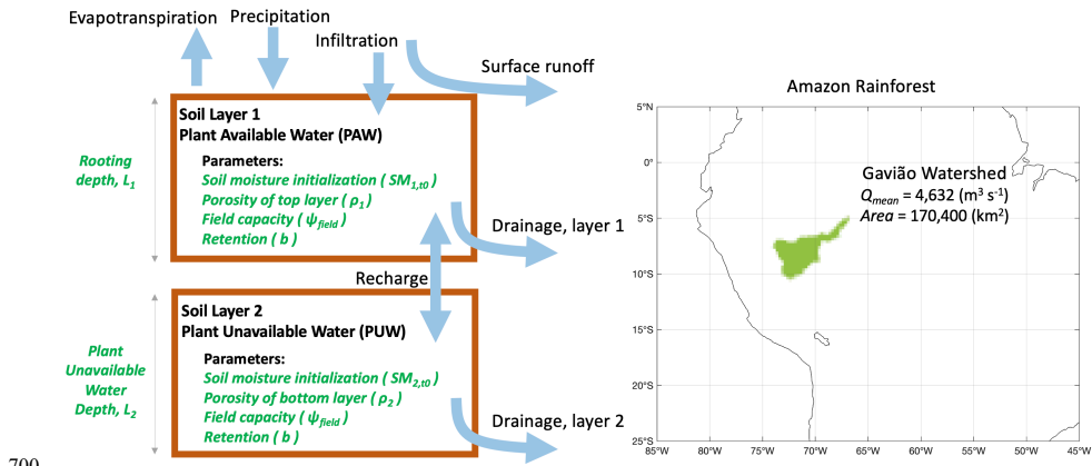
Figure 1: Model schematic for the data-constrained terrestrial water storage model. Arrows indicate the logical flow that describes the movement and storage of water in the model. The domain on the right highlights the western Amazonian watershed investigated in this study, the Gavião Watershed.
