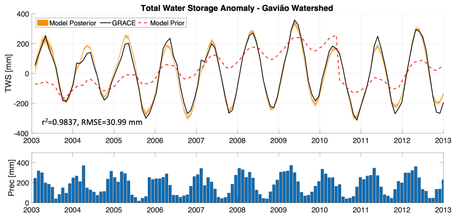
720 Figure 4: Monthly Total Water Storage (TWS) anomaly estimates from satellite data (GRACE TWS), the prior simulation from the model , and the data-constrained version of the model simulations for the Gavião watershed. GRACE-informed posterior ranges of the model simulated TWS are shown here in the orange envelopes. Precipitation values used to drive the model are shown to indicate the seasonal cycle.
