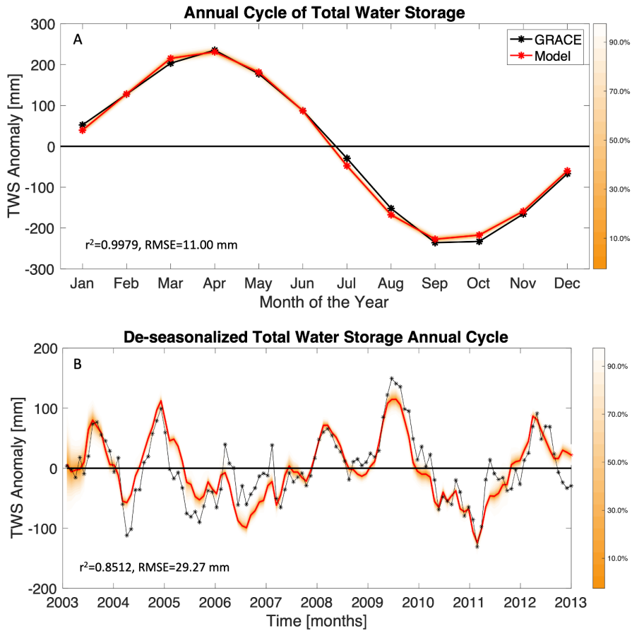
Figure 7: A) Annual cycle of the monthly TWS anomalies [mm], from satellite data (GRACE) and the data-constrained model for the Gavião watershed. GRACE-informed posterior ranges of the model simulated TWS annual cycle are shown here in the orange envelopes. B) To obtain the de-seasonalized values of TWS for the Gavião watershed shown in Panel B, we subtract the annual cycle in Panel A from each month's estimate shown in Figure 4. This shows whether the anomaly values in each time step of Panel B portrays an extremely dry or wet period relative to what is expected in the annual cycle. Hence, the model can capture the 2005-2006 and 2010-2011 droughts that are shown in the GRACE data.
