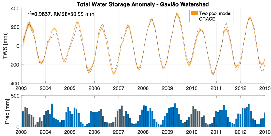
Figure 4: Monthly Total Water Storage (TWS) anomaly estimates from satellite data (GRACE TWS) and the data-constrained model for the Gavião watershed. GRACE-informed posterior ranges of the model simulated TWS are shown here in the orange envelopes. Precipitation values used to drive the model are shown to indicate the seasonal cycle.
